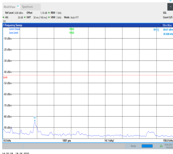
1-N2--15-20-H-1-DFT-PI2BPSK-Inner_1RB_Left-1@ 1-0.009-0.15-Ant1--84.61--43-PASS
