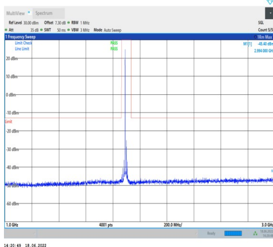
1-N2--15-20-H-1-DFT-PI2BPSK-Inner_1RB_Left-1@ 1-1000-3000-Ant1--45.40--13-PASS
