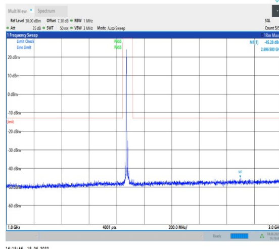
1-N2--15-20-M-1-DFT-PI2BPSK-Inner_1RB_Left-1@ 1-1000-3000-Ant1--45.28--13-PASS
