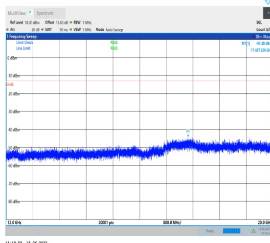
1-N2--15-20-M-1-DFT-PI2BPSK-Inner_1RB_Left-1@ 1-12000-20000-Ant1--44.38--13-PASS
