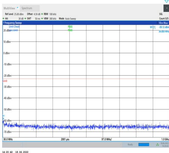
1-N2--15-20-H-1-DFT-PI2BPSK-Inner_1RB_Left-1@ 1-30-1000-Ant1--59.12--23-PASS
