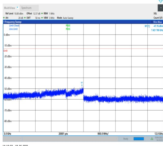
1-N2--15-20-M-1-DFT-PI2BPSK-Inner_1RB_Left-1 @1-3000-12000-Ant1--47.76--13-PASS
