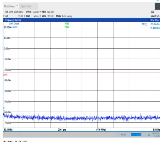
1-N2--15-20-M-1-DFT-PI2BPSK-Inner_1RB_Left-1 @1-30-1000-Ant1--59.85--23-PASS
