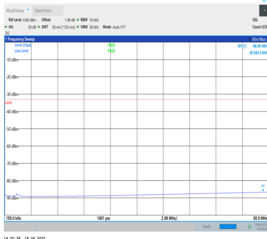
1-N2--15-20-H-1-DFT-PI2BPSK-Inner_1RB_Left-1@ 1-0.15-30-Ant1--86.49--33-PASS
