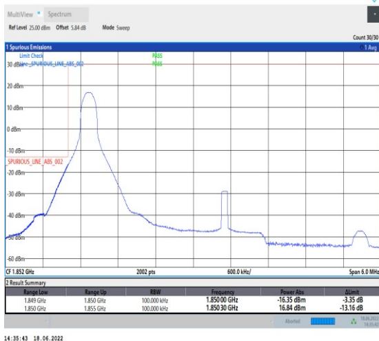
1-N2--15-5-L-4-CP-QPSK-Edge_1RB_Left-1@0-Ant1-s eegraph-PASS-see graph
