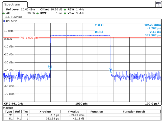
DH1_Hopping 0.382ms
