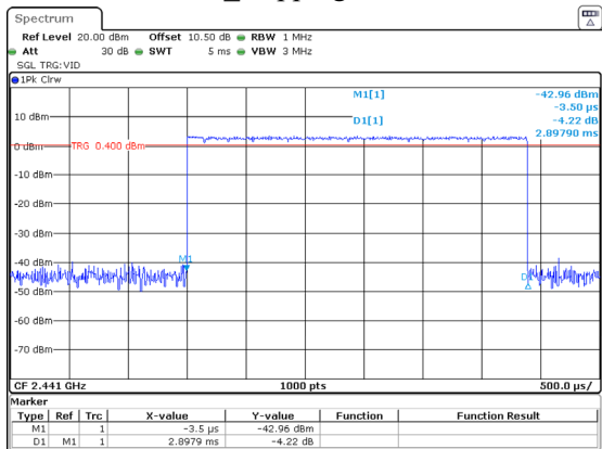
2DH5_Hopping 2.898ms
