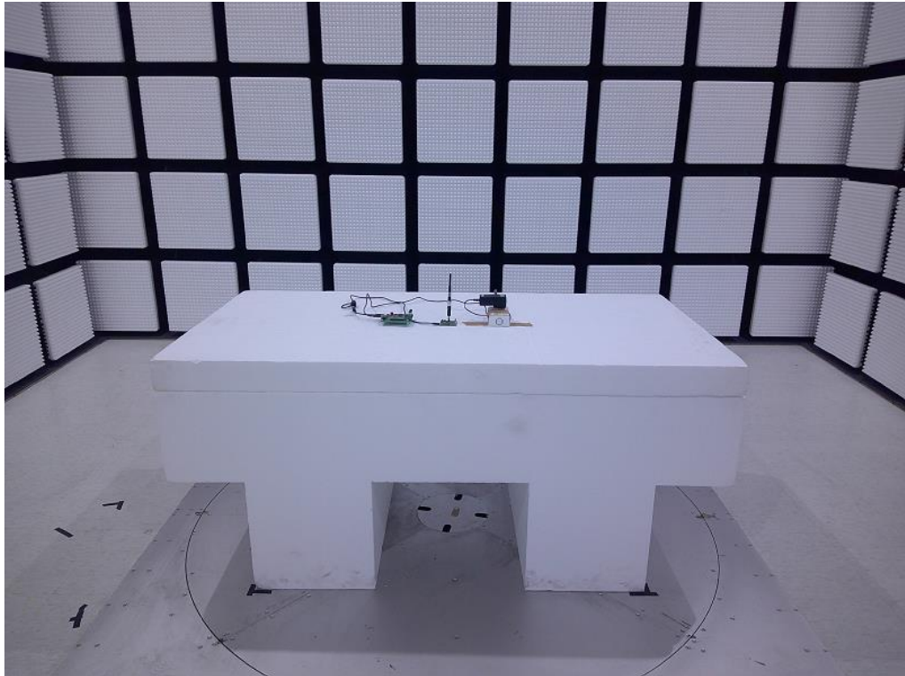
MAYA-W473-00B Dipole
