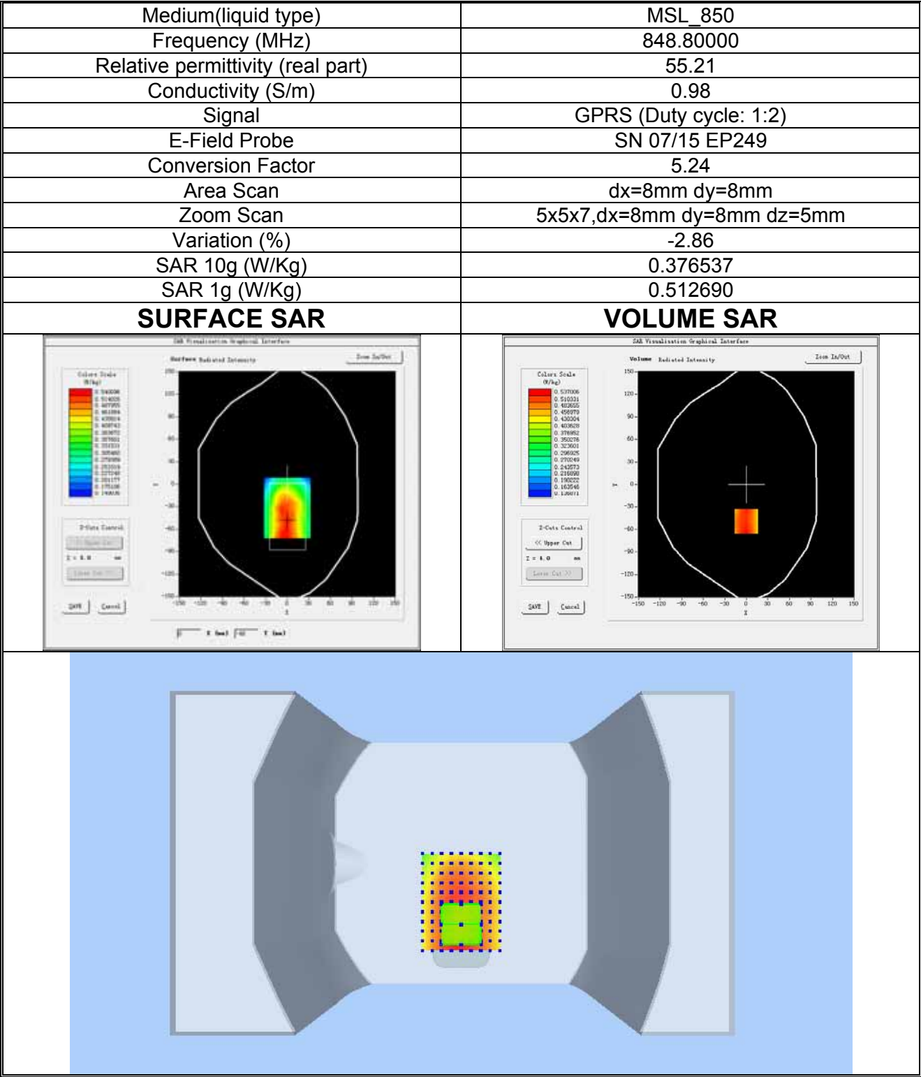
Plot 3: GPRS850MHz, High channel (Body-worn, Back Surface) Product Description:Smart Phone Test Date: 2018-07-04
