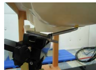
Fig. 17. Head SAR Test Setup
