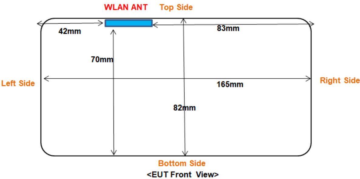
Fig 7.1 Block Diagram for EUT Antenna Position
