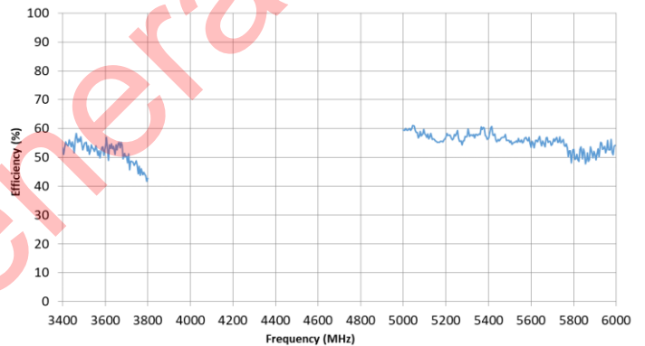
Efficiency (3400-6000 MHz)
