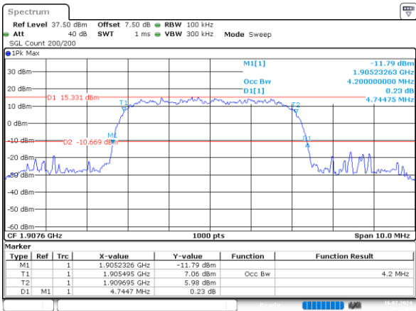
R99_High 4.200MHz
