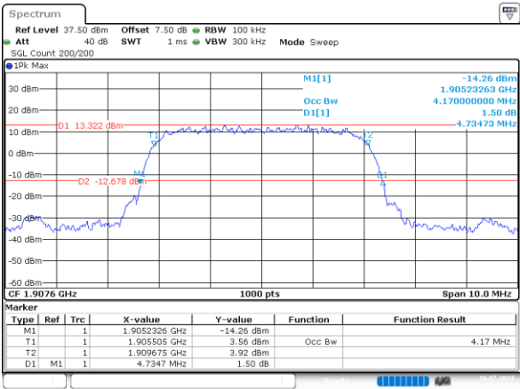
HSDPA_High_Subtest1 4.170MHz
