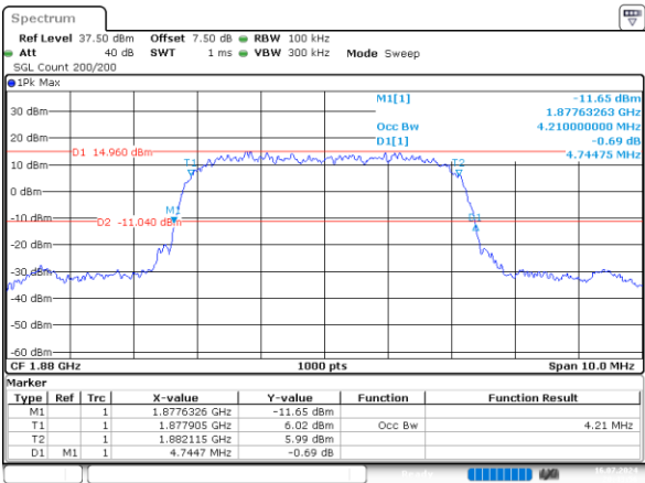
R99_Middle 4.210MHz
