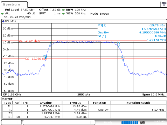
HSDPA_Middle_Subtest1 4.190MHz
