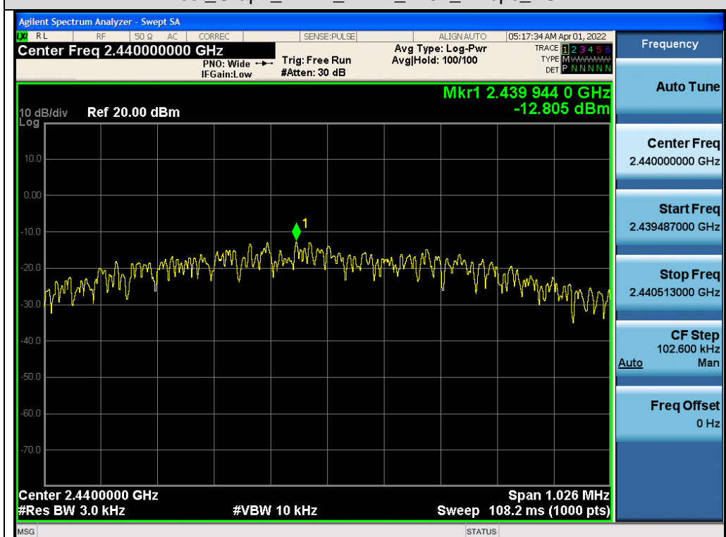
Test_Graph_LE1M_ANT2_2440_1Mbps_PSD
