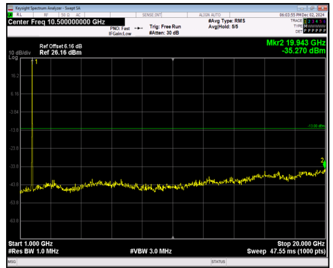
Band66-20MHz-64QAM-132072-1RB#0-Range2:1000~20000MHz
