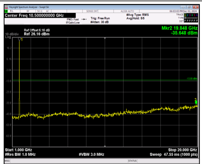
Band66-20MHz-16QAM-132572-1RB#0-Range2:1000~20000MHz
