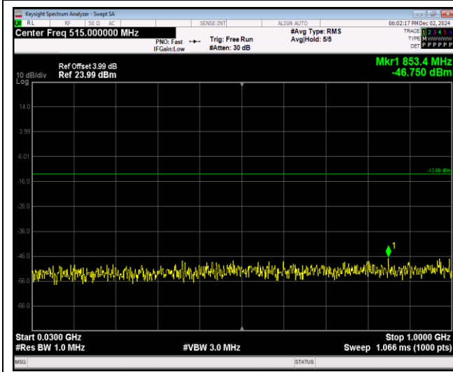
Band66-20MHz-64QAM-132072-1RB#0-Range1:30~1000MHz
