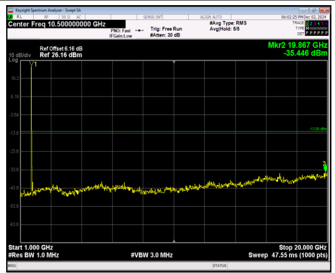
Band66-20MHz-64QAM-132072-1RB#0-Range2:1000~20000MHz
