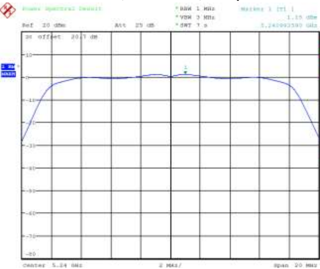
Figure 5-2: Peak Power Spectral Density 802.11a, Channel 48, 6 Mbps
