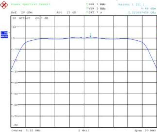
Figure 5-3: Peak Power Spectral Density 802.11a, Channel 64, 6 Mbps
