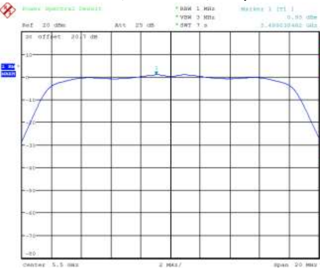
Figure 5-4: Peak Power Spectral Density 802.11a, Channel 100, 6 Mbps
