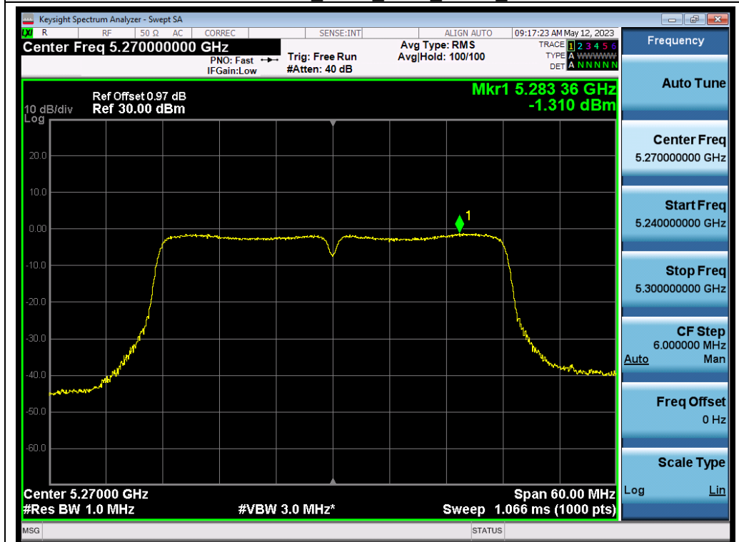
802.11ac40_ANT1_5270_MCS0_PSD
