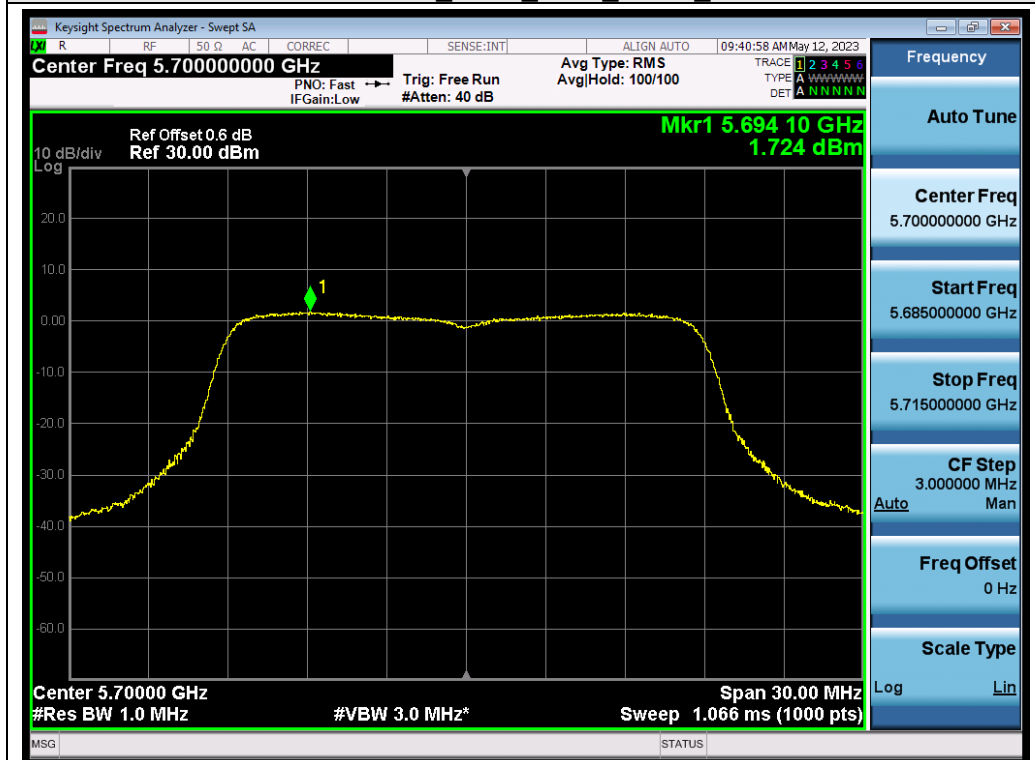
802.11ac20_ANT1_5700_MCS0_PSD
