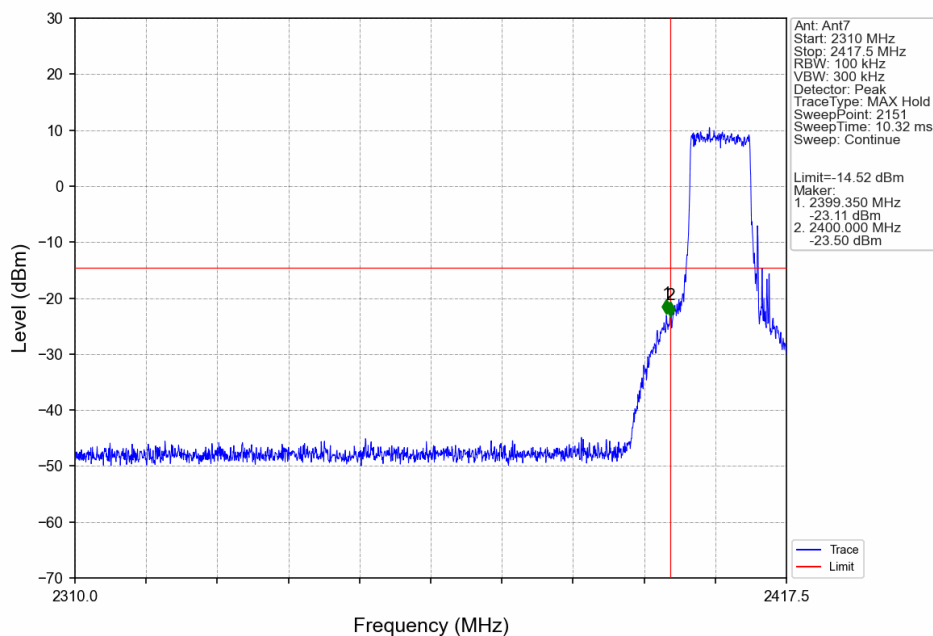
10M_LCH_2407.5MHz_Ant7_NTNV
