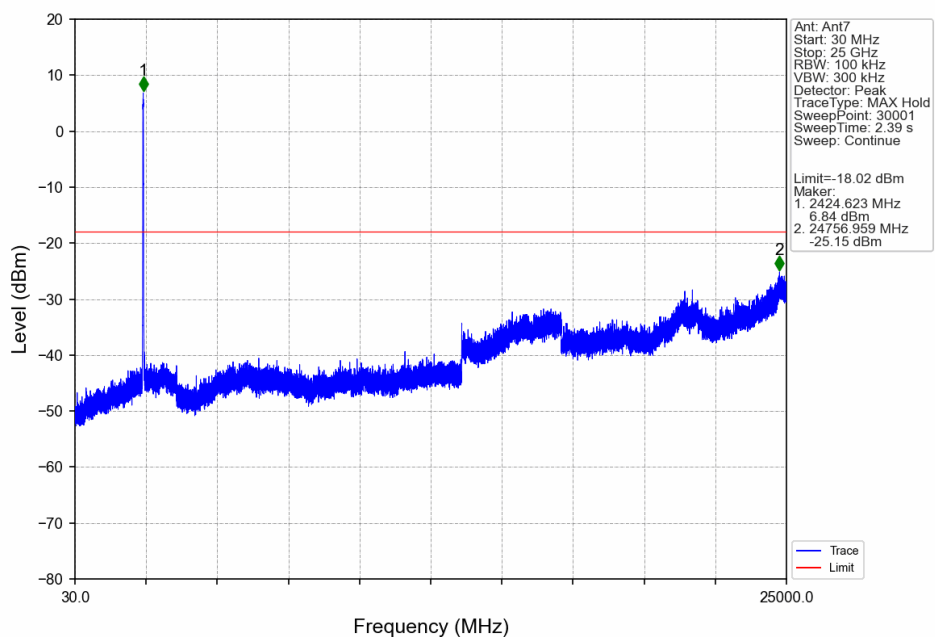
40M_LCH_2422.5MHz_Ant7_NTNV
