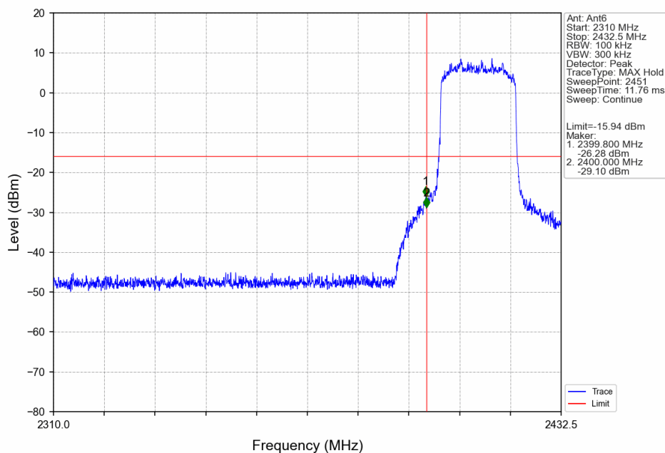
20M_LCH_2412.5MHz_Ant6_NTNV
