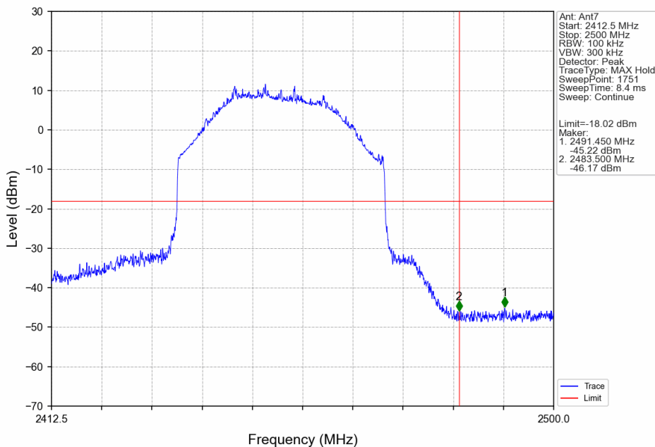
40M_HCH_2452.5MHz_Ant7_NTNV
