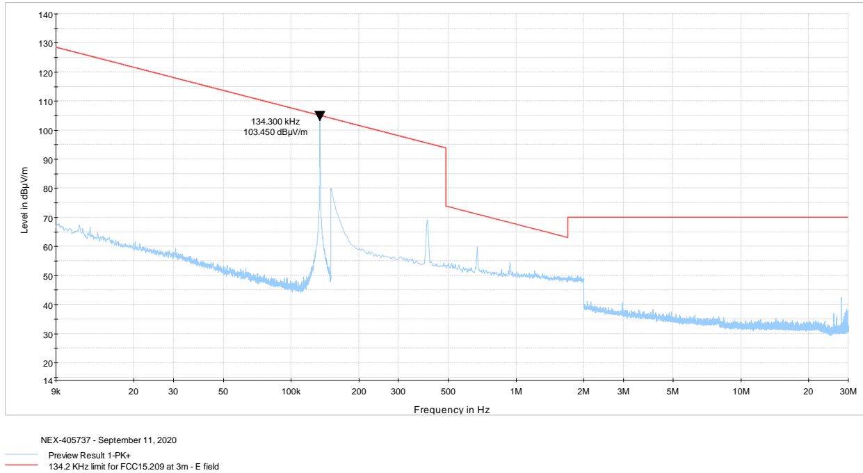
Figure 8.3-1: Radiated spurious emissions below 30 MHz
