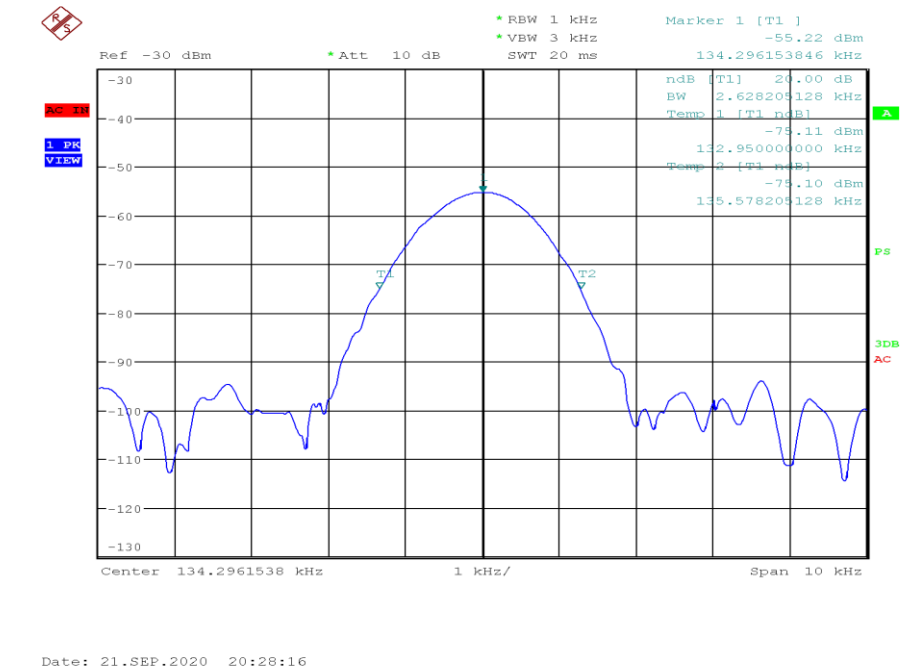
Figure 8.2-1: 20 dB bandwidth
