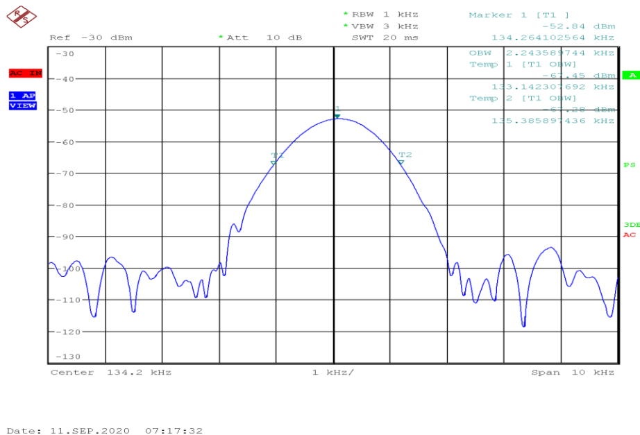
Figure 8.2-2: 99% dB bandwidth
