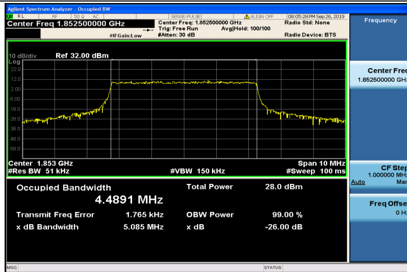
Band2-5MHz-QPSK-18625-25RB#0-4.4891
