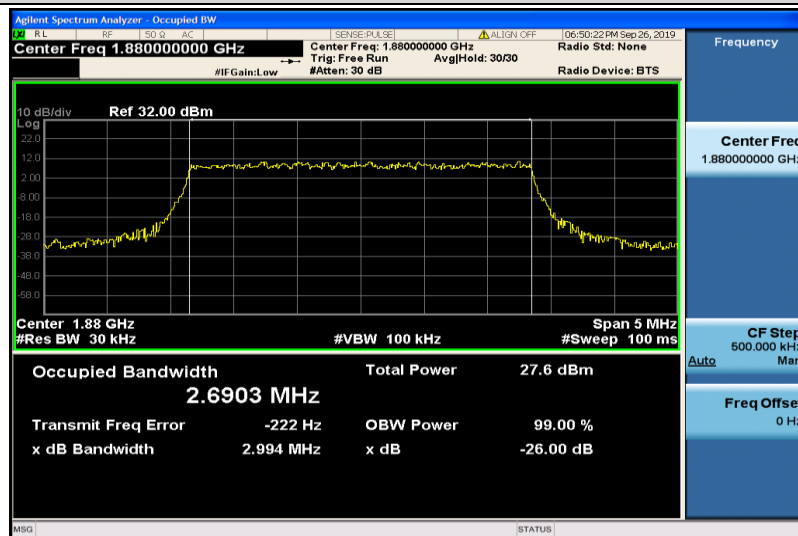
Band2-3MHz-QPSK-18900-15RB#0-2.6903
