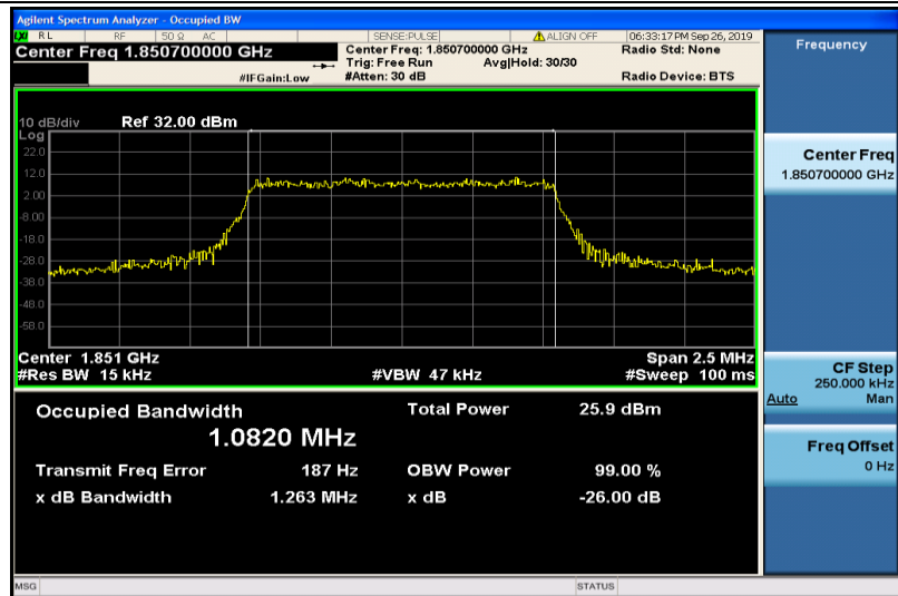
Band2-1.4MHz-16QAM-18607-6RB#0-1.0820
