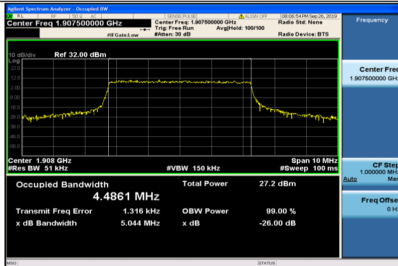
Band2-5MHz-16QAM-19175-25RB#0-4.4861
