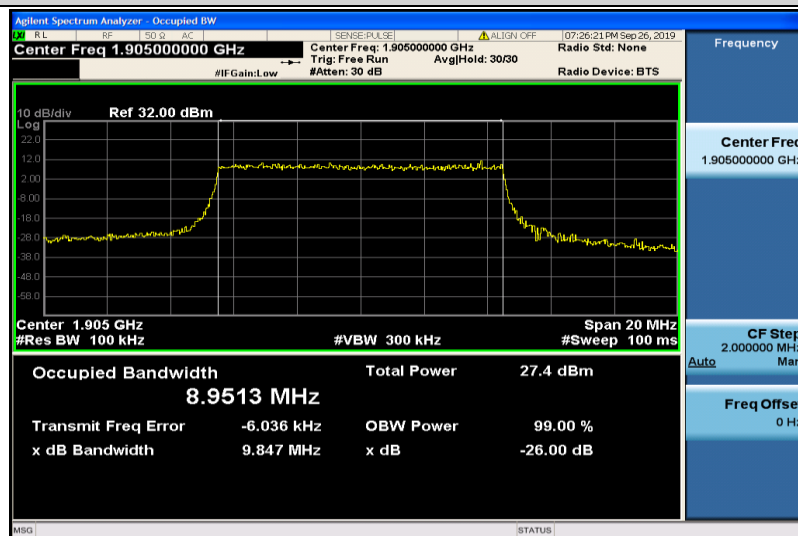
Band2-10MHz-16QAM-19150-50RB#0-8.9513
