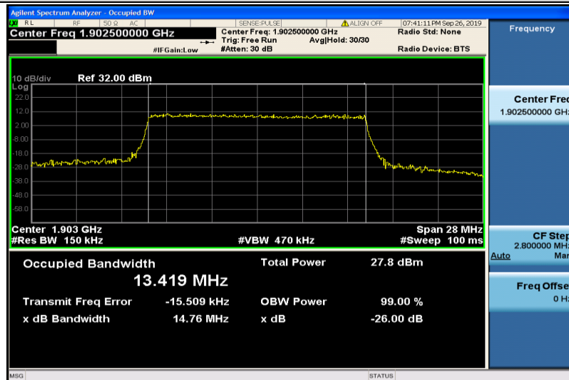
Band2-15MHz-16QAM-19125-75RB#0-13.419
