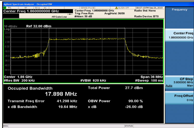
Band2-20MHz-16QAM-18700-100RB#0-17.898
