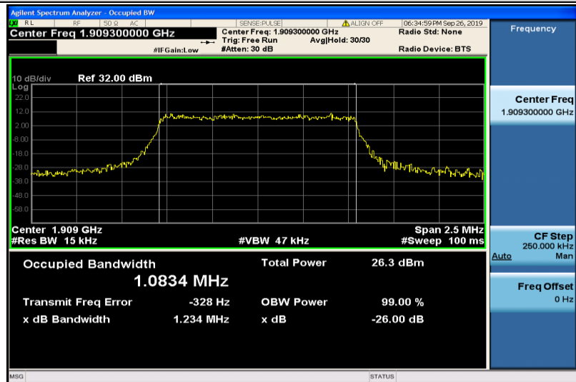
Band2-1.4MHz-16QAM-19193-6RB#0-1.0834
