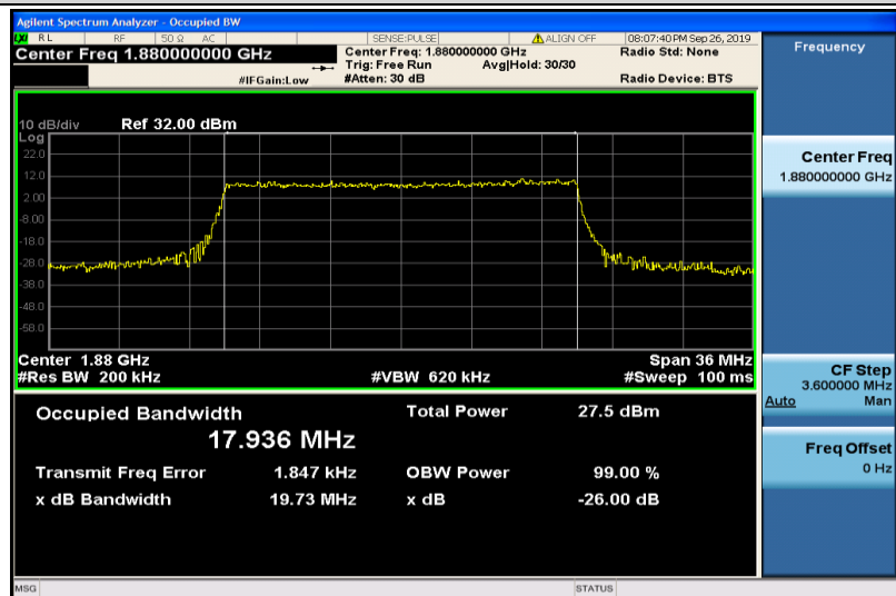
Band2-20MHz-16QAM-18900-100RB#0-17.936
