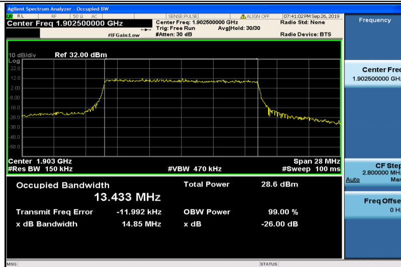
Band2-15MHz-QPSK-19125-75RB#0-13.433
