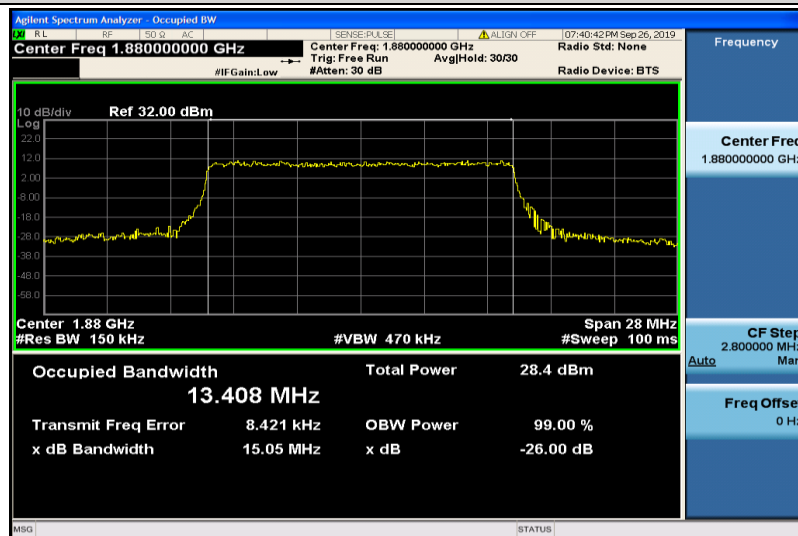
Band2-15MHz-QPSK-18900-75RB#0-13.408
