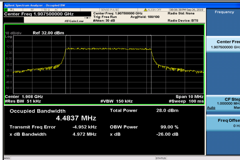
Band2-5MHz-QPSK-19175-25RB#0-4.4837
