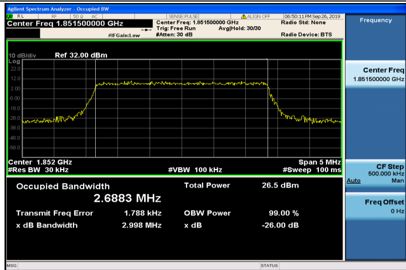
Band2-3MHz-16QAM-18615-15RB#0-2.6883
