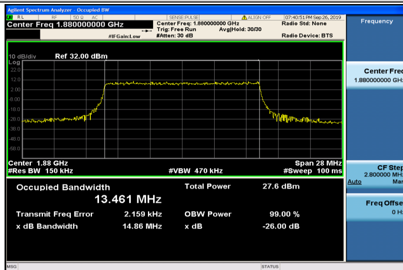
Band2-15MHz-16QAM-18900-75RB#0-13.461
