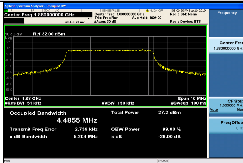
Band2-5MHz-16QAM-18900-25RB#0-4.4855
