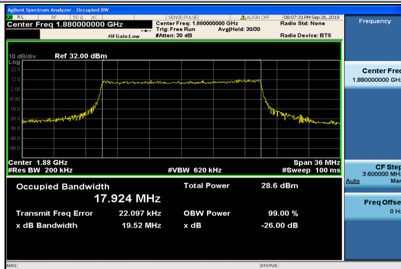
Band2-20MHz-QPSK-18900-100RB#0-17.924
