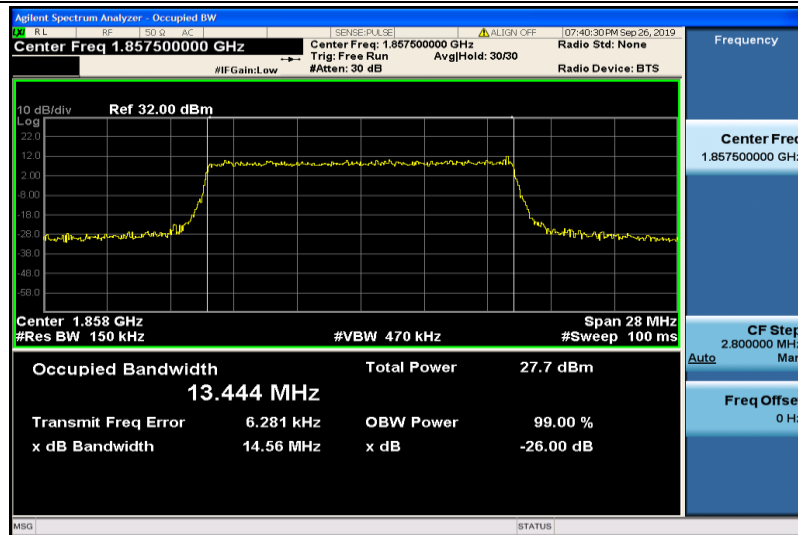
Band2-15MHz-16QAM-18675-75RB#0-13.444
