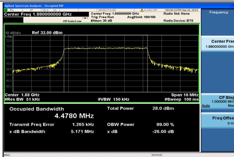
Band2-5MHz-QPSK-18900-25RB#0-4.4780
