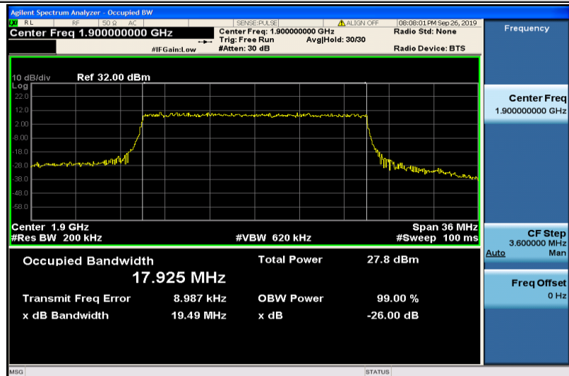
Band2-20MHz-16QAM-19100-100RB#0-17.925
