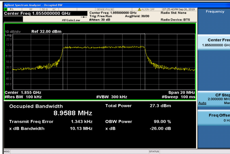
Band2-10MHz-16QAM-18650-50RB#0-8.9588
