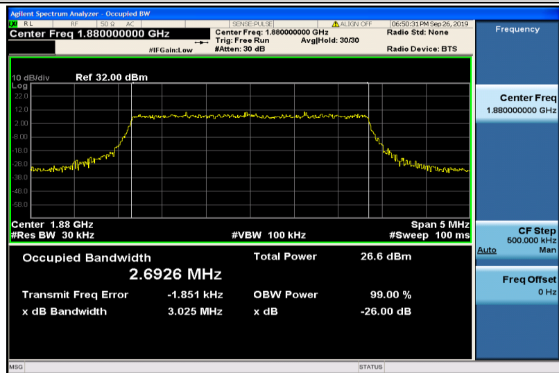
Band2-3MHz-16QAM-18900-15RB#0-2.6926
