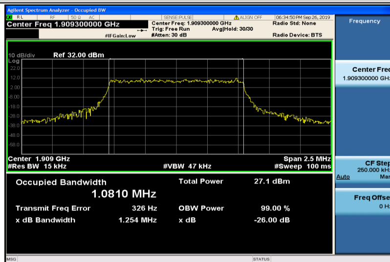
Band2-1.4MHz-QPSK-19193-6RB#0-1.0810
