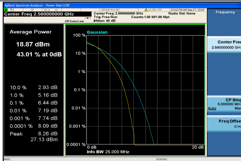
Band7-20MHz-16QAM-21350-100RB#0
