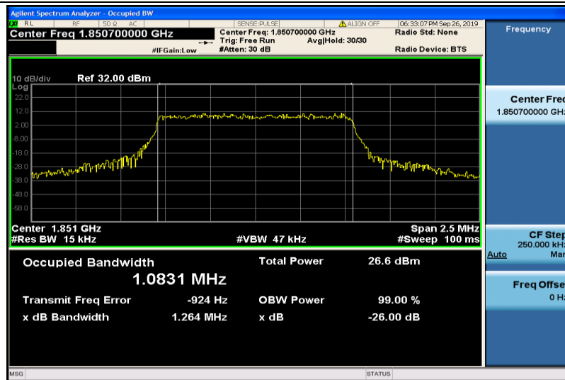
Band2-1.4MHz-QPSK-18607-6RB#0-1.0831
