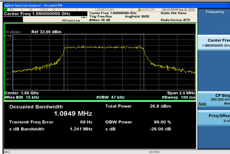
Band2-1.4MHz-QPSK-18900-6RB#0-1.0849
