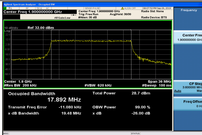
Band2-20MHz-QPSK-19100-100RB#0-17.892
