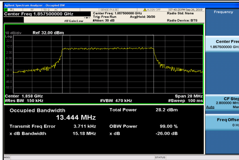
Band2-15MHz-QPSK-18675-75RB#0-13.444
