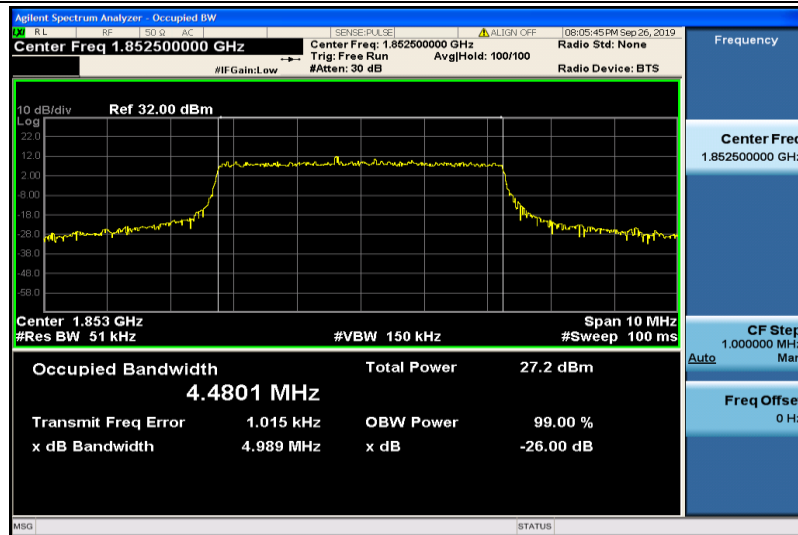
Band2-5MHz-16QAM-18625-25RB#0-4.4801
