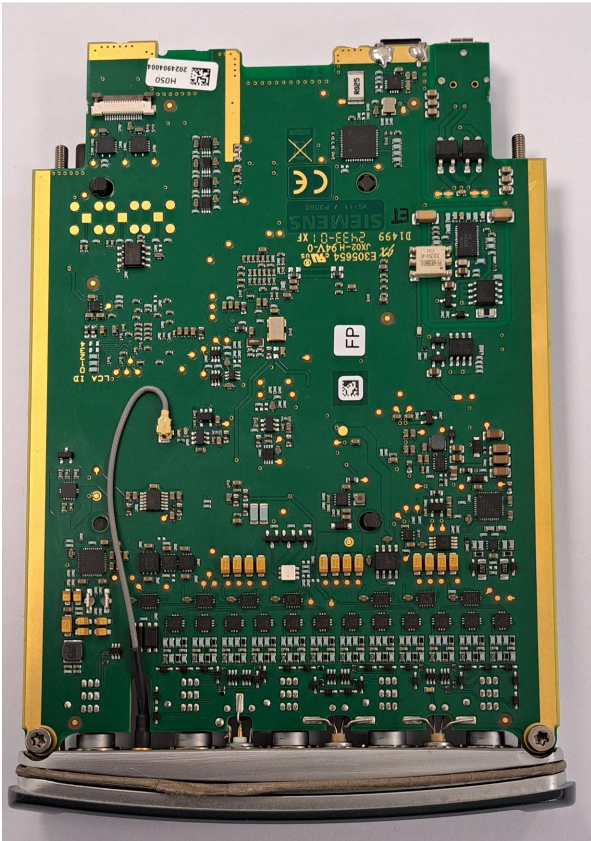
SC-XS12 bottom view
