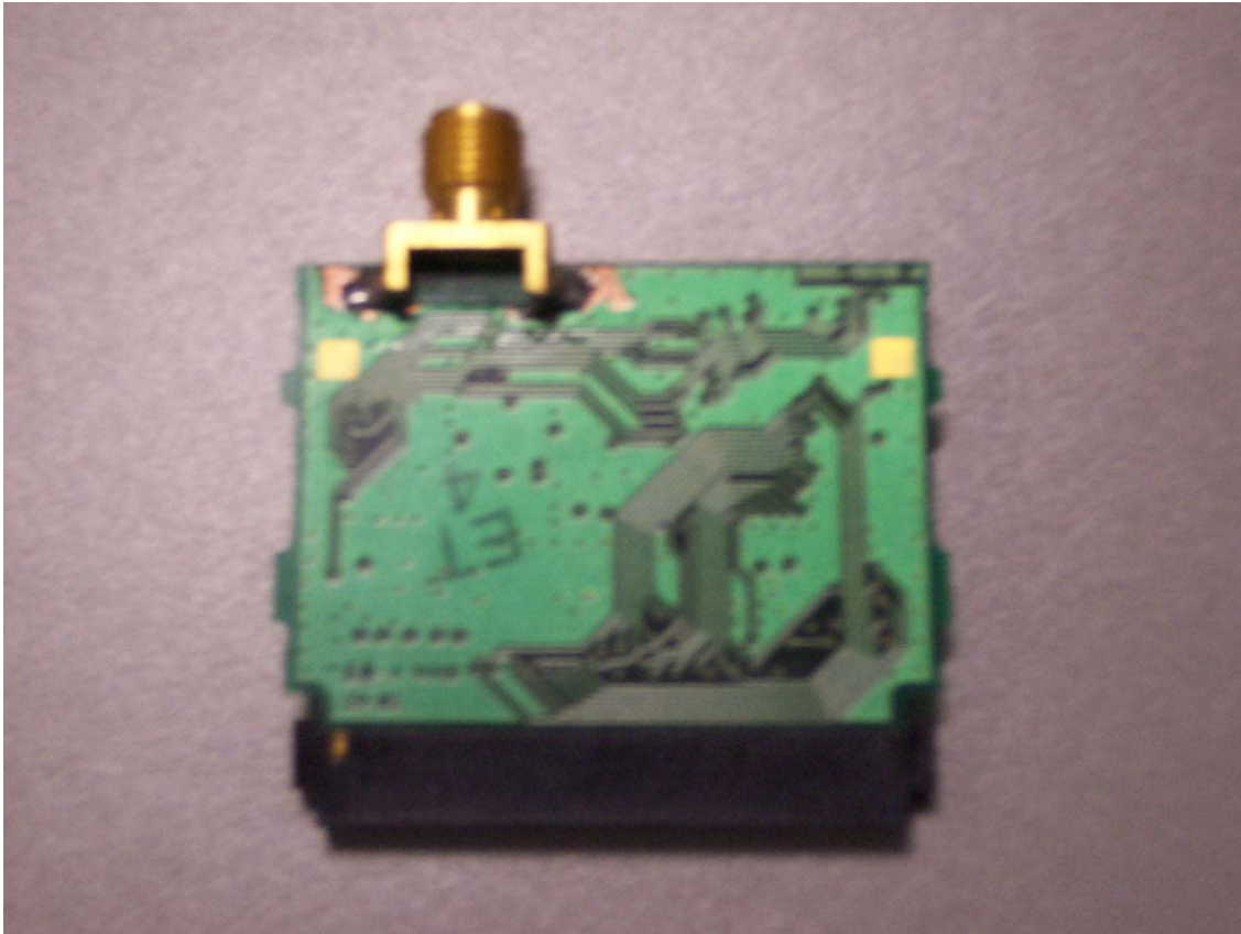
EUT PCB – Solder Side
