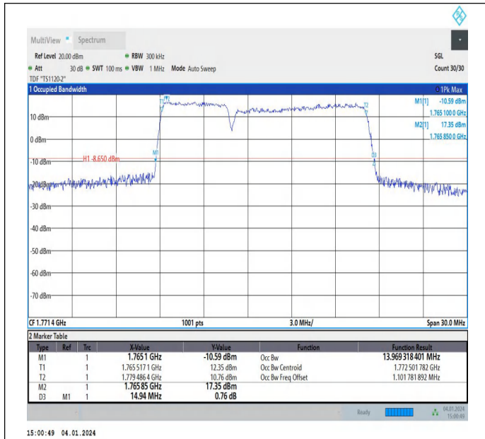
66-66-5MHz-10MHz-64QAM-64QAM-132550-132622-25RB# 0-50RB#0-PASS
