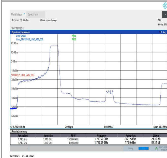
5MHz-15MHz_QPSK@QPSK-QPSK@QPSK_132002-13209 5_1RB#24@25RB#0-0RB#0@75RB#0
