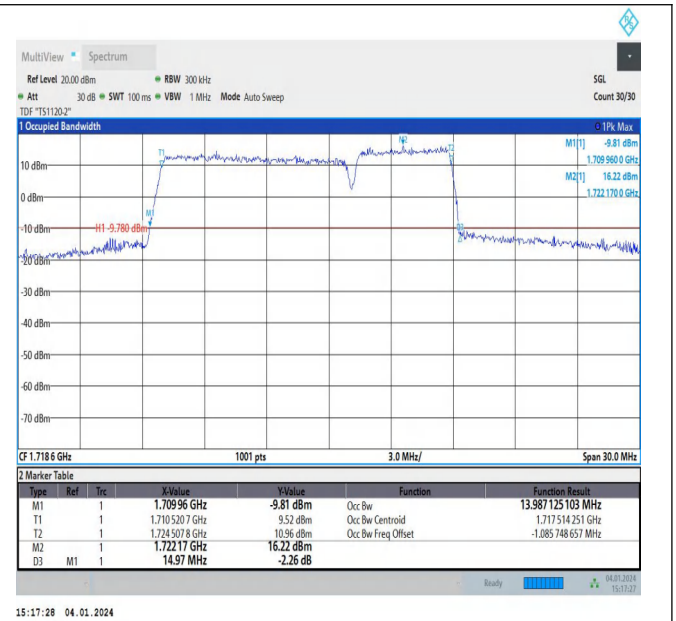
66-66-10MHz-5MHz-64QAM-64QAM-132022-132094-50RB# 0-25RB#0-PASS
