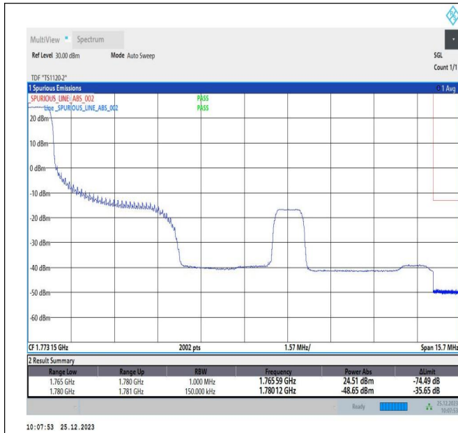
5MHz-10MHz_QPSK@QPSK-QPSK@QPSK_132550-13262 2_1RB#0@25RB#0-0RB#0@50RB#0
