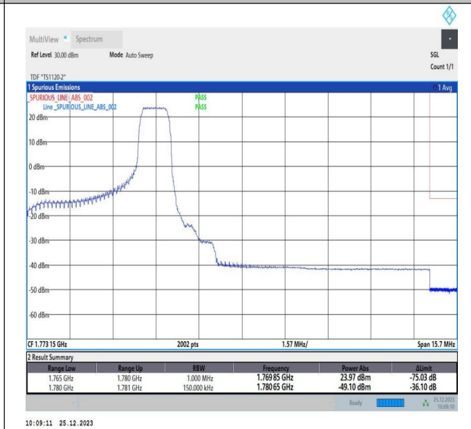
5MHz-10MHz_16QAM@16QAM-16QAM@16QAM_132550-132622_1RB#24@25RB#0-0RB#0@50RB#0
