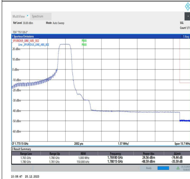
5MHz-10MHz_QPSK@QPSK-QPSK@QPSK_132550-13262 2_1RB#24@25RB#0-0RB#0@50RB#0
