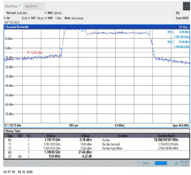
66-66-5MHz-15MHz-64QAM-64QAM-132353-132446-25RB# 0-75RB#0-PASS
