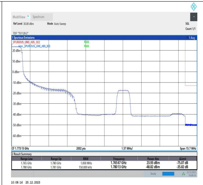
5MHz-10MHz_16QAM@16QAM-16QAM@16QAM_132550-132622_1RB#0@25RB#0-0RB#0@50RB#0
