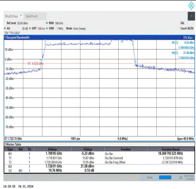
66-66-15MHz-5MHz-64QAM-64QAM-132047-132140-75RB# 0-25RB#0-PASS
