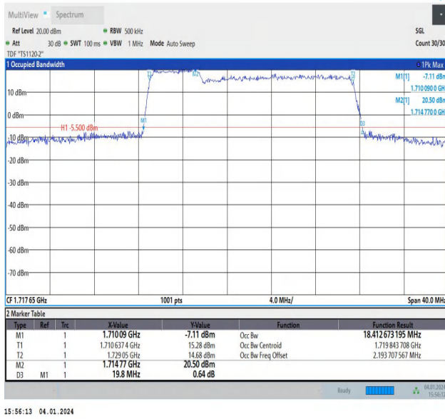
66-66-5MHz-15MHz-64QAM-64QAM-132002-132095-25RB# 0-75RB#0-PASS
