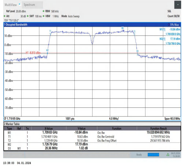
66-66-10MHz-10MHz-64QAM-64QAM-132022-132121-50RB#0-50RB#0-PASS
