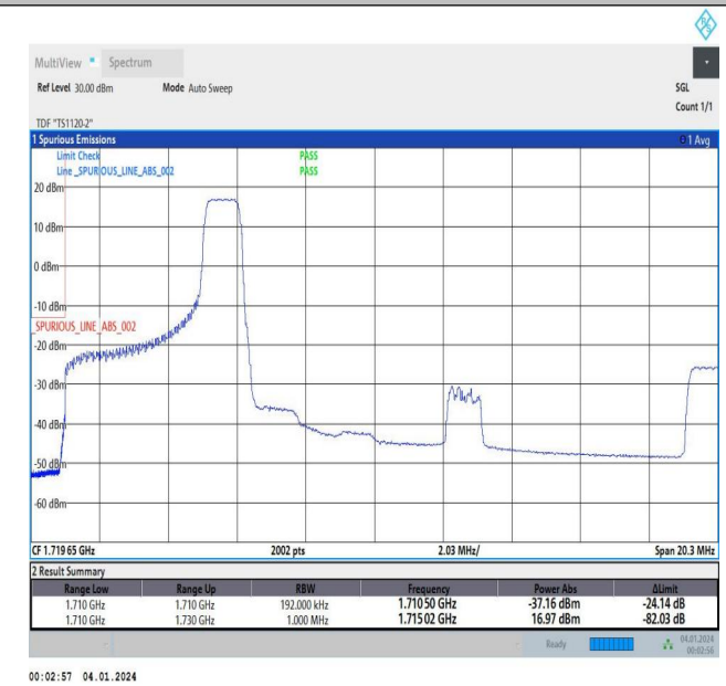
5MHz-15MHz_16QAM@16QAM-16QAM@16QAM_132002-1 32095_1RB#24@25RB#0-0RB#0@75RB#0
