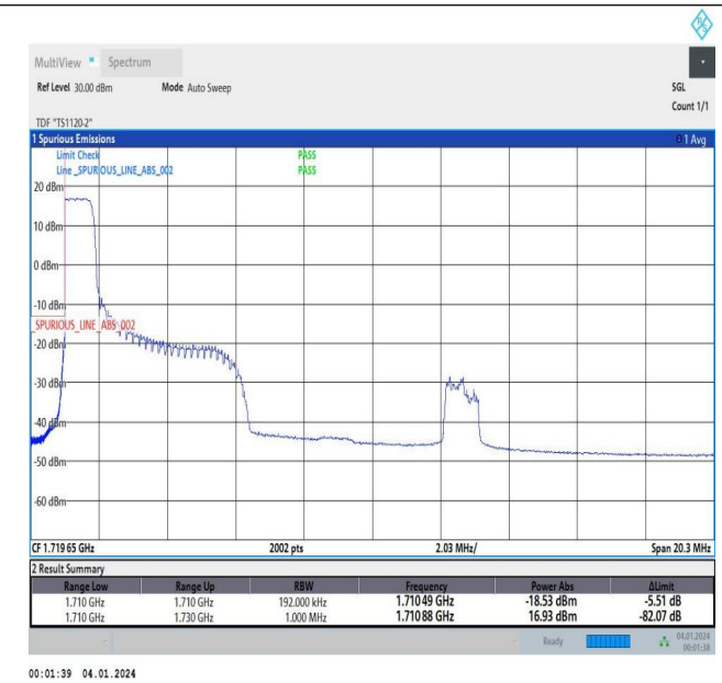
5MHz-15MHz_16QAM@16QAM-16QAM@16QAM_132002-1 32095_1RB#0@25RB#0-0RB#0@75RB#0
