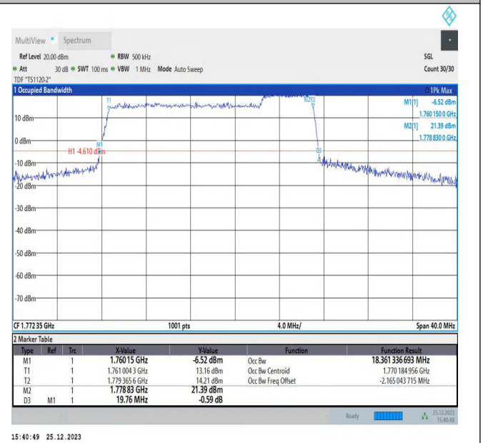
66-66-15MHz-5MHz-16QAM-16QAM-132549-132642-75RB# 0-25RB#0-PASS
