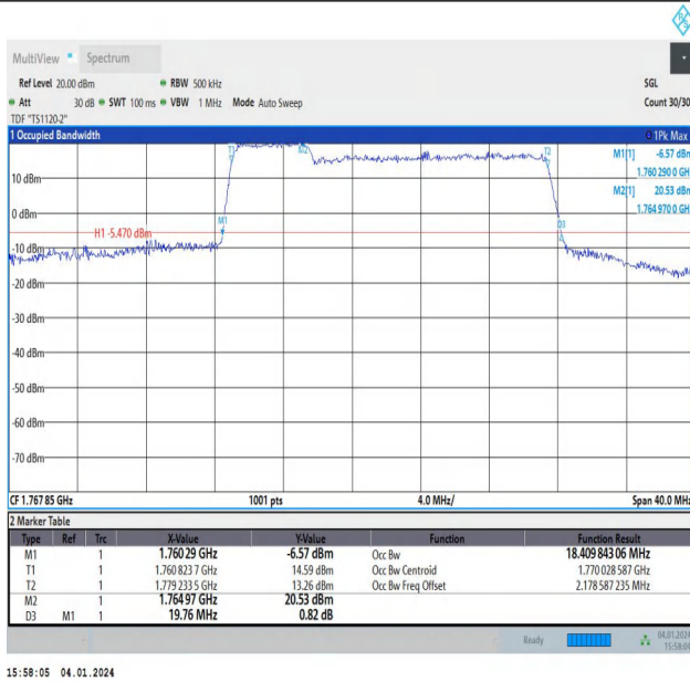
66-66-5MHz-15MHz-64QAM-64QAM-132504-132597-25RB# 0-75RB#0-PASS
