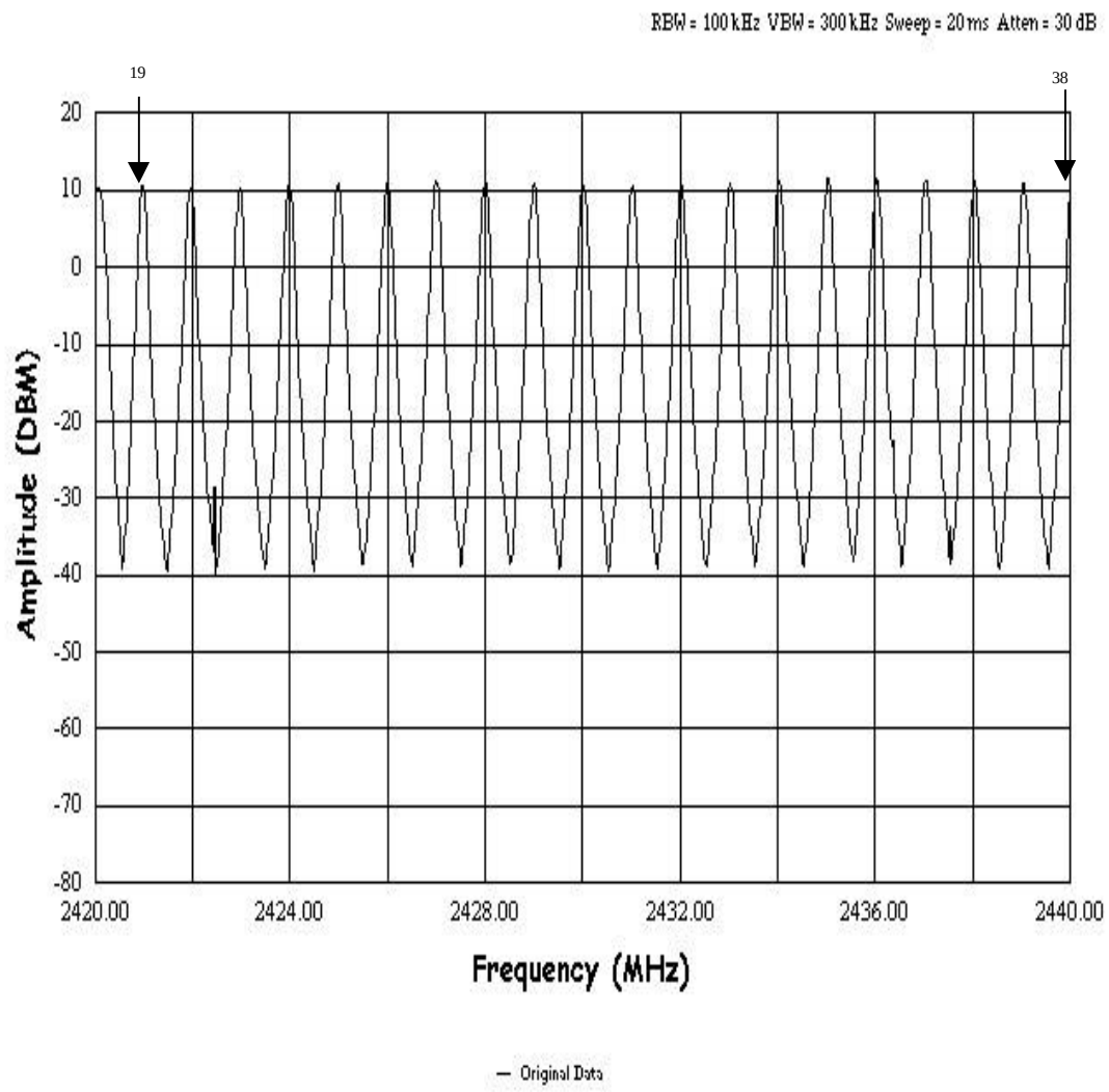
F3: 2.42-2.44GHz HOPPING CHANNELS 19-38
