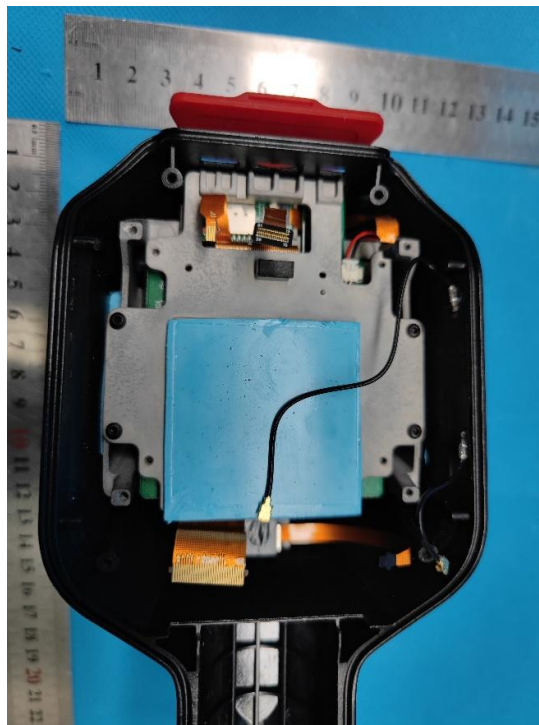
Wi-Fi & Bluetooth Antenna, GPS Antenna
