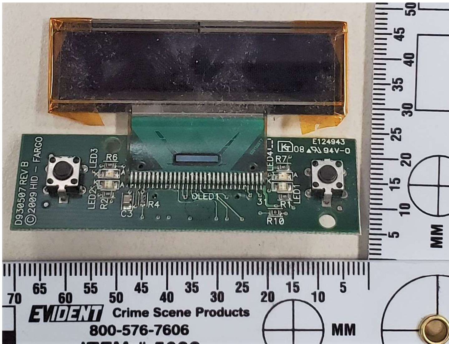
OLED Display Board Top Side
