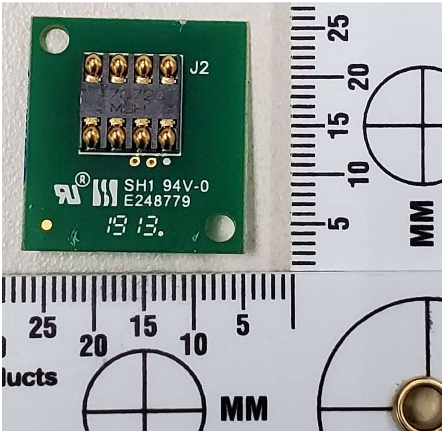
Contact Encoder Board Bottom Side
