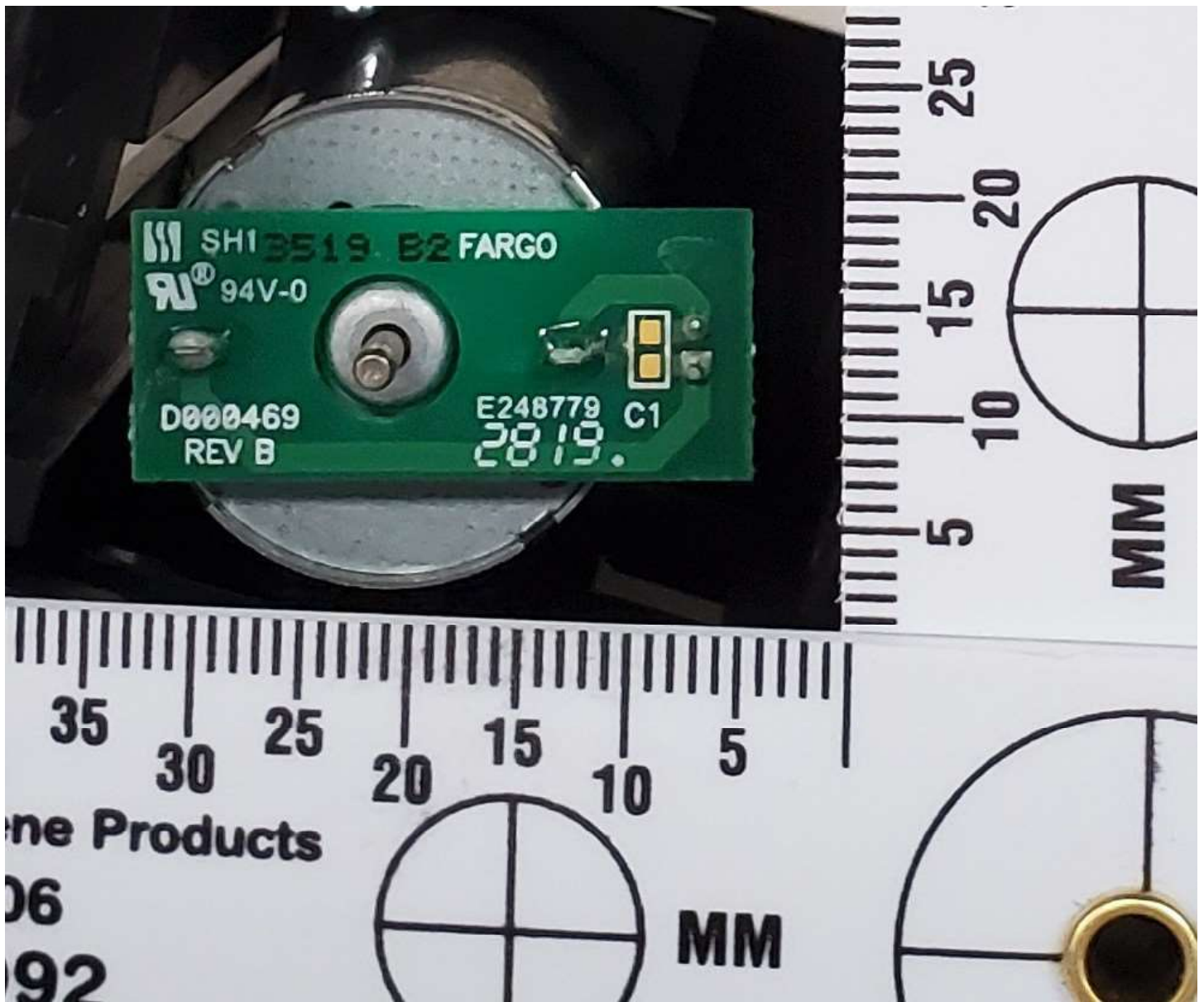
DC Motor board (no components, single sided)
