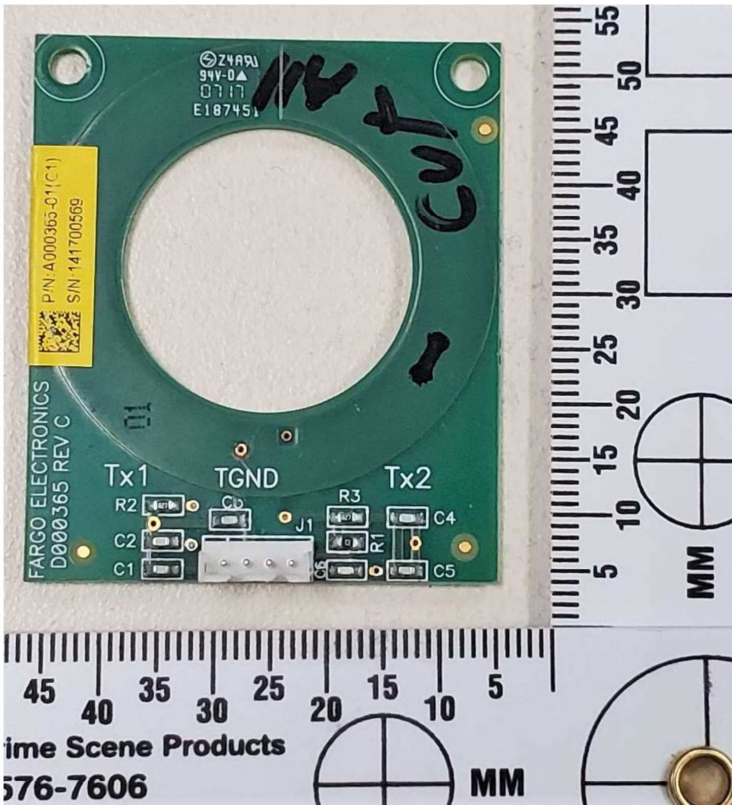
Ribbon Antenna Board Top Side
