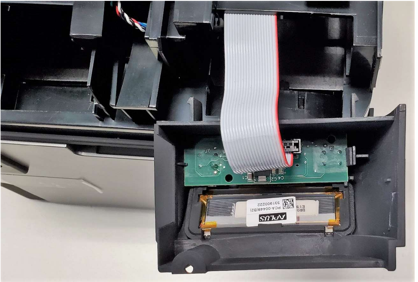
OLED Display Mounted
