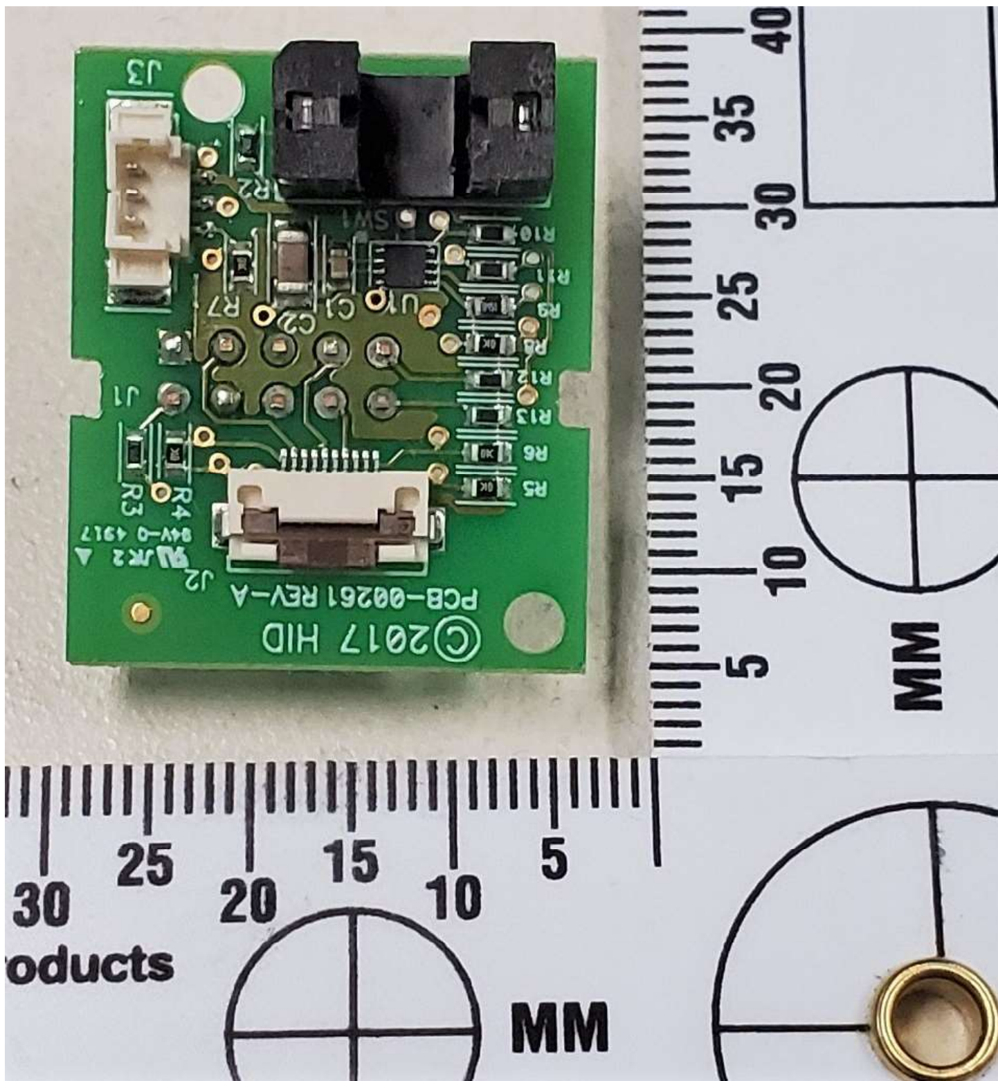
Contact Encoder Interface Board Top Side
