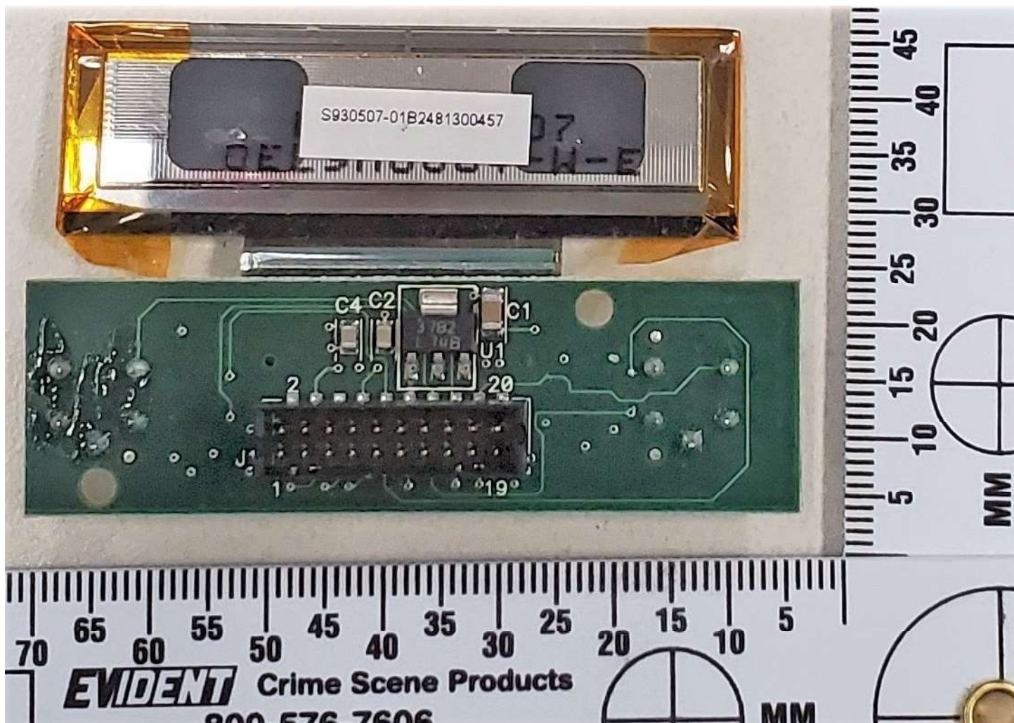
OLED Display Board Bottom Side
