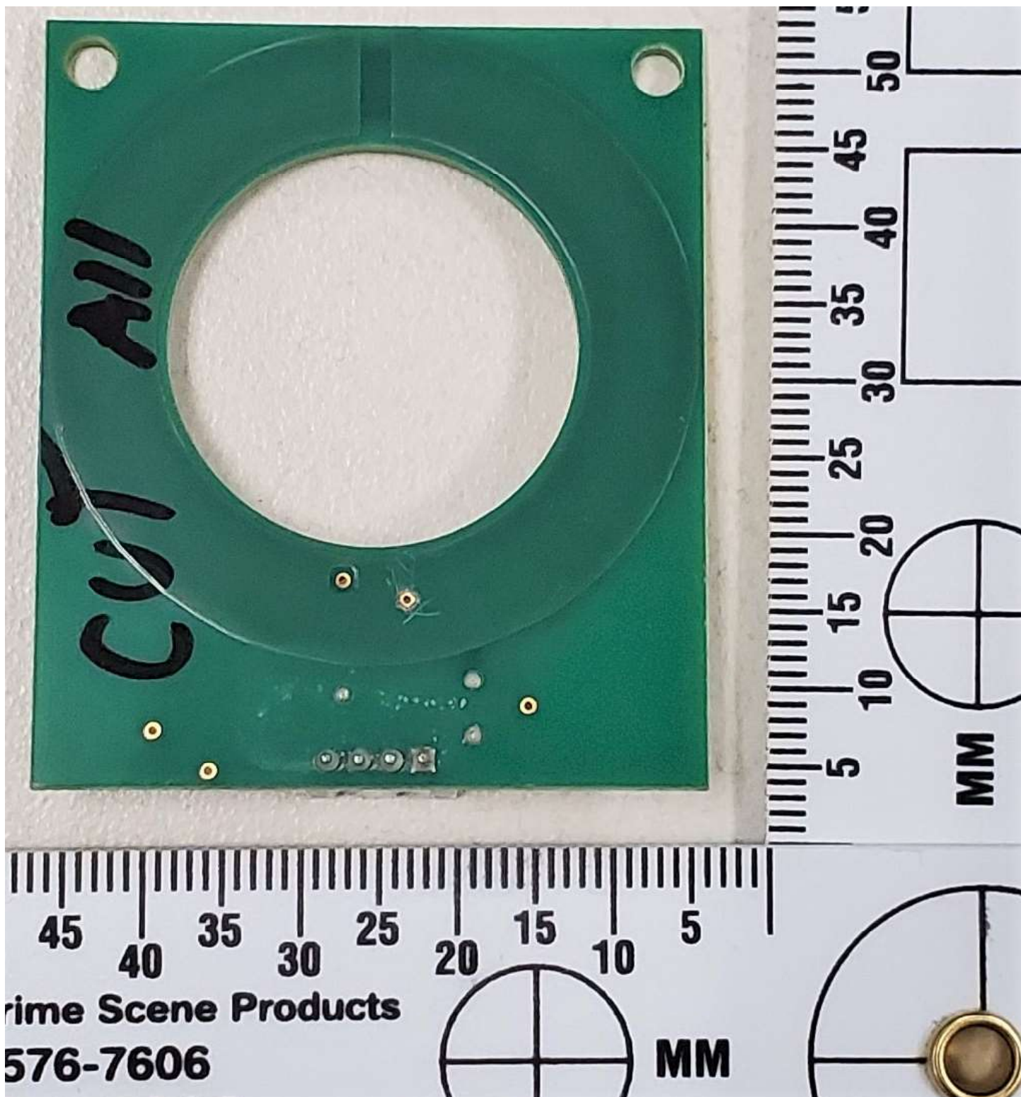
Ribbon Antenna Board Bottom Side
