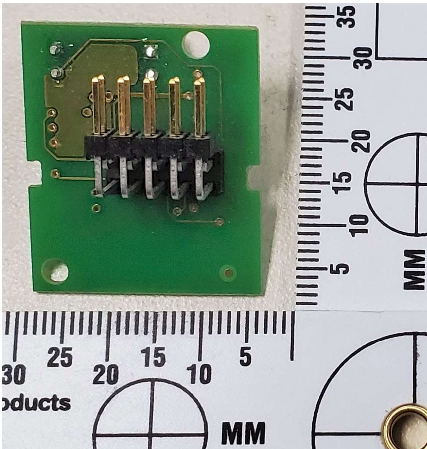
Contact Encoder Interface Board Bottom Side
