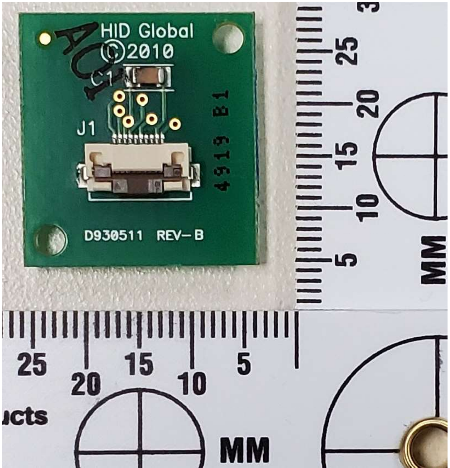
Contact Encoder Board Top Side
