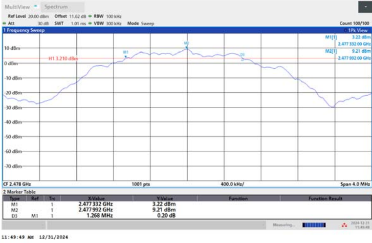
BLE_2M-Ant1-2478-PASS
