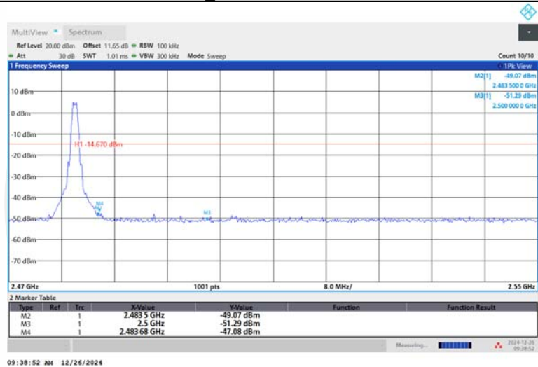
BLE_1M-Ant1-2480-PASS
