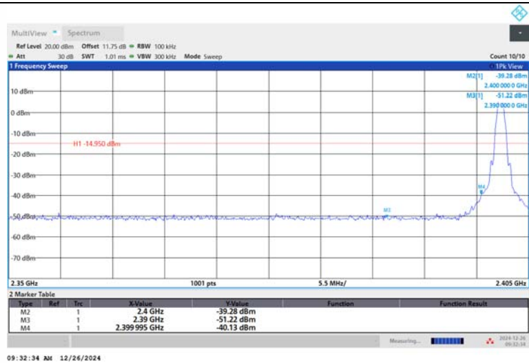
BLE_1M-Ant1-2402-PASS
