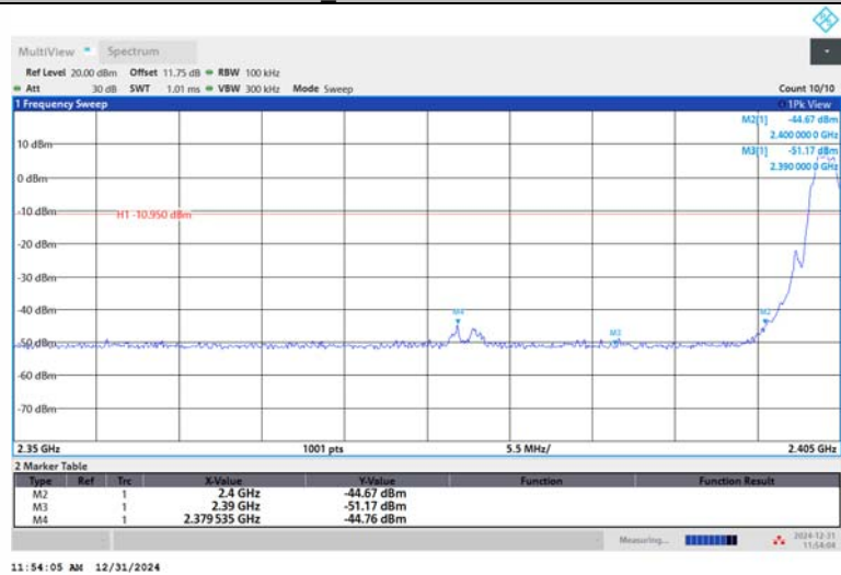
BLE_2M-Ant1-2404-PASS
