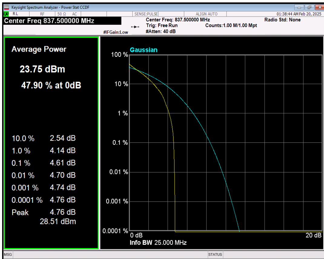
Band19 16QAM BW=10MHz Channel=24075 RB Size=1 Position=#0
