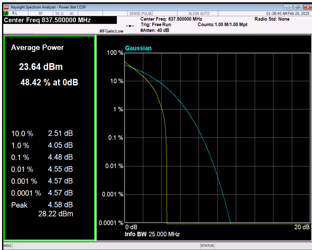
Band19 16QAM BW=5MHz Channel=24075 RB Size=1 Position=#0
