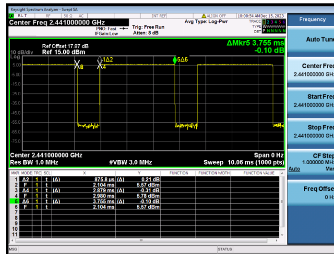
Bluetooth-GFSK
