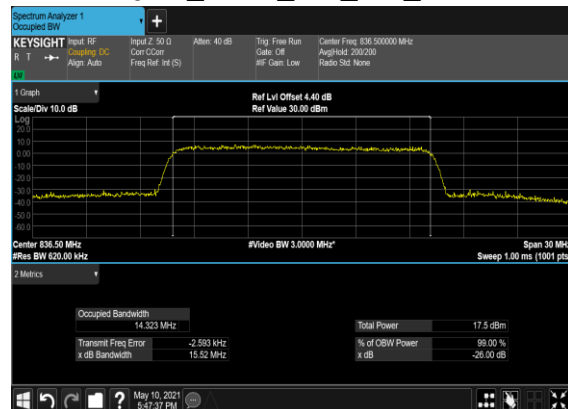
B7_N5(15M)_CP-OFDM_256 QAM_Outer_Full_Mid_CH
