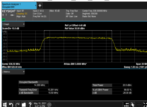
B7_N5(15M)_CP-OFDM_64 QAM_Outer_Full_Mid_CH
