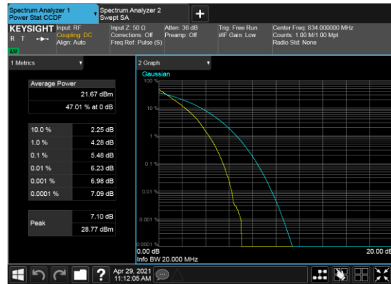
B7_N5(20M)_DFT-s- OFDM_QPSK_Outer_Full_Low_CH
