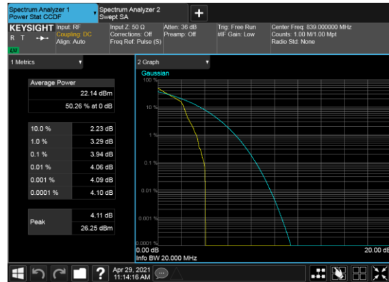
B7_N5(20M)_DFT-s-OFDM_PI_2-BPSK_Edge_1RB_Left_High_CH
