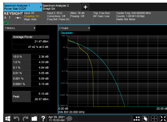
B7_N5(20M)_DFT-s-OFDM_QPSK_Edge_1RB_Right_High_C H
