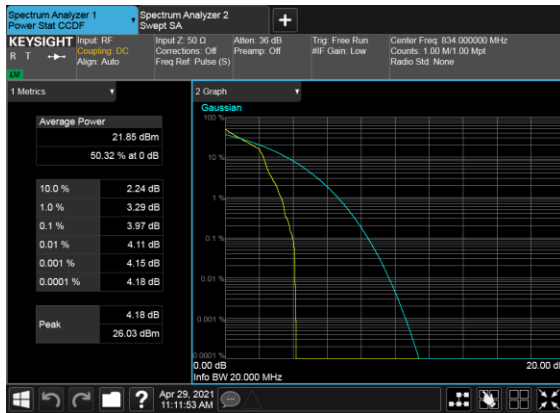
B7_N5(20M)_DFT-s-OFDM_PI_2- BPSK_Edge_1RB_Right_Low_CH
