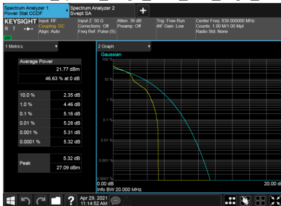
B7_N5(20M)_DFT-s-OFDM_QPSK_Edge_1RB_Left_High_CH
