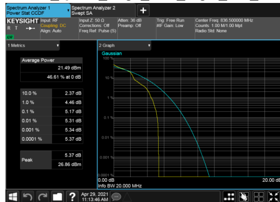
B7_N5(20M)_DFT-s- OFDM_QPSK_Edge_1RB_Right_Mid_CH
