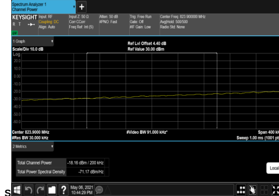
B7_N5(20M)_DFT-s- OFDM_BPSK_Edge_1RB_Left_Low_CH_CHP_PAS
