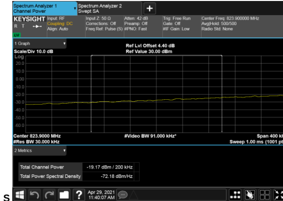
B7_N5(20M)_DFT-s- OFDM_QPSK_Edge_1RB_Left_Low_CH_CHP_PAS
