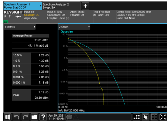
B7_N5(20M)_DFT-s-OFDM_QPSK_Outer_Full_High_CH
