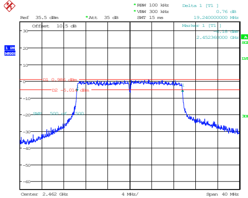
802.11ax20_2462MHz_RU_Full_Chain 1
