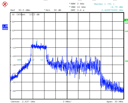
802.11ax20_2437MHz_RU_52/37_Chain 1
