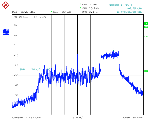
802.11ax20_2462MHz_RU_52/40_Chain 1
