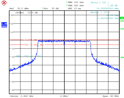
802.11ax20_2462MHz_RU_Full_Chain 0
