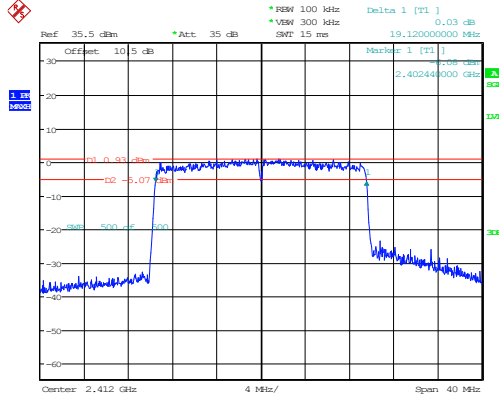
802.11ax20_2412MHz_RU_Full_Chain 1
