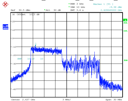
802.11ax20_2437MHz_RU_106/53_Chain 0
