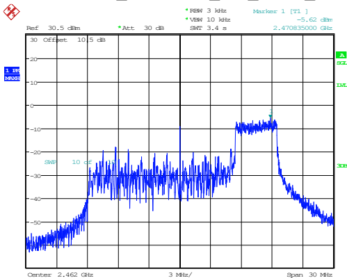
802.11ax20_2462MHz_RU_52/40_Chain 0
