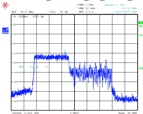
802.11ax20_2412MHz_RU_106/53_Chain 1
