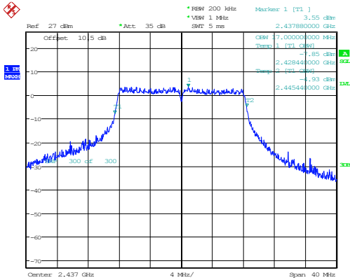
802.11g_2437MHz_Chain 1
