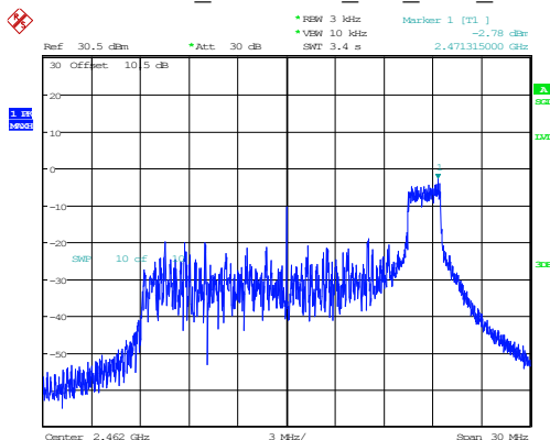
802.11ax20_2462MHz_RU_26/8_Chain 1
