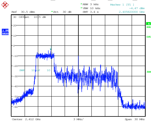
802.11ax20_2412MHz_RU_52/37_Chain 1
