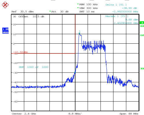
802.11ax20_2412MHz_RU_26/0_Chain 1
