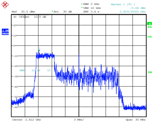
802.11ax20_2412MHz_RU_52/37_Chain 0
