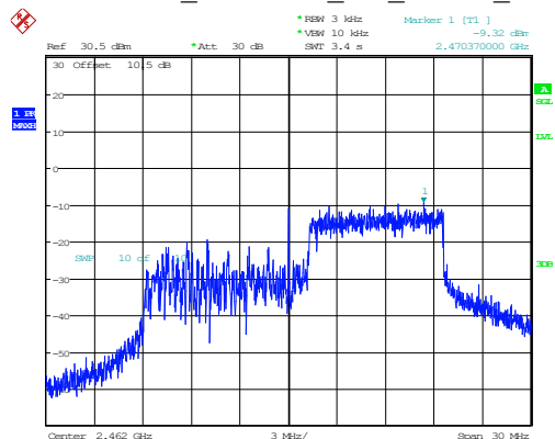
802.11ax20_2462MHz_RU_106/54_Chain 1
