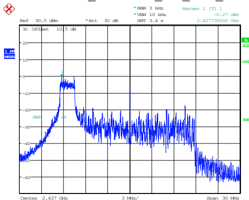
802.11ax20_2437MHz_RU_26/0_Chain 1
