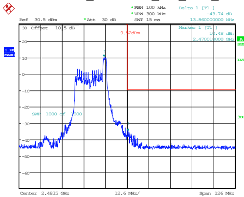
802.11ax20_2462MHz_RU_26/8_Chain 1
