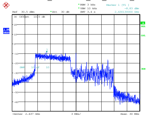
802.11ax20_2437MHz_RU_106/53_Chain 1
