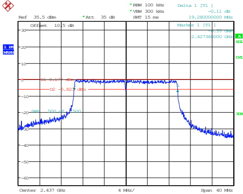
802.11ax20_2437MHz_RU_Full_Chain 1
