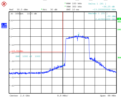
802.11ax20_2412MHz_RU_Full_Chain 1
