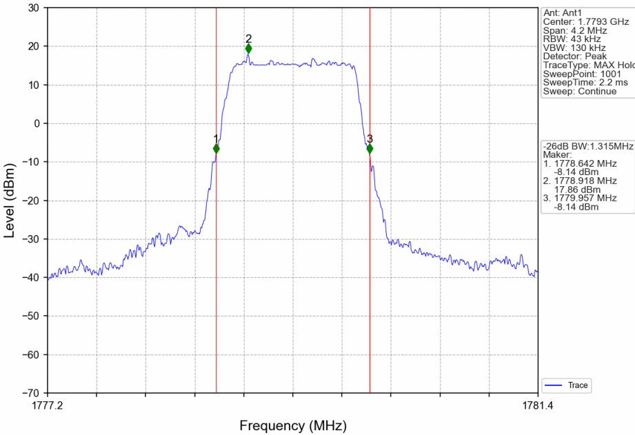
Band66_1.4MHz_16QAM_HCH_1779.3MHz_RB_6_0_NTNV
