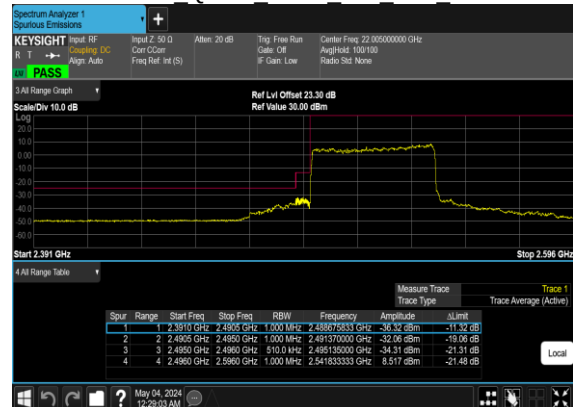
N41(50M)_DFT-s- OFDM QPSK Outer Full Low CH
