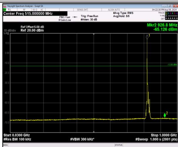
5-5-5MHz-3MHz-16QAM-16QAM-20425-20464-1RB#0-0 RB#0-30~1000MHz-PASS
