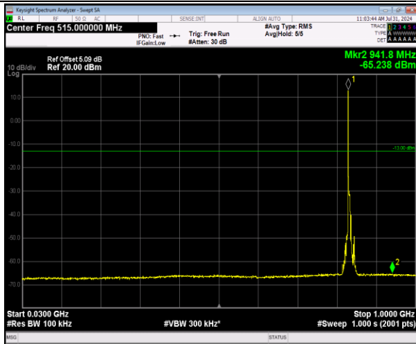
5-5-5MHz-3MHz-64QAM-64QAM-20510-20549-1RB#0-0RB#0-30~1000MHz-PASS
