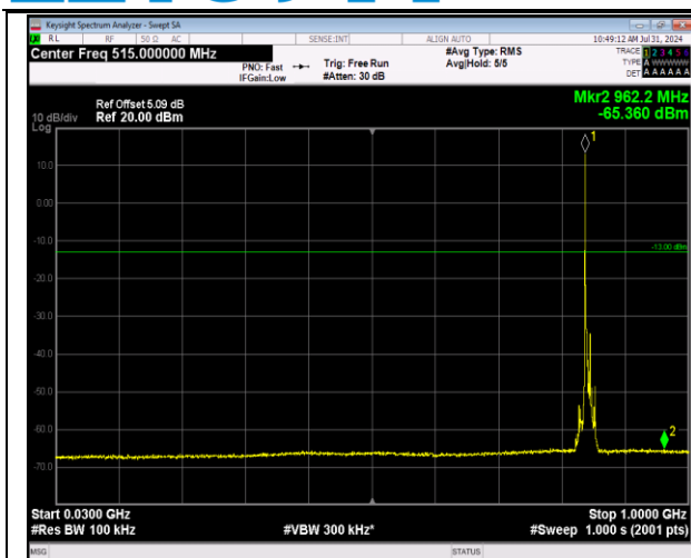
5-5-3MHz-5MHz-64QAM-64QAM-20586-20625-1RB#0-1 RB#24-30~1000MHz-PASS
