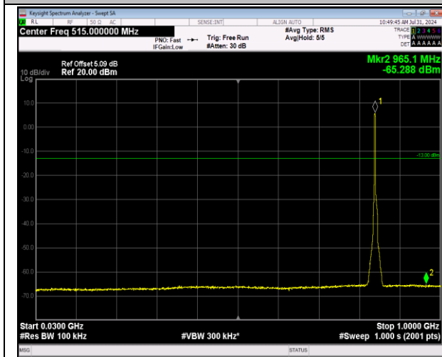
5-5-3MHz-5MHz-64QAM-64QAM-20586-20625-15RB#0- 25RB#0-30~1000MHz-PASS
