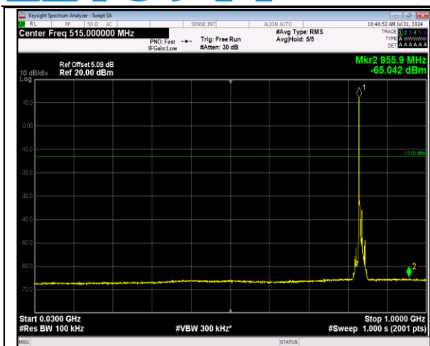
5-5-3MHz-5MHz-64QAM-64QAM-20501-20540-1RB#0-1 RB#24-30~1000MHz-PASS
