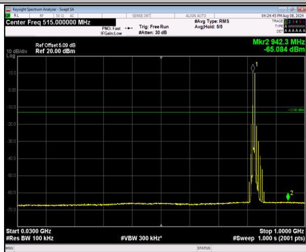
5-5-5MHz-3MHz-16QAM-16QAM-20425-20464-1RB#0-1 RB#15-30~1000MHz-PASS
