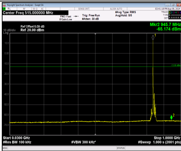
5-5-3MHz-5MHz-16QAM-16QAM-20586-20625-1RB#0-0 RB#0-30~1000MHz-PASS
