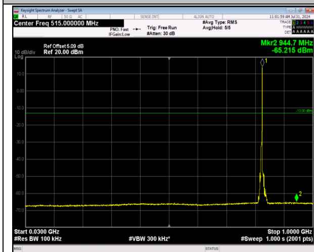
5-5-5MHz-3MHz-64QAM-64QAM-20425-20464-1RB#24- ORB#0-30~1000MHz-PASS
