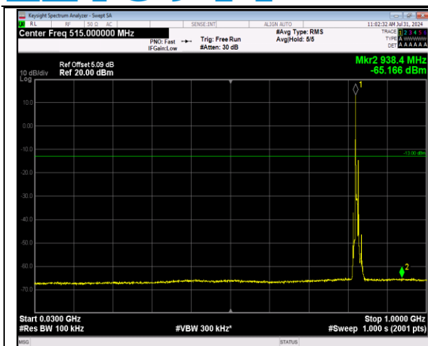
5-5-5MHz-3MHz-64QAM-64QAM-20425-20464-1RB#0-1 RB#15-30~1000MHz-PASS
