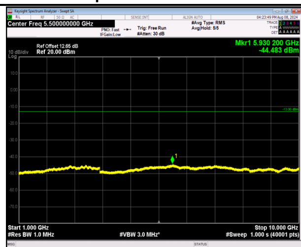
5-5-5MHz-3MHz-16QAM-16QAM-20425-20464-1RB#24- ORB#0-1000~10000MHz-PASS
