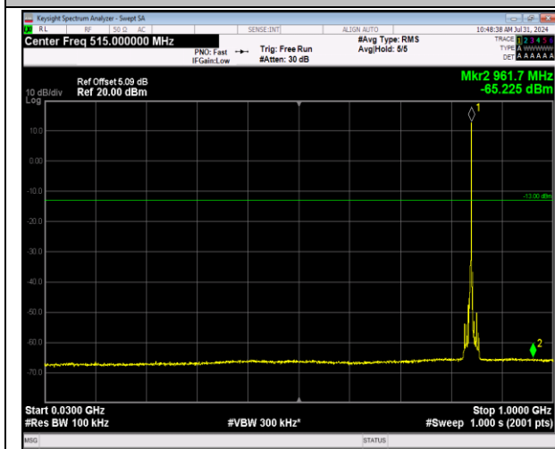
5-5-3MHz-5MHz-64QAM-64QAM-20586-20625-1RB#14- ORB#0-30~1000MHz-PASS
