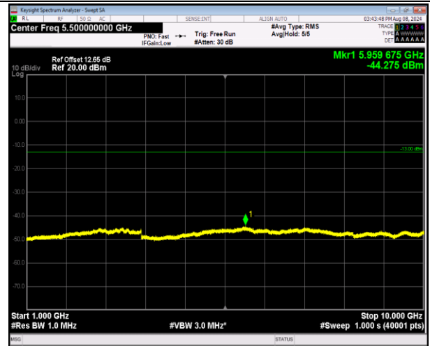
5-5-3MHz-5MHz-16QAM-16QAM-20586-20625-1RB#0-1 RB#24-1000~10000MHz-PASS
