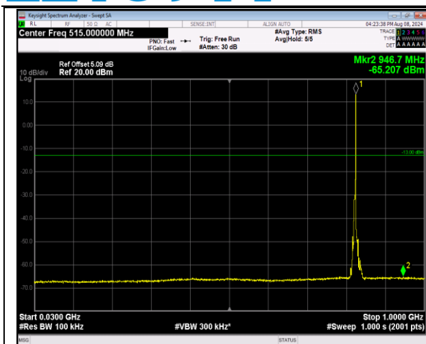
5-5-5MHz-3MHz-16QAM-16QAM-20425-20464-1RB#24- ORB#0-30~1000MHz-PASS
