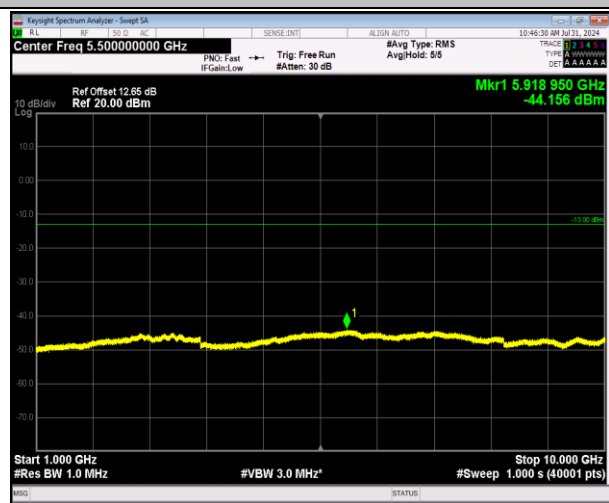
5-5-3MHz-5MHz-64QAM-64QAM-20501-20540-1RB#14- ORB#0-1000~10000MHz-PASS
