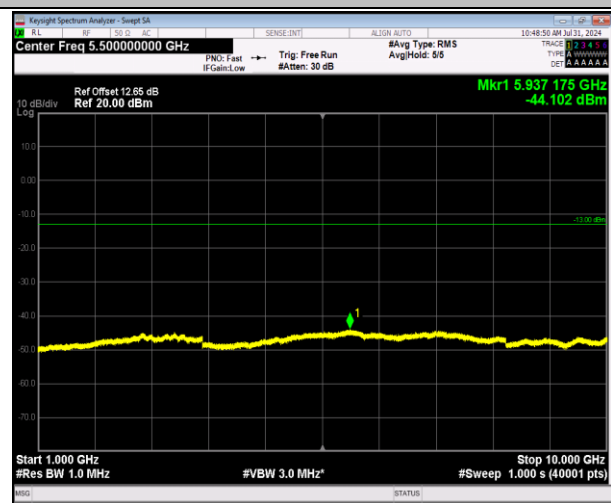
5-5-3MHz-5MHz-64QAM-64QAM-20586-20625-1RB#14- ORB#0-1000~10000MHz-PASS
