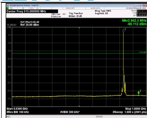
5-5-3MHz-5MHz-QPSK-QPSK-20501-20540-1RB#0-0R B#0-30~1000MHz-PASS
