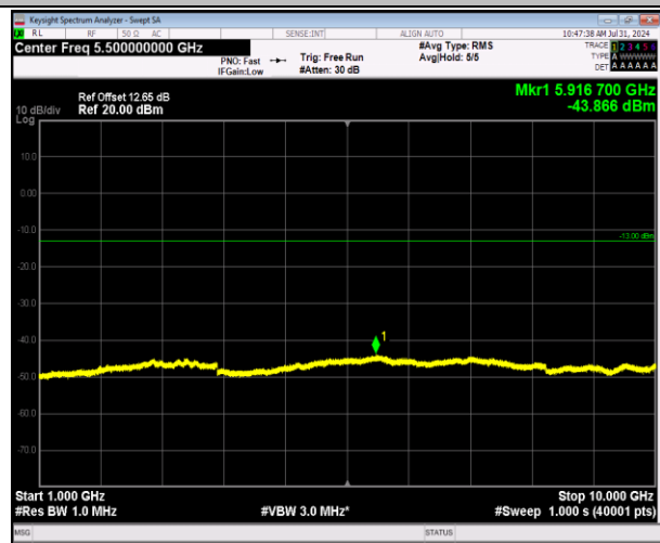
5-5-3MHz-5MHz-64QAM-64QAM-20501-20540-15RB#0- 25RB#0-1000~10000MHz-PASS
