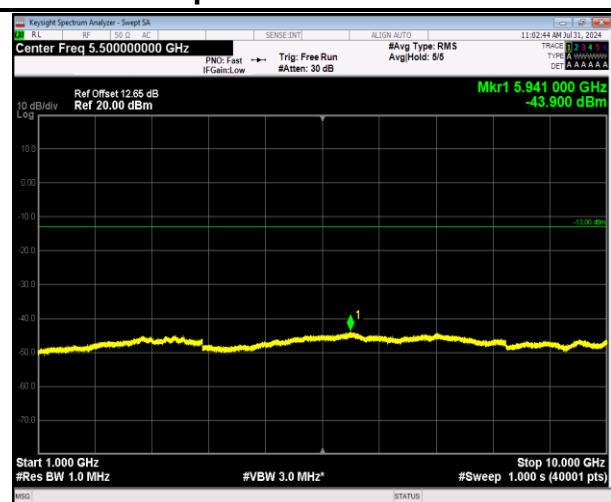
5-5-5MHz-3MHz-64QAM-64QAM-20425-20464-1RB#0-1 RB#15-1000~10000MHz-PASS
