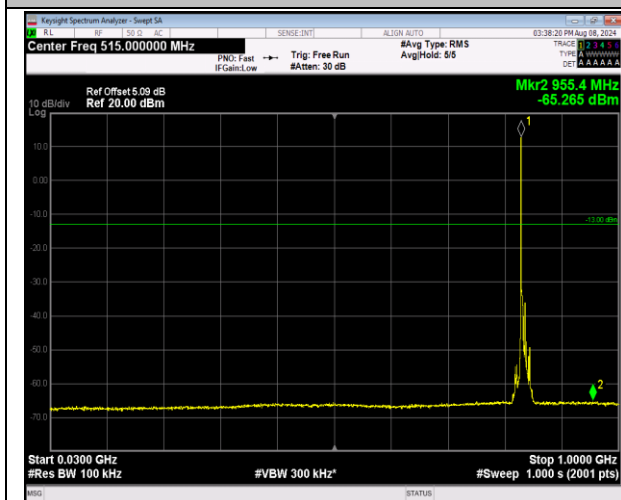
5-5-3MHz-5MHz-QPSK-QPSK-20501-20540-1RB#0-1R B#24-30~1000MHz-PASS
