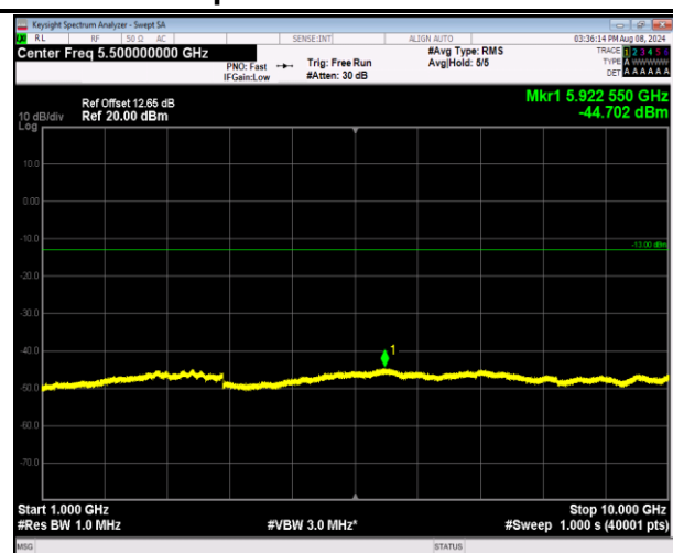
5-5-3MHz-5MHz-QPSK-QPSK-20501-20540-1RB#0-0RB #0-1000~10000MHz-PASS
