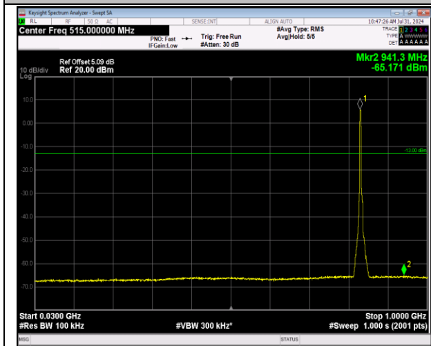
5-5-3MHz-5MHz-64QAM-64QAM-20501-20540-15RB#0- 25RB#0-30~1000MHz-PASS
