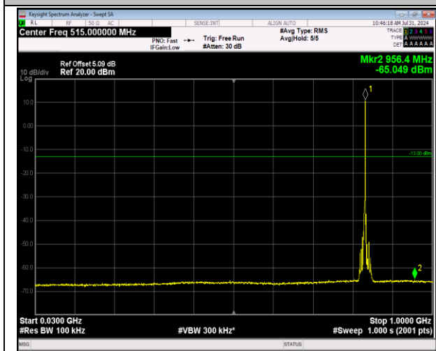
5-5-3MHz-5MHz-64QAM-64QAM-20501-20540-1RB#14- ORB#0-30~1000MHz-PASS
