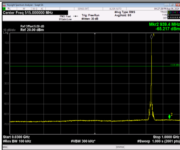
5-5-5MHz-3MHz-QPSK-QPSK-20510-20549-1RB#24-0R B#0-30~1000MHz-PASS
