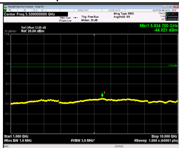
5-5-3MHz-5MHz-64QAM-64QAM-20501-20540-1RB#0-1 RB#24-1000~10000MHz-PASS
