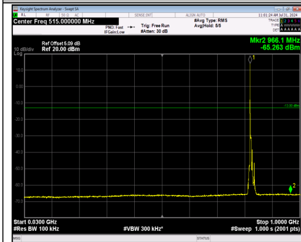
5-5-5MHz-3MHz-64QAM-64QAM-20425-20464-1RB#0-0 RB#0-30~1000MHz-PASS
