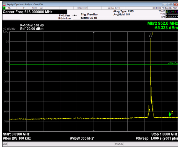
5-5-3MHz-5MHz-16QAM-16QAM-20586-20625-1RB#0-1 RB#24-30~1000MHz-PASS
