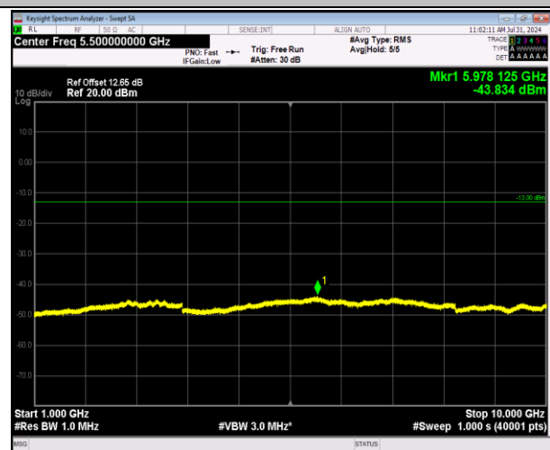
5-5-5MHz-3MHz-64QAM-64QAM-20425-20464-1RB#24- ORB#0-1000~10000MHz-PASS
