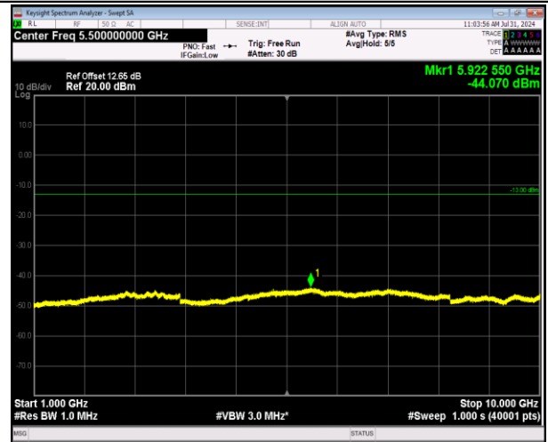
5-5-5MHz-3MHz-64QAM-64QAM-20510-20549-1RB#0-0RB#0-1000~10000MHz-PASS
