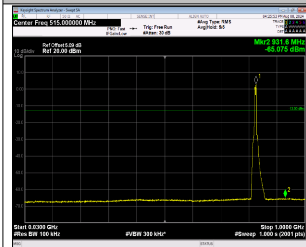
5-5-5MHz-3MHz-16QAM-16QAM-20425-20464-25RB#0- 15RB#0-30~1000MHz-PASS
