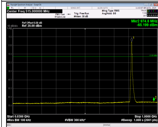
5-5-5MHz-3MHz-64QAM-64QAM-20425-20464-25RB#0- 15RB#0-30~1000MHz-PASS
