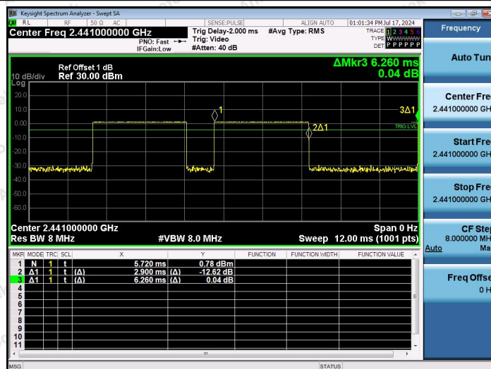
NTNV-2.4G-Ant1-2441
