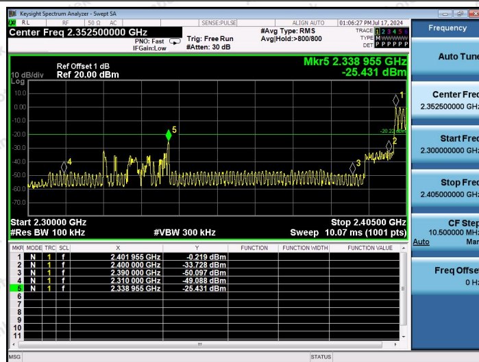
2.4G-Ant1-Hop_2402-PASS
