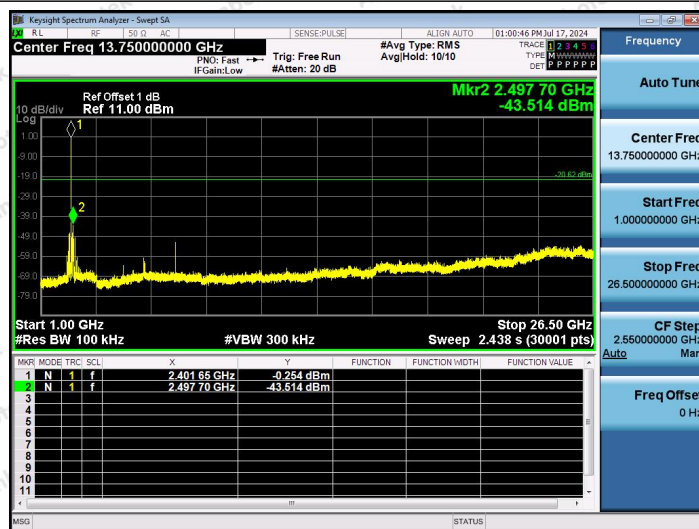
2.4G-Ant1-2402-1000~26500-PASS
