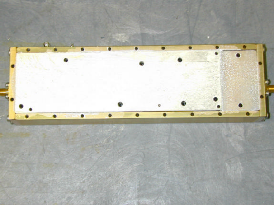
PCB Back (The PCB is heat sink. There are no traces or components)
