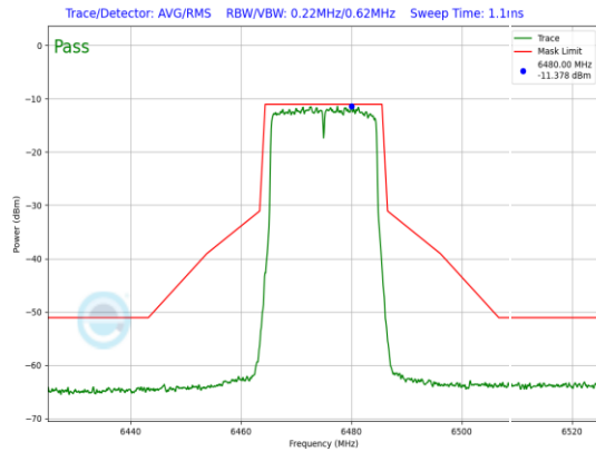
Plot 7-718. LPI In-Band Emission Plot Antenna WF5B (20MHz 802.11ax (UNII Band 6) – Ch. 105, MCS4)
