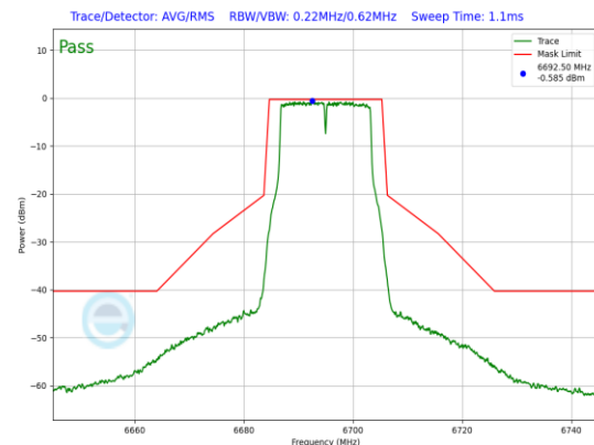
Plot 7-757. SP In-Band Emission Plot Antenna WF5B (20MHz 802.11a (UNII Band 7) – Ch. 149, 12Mbps)
