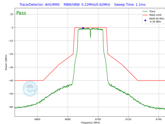
Plot 7-767. SP In-Band Emission Plot Antenna WF5B (20MHz 802.11a (UNII Band 7) – Ch. 149, 24Mbps)
