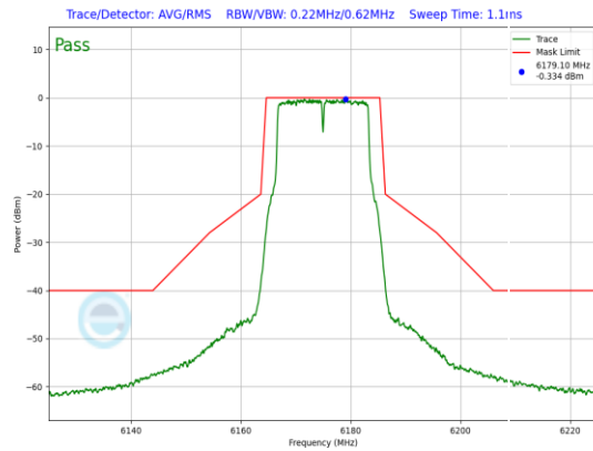
Plot 7-752. SP In-Band Emission Plot Antenna WF5B (20MHz 802.11a (UNII Band 5) – Ch. 45, 12Mbps)
