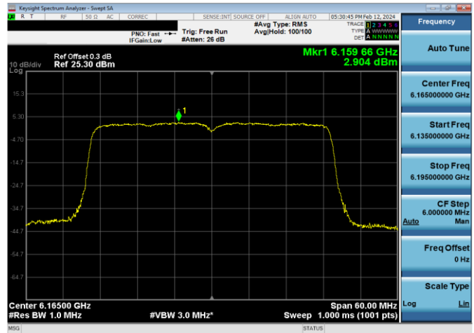
Plot 7-636. Power Spectral Density Plot SDM Diversity Antenna WF7 Standard Power (40MHz 802.11ax (UNII Band 5) – Ch. 43, MCS11)
