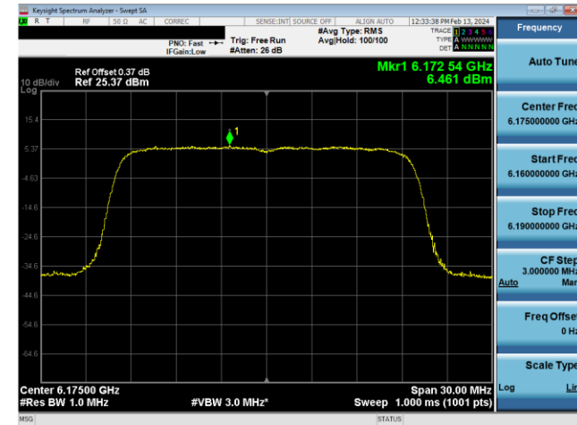
Plot 7-633. Power Spectral Density Plot SDM Diversity Antenna WF8 Standard Power (20MHz 802.11ax (UNII Band 5) – Ch. 45, MCS11)
