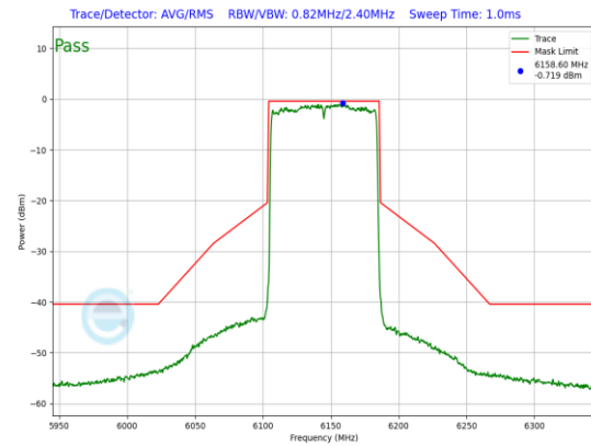
Plot 7-755. SP In-Band Emission Plot Antenna WF5B (80MHz 802.11ax (UNII Band 5) – Ch. 39, MCS2)
