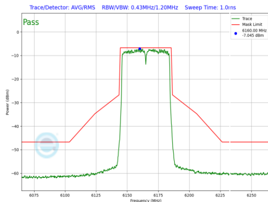
Plot 7-734. LPI In-Band Emission Plot Antenna WF5B (40MHz 802.11ax (UNII Band 5) – Ch. 43, MCS11)
