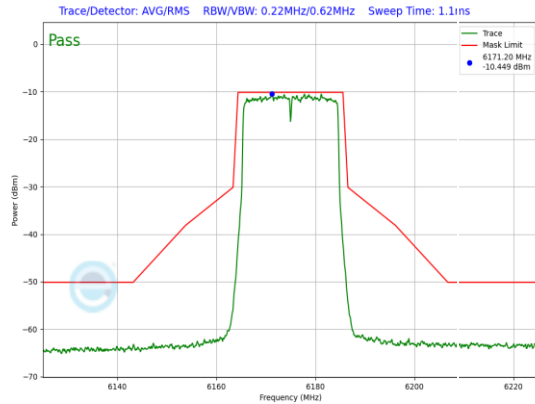
Plot 7-693. LPI In-Band Emission Plot Antenna WF5B (20MHz 802.11ax (UNII Band 5) – Ch. 45, MCS2)
