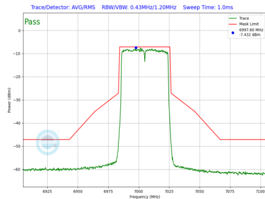
Plot 7-729. LPI In-Band Emission Plot Antenna WF5B (40MHz 802.11ax (UNII Band 8) – Ch. 211, MCS4)
