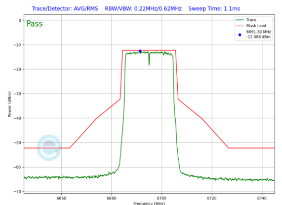
Plot 7-703. LPI In-Band Emission Plot Antenna WF5B (20MHz 802.11ax (UNII Band 7) – Ch. 149, MCS2)
