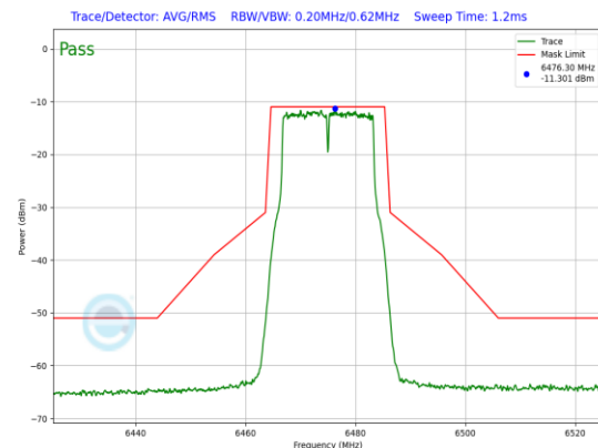
Plot 7-717. LPI In-Band Emission Plot Antenna WF5B (20MHz 802.11a (UNII Band 6) – Ch. 105, 24Mbps)
