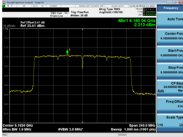
Plot 7-639. Power Spectral Density Plot SDM Diversity Antenna WF8 Standard Power (160MHz 802.11ax (UNII Band 5) – Ch. 47, MCS11)
