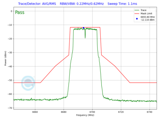
Plot 7-722. LPI In-Band Emission Plot Antenna WF5B (20MHz 802.11a (UNII Band 7) – Ch. 149, 24Mbps)
