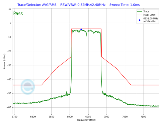
Plot 7-750. LPI In-Band Emission Plot Antenna WF5B (80MHz 802.11ax (UNII Band 8) – Ch. 199, MCS11)
