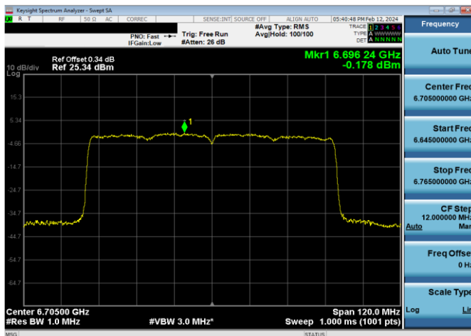
Plot 7-646. Power Spectral Density Plot SDM Diversity Antenna WF7 Standard Power (80MHz 802.11ax (UNII Band 7) – Ch. 151, MCS11)
