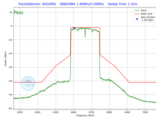
Plot 7-771. SP In-Band Emission Plot Antenna WF5B (160MHz 802.11ax (UNII Band 7) – Ch. 143, MCS4)
