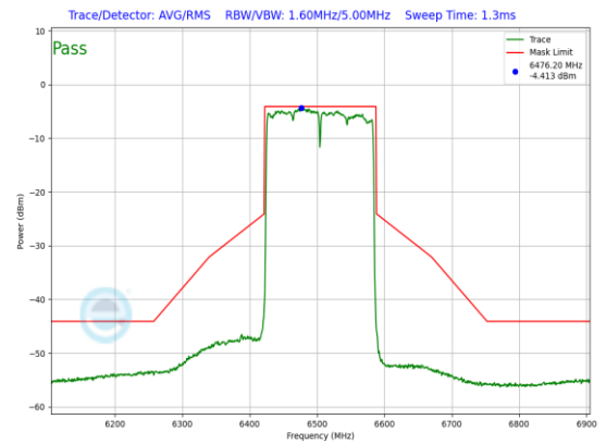
Plot 7-701. LPI In-Band Emission Plot Antenna WF5B (160MHz 802.11ax (UNII Band 6) – Ch. 111, MCS2)
