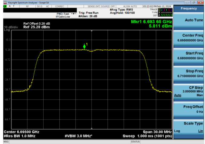
Plot 7-626. Power Spectral Density Plot SDM Diversity Antenna WF7 Standard Power (20MHz 802.11ax (UNII Band 7) – Ch. 149, MCS4)
