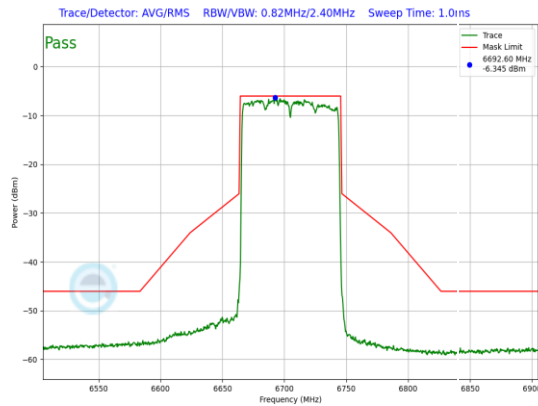
Plot 7-745. LPI In-Band Emission Plot Antenna WF5B (80MHz 802.11ax (UNII Band 7) – Ch. 151, MCS11)
