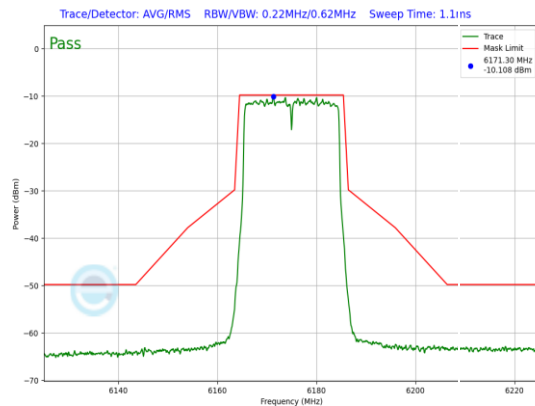
Plot 7-713. LPI In-Band Emission Plot Antenna WF5B (20MHz 802.11ax (UNII Band 5) – Ch. 45, MCS4)
