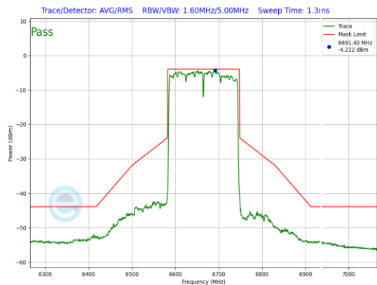
Plot 7-746. LPI In-Band Emission Plot Antenna WF5B (160MHz 802.11ax (UNII Band 7) – Ch. 143, MCS11)
