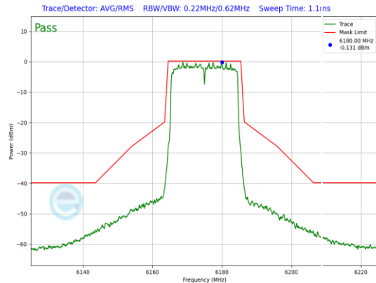
Plot 7-773. SP In-Band Emission Plot Antenna WF5B (20MHz 802.11ax (UNII Band 5) – Ch. 45, MCS11)
