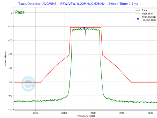
Plot 7-708. LPI In-Band Emission Plot Antenna WF5B (20MHz 802.11ax (UNII Band 8) – Ch. 209, MCS2)
