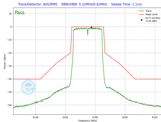
Plot 7-753. SP In-Band Emission Plot Antenna WF5B (20MHz 802.11ax (UNII Band 5) – Ch. 45, MCS2)
