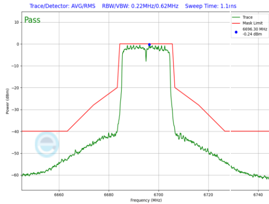
Plot 7-778. SP In-Band Emission Plot Antenna WF5B (20MHz 802.11ax (UNII Band 7) – Ch. 149, MCS11)
