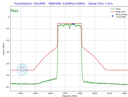
Plot 7-740. LPI In-Band Emission Plot Antenna WF5B (80MHz 802.11ax (UNII Band 6) – Ch. 103, MCS11)
