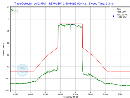
Plot 7-726. LPI In-Band Emission Plot Antenna WF5B (160MHz 802.11ax (UNII Band 7) – Ch. 143, MCS4)
