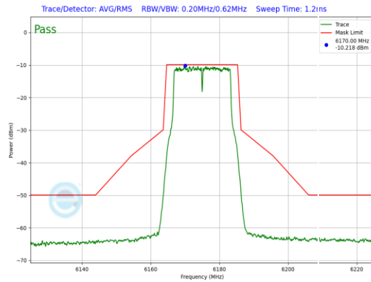
Plot 7-712. LPI In-Band Emission Plot Antenna WF5B (20MHz 802.11a (UNII Band 5) – Ch. 45, 24Mbps)
