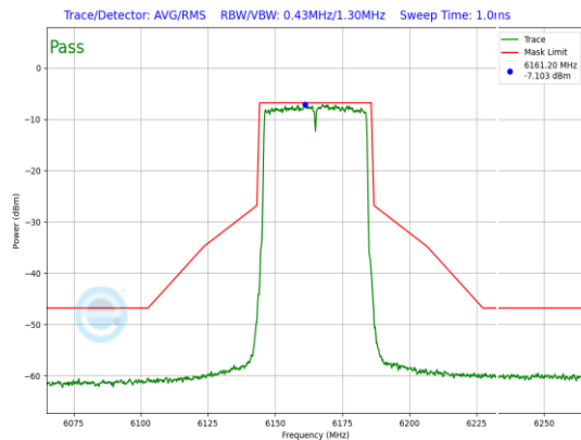
Plot 7-694. LPI In-Band Emission Plot Antenna WF5B (40MHz 802.11ax (UNII Band 5) – Ch. 43, MCS2)
