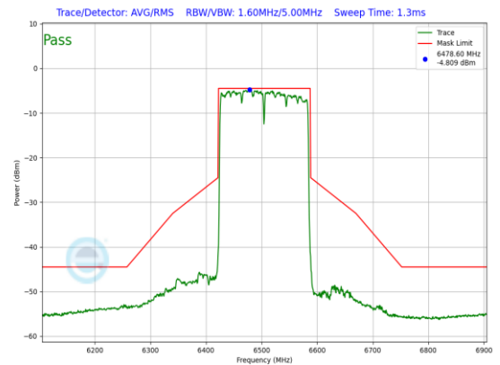
Plot 7-741. LPI In-Band Emission Plot Antenna WF5B (160MHz 802.11ax (UNII Band 6) – Ch. 111, MCS11)
