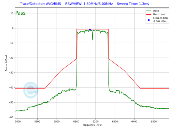
Plot 7-766. SP In-Band Emission Plot Antenna WF5B (160MHz 802.11ax (UNII Band 5) – Ch. 47, MCS4)
