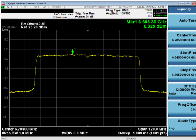
Plot 7-630. Power Spectral Density Plot SDM Diversity Antenna WF7 Standard Power (80MHz 802.11ax (UNII Band 7) – Ch. 151, MCS4)
