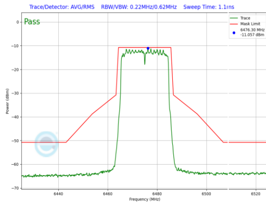
Plot 7-738. LPI In-Band Emission Plot Antenna WF5B (20MHz 802.11ax (UNII Band 6) – Ch. 105, MCS11)
