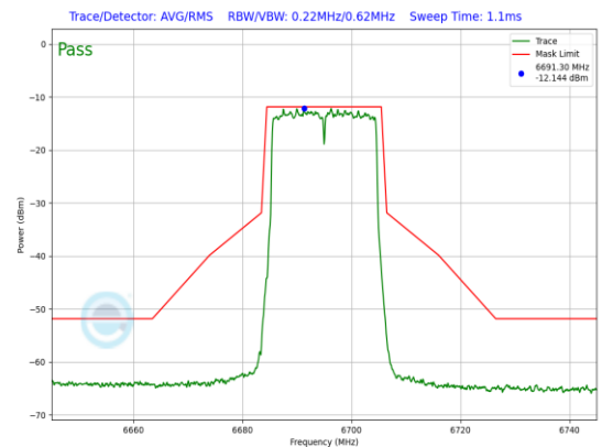
Plot 7-723. LPI In-Band Emission Plot Antenna WF5B (20MHz 802.11ax (UNII Band 7) – Ch. 149, MCS4)
