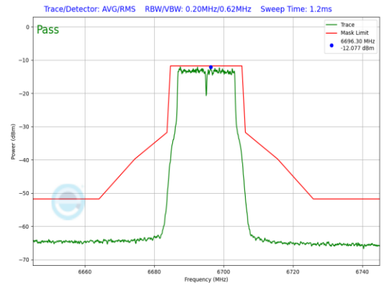
Plot 7-742. LPI In-Band Emission Plot Antenna WF5B (20MHz 802.11a (UNII Band 7) – Ch. 149, 54Mbps)
