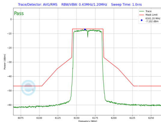
Plot 7-714. LPI In-Band Emission Plot Antenna WF5B (40MHz 802.11ax (UNII Band 5) – Ch. 43, MCS4)
