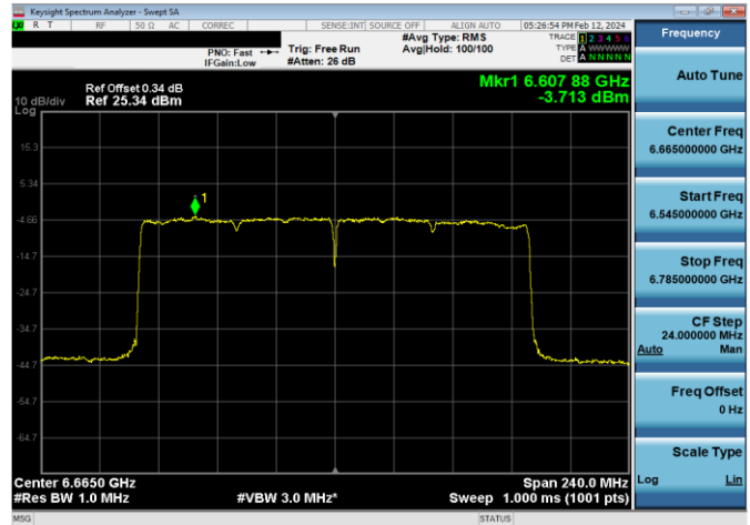
Plot 7-632. Power Spectral Density Plot SDM Diversity Antenna WF7 Standard Power (160MHz 802.11ax (UNII Band 7) – Ch. 143, MCS4)
