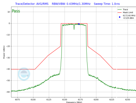
Plot 7-754. SP In-Band Emission Plot Antenna WF5B (40MHz 802.11ax (UNII Band 5) – Ch. 43, MCS2)
