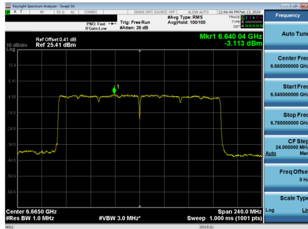
Plot 7-647. Power Spectral Density Plot SDM Diversity Antenna WF8 Standard Power (160MHz 802.11ax (UNII Band 7) – Ch. 143, MCS11)
