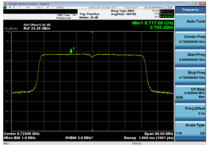
Plot 7-628. Power Spectral Density Plot SDM Diversity Antenna WF7 Standard Power (40MHz 802.11ax (UNII Band 7) – Ch. 155, MCS4)
