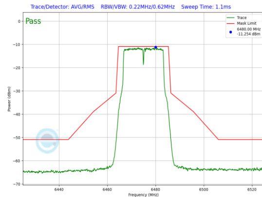
Plot 7-697. LPI In-Band Emission Plot Antenna WF5B (20MHz 802.11a (UNII Band 6) – Ch. 105, 12Mbps)
