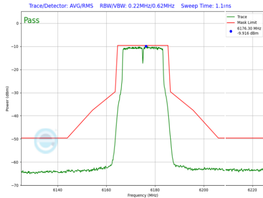
Plot 7-692. LPI In-Band Emission Plot Antenna WF5B (20MHz 802.11a (UNII Band 5) – Ch. 45, 12Mbps)
