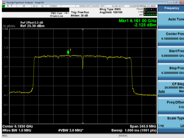
Plot 7-623. Power Spectral Density Plot SDM Diversity Antenna WF8 Standard Power (160MHz 802.11ax (UNII Band 5) – Ch. 47, MCS4)
