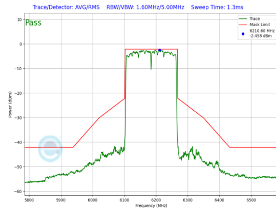
Plot 7-736. LPI In-Band Emission Plot Antenna WF5B (160MHz 802.11ax (UNII Band 5) – Ch. 47, MCS11)
