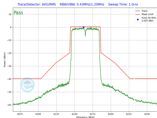
Plot 7-774. SP In-Band Emission Plot Antenna WF5B (40MHz 802.11ax (UNII Band 5) – Ch. 43, MCS11)
