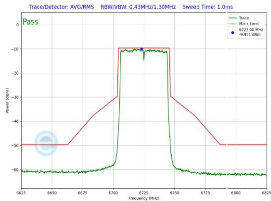
Plot 7-704. LPI In-Band Emission Plot Antenna WF5B (40MHz 802.11ax (UNII Band 7) – Ch. 155, MCS2)
