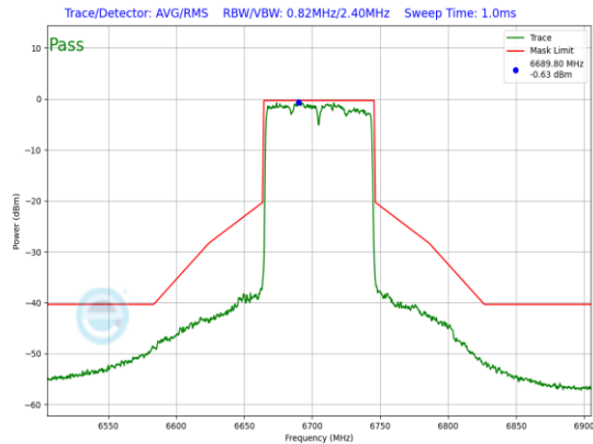
Plot 7-780. SP In-Band Emission Plot Antenna WF5B (80MHz 802.11ax (UNII Band 7) – Ch. 151, MCS11)
