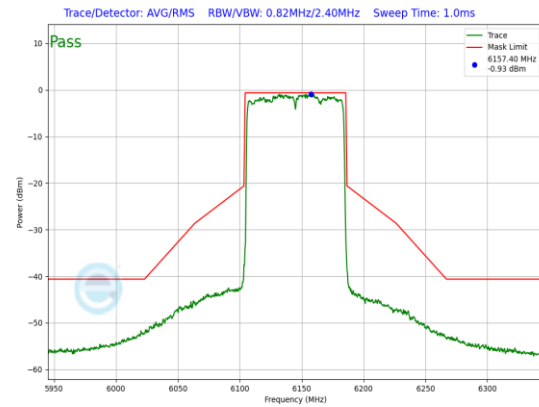
Plot 7-765. SP In-Band Emission Plot Antenna WF5B (80MHz 802.11ax (UNII Band 5) – Ch. 39, MCS4)
