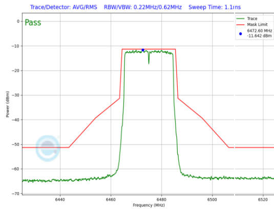
Plot 7-698. LPI In-Band Emission Plot Antenna WF5B (20MHz 802.11ax (UNII Band 6) – Ch. 105, MCS2)
