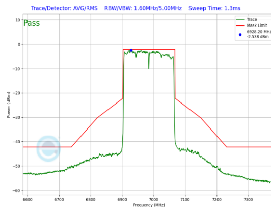
Plot 7-731. LPI In-Band Emission Plot Antenna WF5B (160MHz) 802.11ax (UNII Band 8) – Ch. 207, MCS4)
