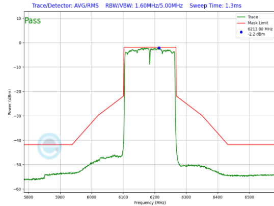
Plot 7-696. LPI In-Band Emission Plot Antenna WF5B (160MHz 802.11ax (UNII Band 5) – Ch. 47, MCS2)
