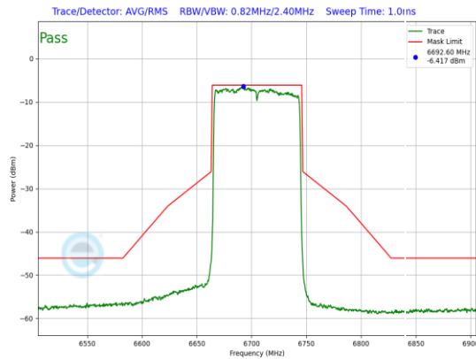
Plot 7-705. LPI In-Band Emission Plot Antenna WF5B (80MHz 802.11ax (UNII Band 7) – Ch. 151, MCS2)
