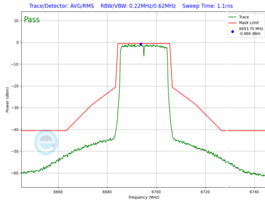
Plot 7-758. SP In-Band Emission Plot Antenna WF5B (20MHz 802.11ax (UNII Band 7) – Ch. 149, MCS2)
