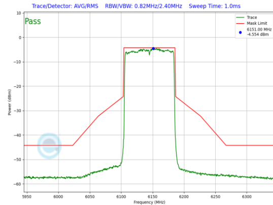
Plot 7-695. LPI In-Band Emission Plot Antenna WF5B (80MHz 802.11ax (UNII Band 5) – Ch. 39, MCS2)
