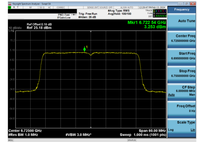
Plot 7-627. Power Spectral Density Plot SDM Diversity Antenna WF8 Standard Power (40MHz 802.11ax (UNII Band 7) – Ch. 155, MCS4)
