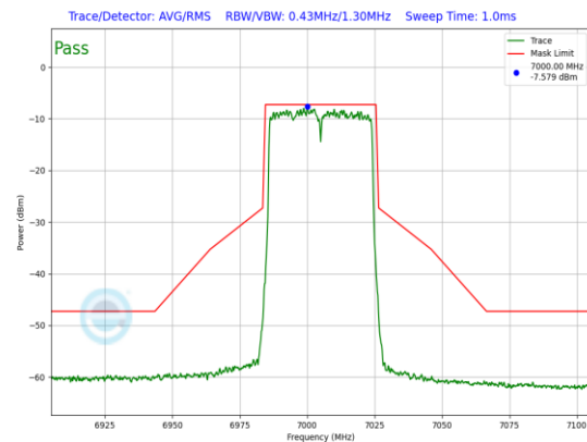
Plot 7-749. LPI In-Band Emission Plot Antenna WF5B (40MHz 802.11ax (UNII Band 8) – Ch. 211, MCS11)
