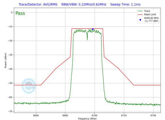
Plot 7-743. LPI In-Band Emission Plot Antenna WF5B (20MHz 802.11ax (UNII Band 7) – Ch. 149, MCS11)
