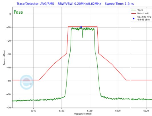
Plot 7-732. LPI In-Band Emission Plot Antenna WF5B (20MHz 802.11a (UNII Band 5) – Ch. 45, 54Mbps)
