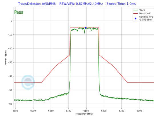
Plot 7-735. LPI In-Band Emission Plot Antenna WF5B (80MHz 802.11ax (UNII Band 5) – Ch. 39, MCS11)
