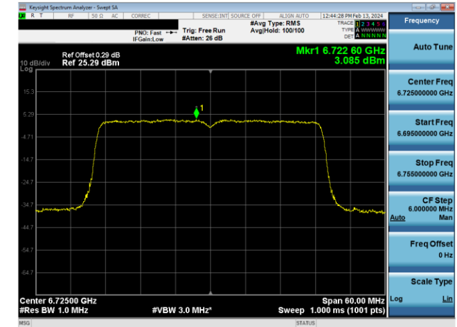
Plot 7-643. Power Spectral Density Plot SDM Diversity Antenna WF8 Standard Power (40MHz 802.11ax (UNII Band 7) – Ch. 155, MCS11)
