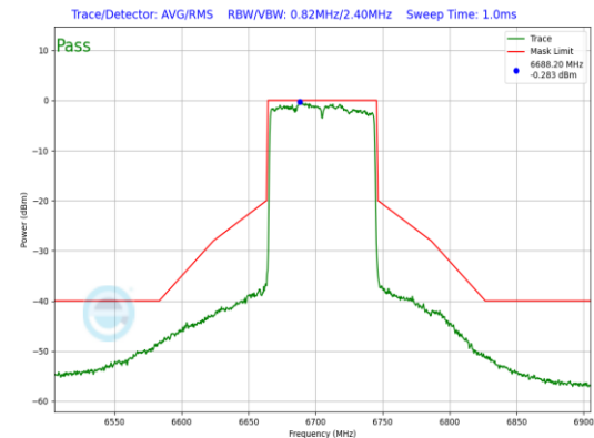
Plot 7-770. SP In-Band Emission Plot Antenna WF5B (80MHz 802.11ax (UNII Band 7) – Ch. 151, MCS4)
