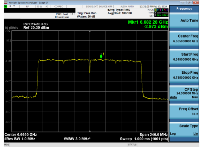
Plot 7-631. Power Spectral Density Plot SDM Diversity Antenna WF8 Standard Power (160MHz 802.11ax (UNII Band 7) – Ch. 143, MCS4)
