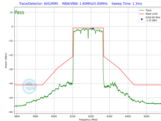
Plot 7-776. SP In-Band Emission Plot Antenna WF5B (160MHz 802.11ax (UNII Band 5) – Ch. 47, MCS11)
