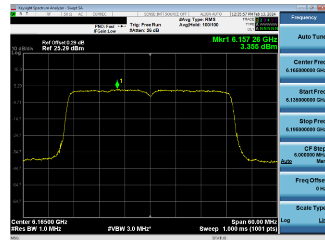
Plot 7-635. Power Spectral Density Plot SDM Diversity Antenna WF8 Standard Power (40MHz 802.11ax (UNII Band 5) – Ch. 43, MCS11)
