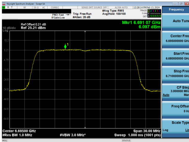
Plot 7-625. Power Spectral Density Plot SDM Diversity Antenna WF8 Standard Power (20MHz 802.11ax (UNII Band 7) – Ch. 149, MCS4)
