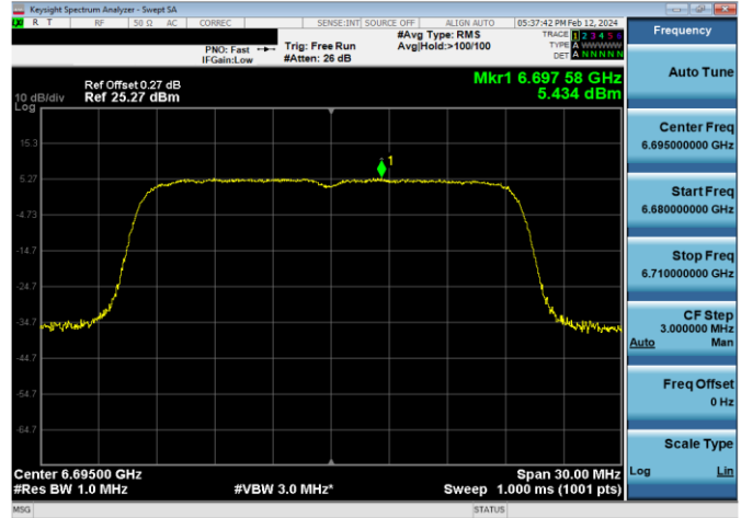
Plot 7-642. Power Spectral Density Plot SDM Diversity Antenna WF7 Standard Power (20MHz 802.11ax (UNII Band 7) – Ch. 149, MCS11)
