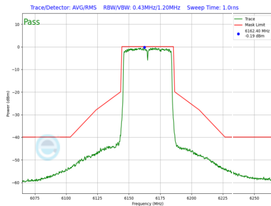
Plot 7-764. SP In-Band Emission Plot Antenna WF5B (40MHz 802.11ax (UNII Band 5) – Ch. 43, MCS4)
