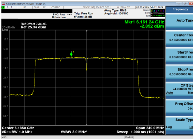
Plot 7-624. Power Spectral Density Plot SDM Diversity Antenna WF7 Standard Power (160MHz 802.11ax (UNII Band 5) – Ch. 47, MCS4)
