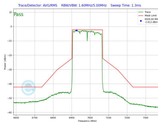
Plot 7-711. LPI In-Band Emission Plot Antenna WF5B (160MHz 802.11ax (UNII Band 8) – Ch. 207, MCS2)
