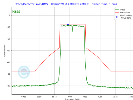
Plot 7-709. LPI In-Band Emission Plot Antenna WF5B (40MHz 802.11ax (UNII Band 8) – Ch. 211, MCS2)
