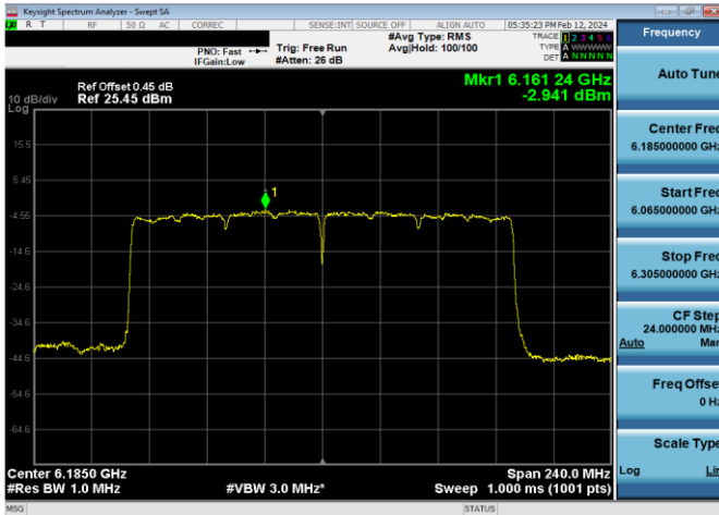
Plot 7-640. Power Spectral Density Plot SDM Diversity Antenna WF7 Standard Power (160MHz 802.11ax (UNII Band 5) – Ch. 47, MCS11)
