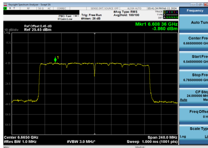
Plot 7-648. Power Spectral Density Plot SDM Diversity Antenna WF7 Standard Power (160MHz 802.11ax (UNII Band 7) – Ch. 143, MCS11)
