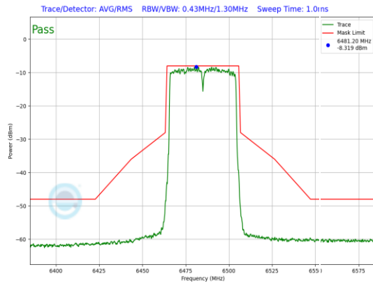
Plot 7-739. LPI In-Band Emission Plot Antenna WF5B (40MHz 802.11ax (UNII Band 6) – Ch. 107, MCS11)
