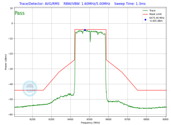
Plot 7-721. LPI In-Band Emission Plot Antenna WF5B (160MHz 802.11ax (UNII Band 6) – Ch. 111, MCS4)
