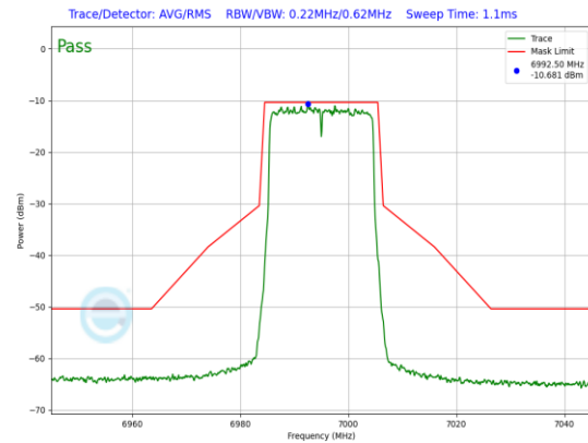
Plot 7-728. LPI In-Band Emission Plot Antenna WF5B (20MHz 802.11ax (UNII Band 8) – Ch. 209, MCS4)
