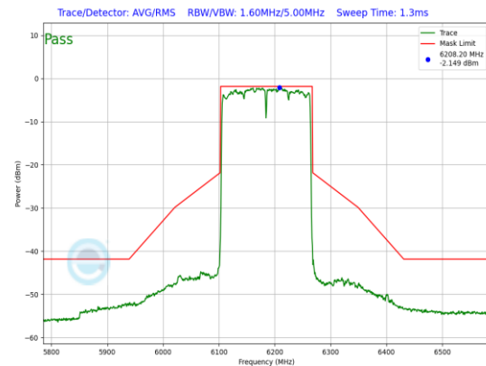
Plot 7-716. LPI In-Band Emission Plot Antenna WF5B (160MHz 802.11ax (UNII Band 5) – Ch. 47, MCS4)
