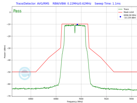
Plot 7-707. LPI In-Band Emission Plot Antenna WF5B (20MHz 802.11a (UNII Band 8) – Ch. 209, 12Mbps)
