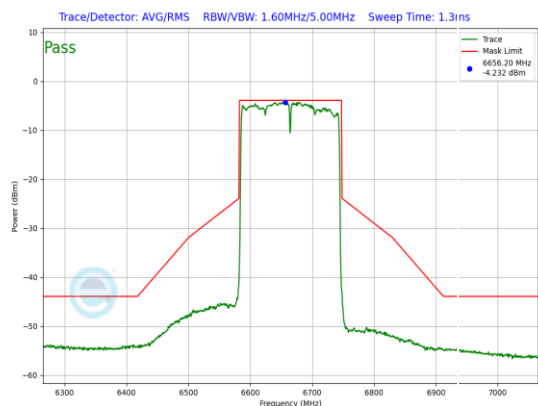
Plot 7-706. LPI In-Band Emission Plot Antenna WF5B (160MHz 802.11ax (UNII Band 7) – Ch. 143, MCS2)
