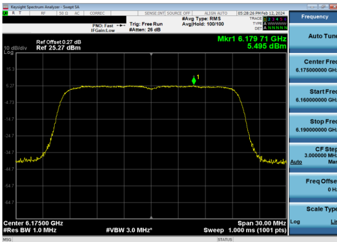
Plot 7-634. Power Spectral Density Plot SDM Diversity Antenna WF7 Standard Power (20MHz 802.11ax (UNII Band 5) – Ch. 45, MCS11)
