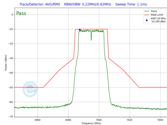
Plot 7-727. LPI In-Band Emission Plot Antenna WF5B (20MHz 802.11a (UNII Band 8) – Ch. 209, 24Mbps)
