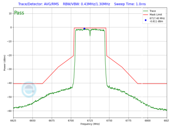
Plot 7-759. SP In-Band Emission Plot Antenna WF5B (40MHz 802.11ax (UNII Band 7) – Ch. 155, MCS2)
