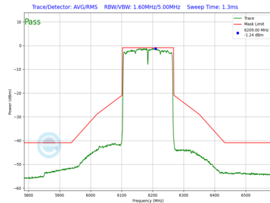
Plot 7-756. SP In-Band Emission Plot Antenna WF5B (160MHz 802.11ax (UNII Band 5) – Ch. 47, MCS2)
