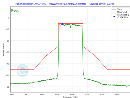
Plot 7-730. LPI In-Band Emission Plot Antenna WF5B (80MHz) 802.11ax (UNII Band 8) – Ch. 199, MCS4)
