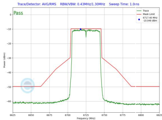
Plot 7-724. LPI In-Band Emission Plot Antenna WF5B (40MHz 802.11ax (UNII Band 7) – Ch. 155, MCS4)
