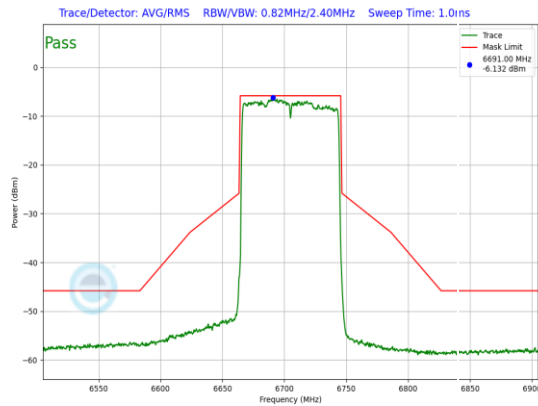
Plot 7-725. LPI In-Band Emission Plot Antenna WF5B (80MHz 802.11ax (UNII Band 7) – Ch. 151, MCS4)
