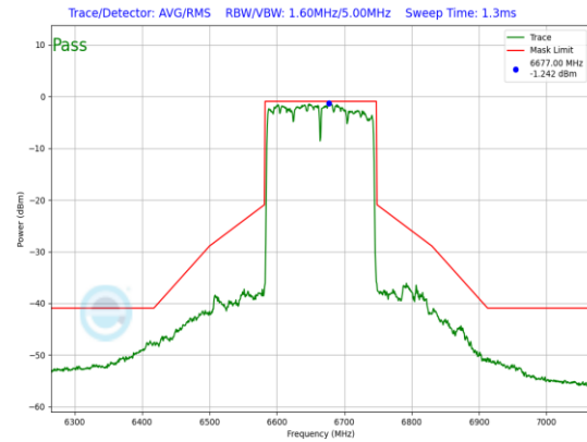
Plot 7-781. SP In-Band Emission Plot Antenna WF5B (160MHz 802.11ax (UNII Band 7) – Ch. 143, MCS11)
