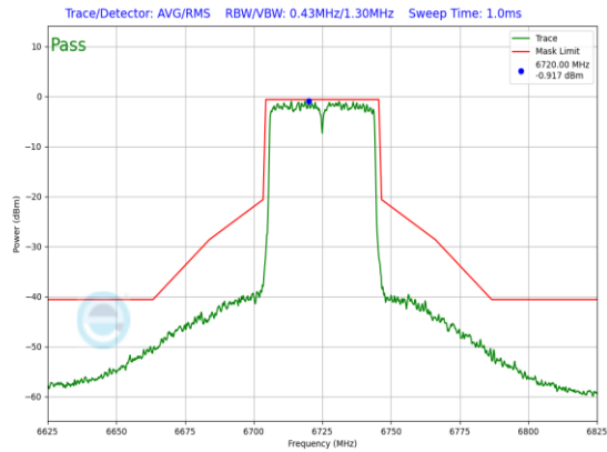
Plot 7-779. SP In-Band Emission Plot Antenna WF5B (40MHz 802.11ax (UNII Band 7) – Ch. 155, MCS11)
