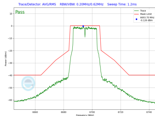
Plot 7-777. SP In-Band Emission Plot Antenna WF5B (20MHz 802.11a (UNII Band 7) – Ch. 149, 54Mbps)
