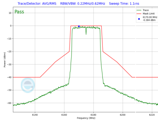
Plot 7-763. SP In-Band Emission Plot Antenna WF5B (20MHz 802.11ax (UNII Band 5) – Ch. 45, MCS4)
