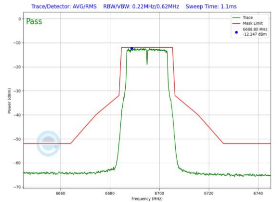
Plot 7-702. LPI In-Band Emission Plot Antenna WF5B (20MHz 802.11a (UNII Band 7) – Ch. 149, 12Mbps)
