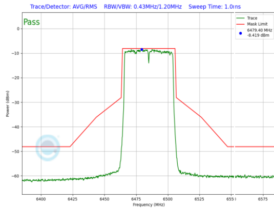
Plot 7-719. LPI In-Band Emission Plot Antenna WF5B (40MHz 802.11ax (UNII Band 6) – Ch. 107, MCS4)
