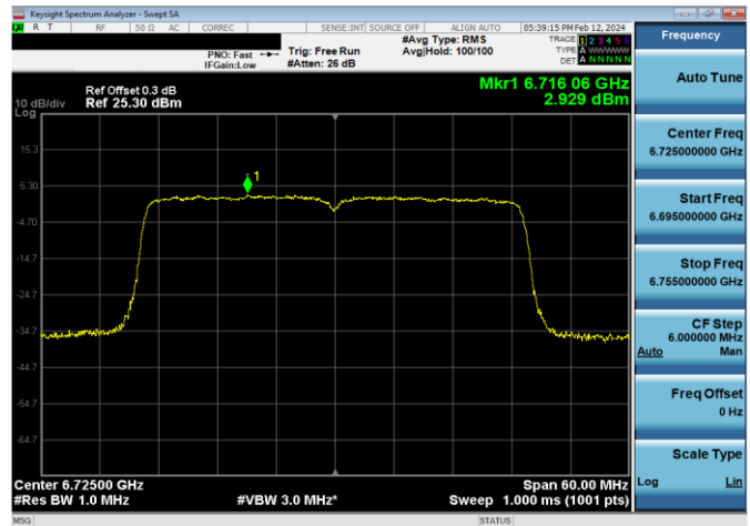
Plot 7-644. Power Spectral Density Plot SDM Diversity Antenna WF7 Standard Power (40MHz 802.11ax (UNII Band 7) – Ch. 155, MCS11)
