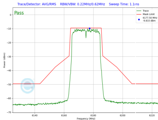
Plot 7-733. LPI In-Band Emission Plot Antenna WF5B (20MHz 802.11ax (UNII Band 5) – Ch. 45, MCS11)
