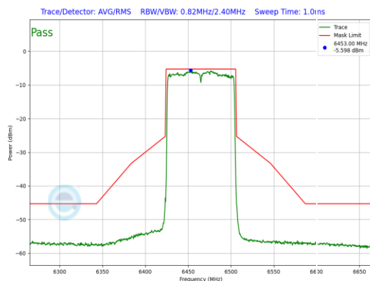
Plot 7-700. LPI In-Band Emission Plot Antenna WF5B (80MHz 802.11ax (UNII Band 6) – Ch. 103, MCS2)
