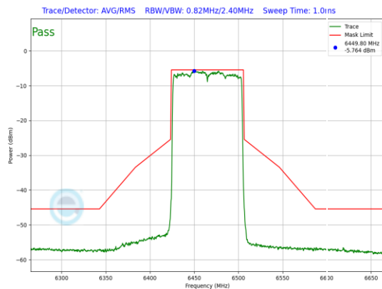
Plot 7-720. LPI In-Band Emission Plot Antenna WF5B (80MHz 802.11ax (UNII Band 6) – Ch. 103, MCS4)
