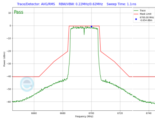
Plot 7-768. SP In-Band Emission Plot Antenna WF5B (20MHz 802.11ax (UNII Band 7) – Ch. 149, MCS4)
