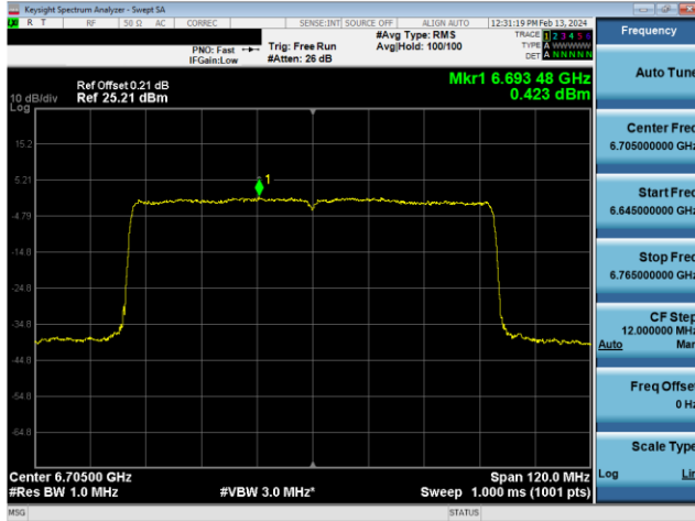
Plot 7-629. Power Spectral Density Plot SDM Diversity Antenna WF8 Standard Power (80MHz 802.11ax (UNII Band 7) – Ch. 151, MCS4)
