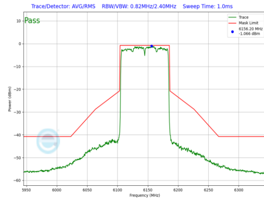
Plot 7-775. SP In-Band Emission Plot Antenna WF5B (80MHz 802.11ax (UNII Band 5) – Ch. 39, MCS11)
