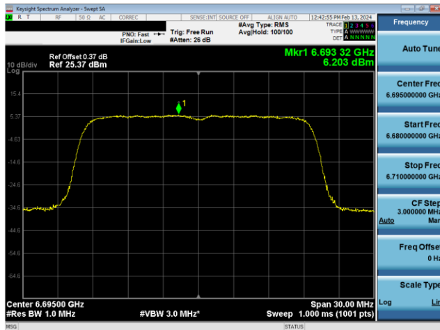
Plot 7-641. Power Spectral Density Plot SDM Diversity Antenna WF8 Standard Power (20MHz 802.11ax (UNII Band 7) – Ch. 149, MCS11)
