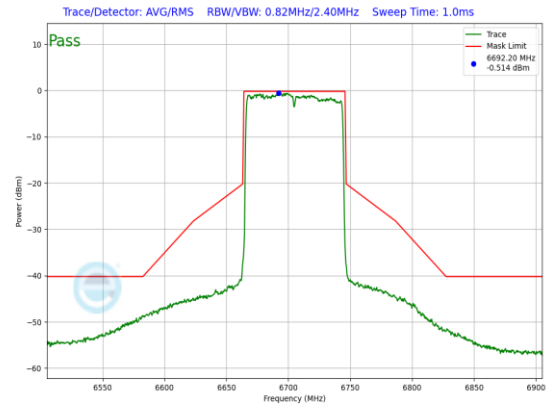
Plot 7-760. SP In-Band Emission Plot Antenna WF5B (80MHz 802.11ax (UNII Band 7) – Ch. 151, MCS2)
