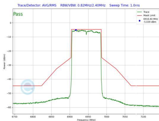
Plot 7-710. LPI In-Band Emission Plot Antenna WF5B (80MHz 802.11ax (UNII Band 8) – Ch. 199, MCS2)
