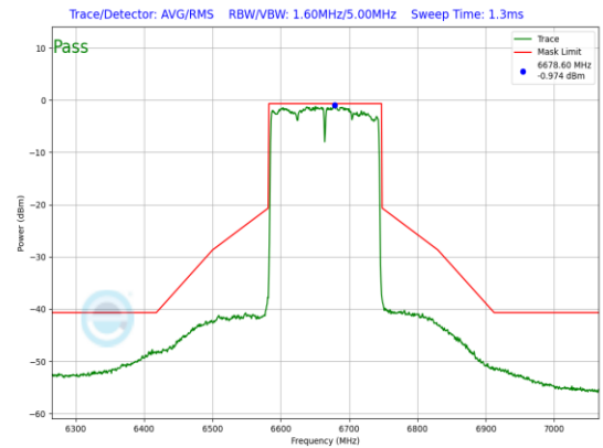
Plot 7-761. SP In-Band Emission Plot Antenna WF5B (160MHz 802.11ax (UNII Band 7) – Ch. 143, MCS2)
