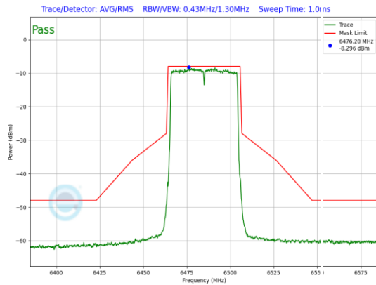
Plot 7-699. LPI In-Band Emission Plot Antenna WF5B (40MHz 802.11ax (UNII Band 6) – Ch. 107, MCS2)
