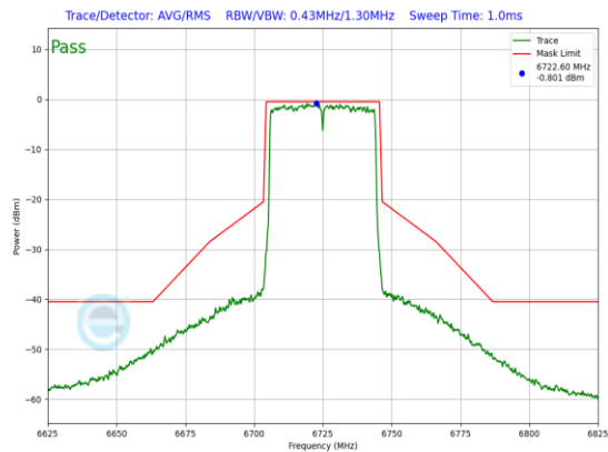
Plot 7-769. SP In-Band Emission Plot Antenna WF5B (40MHz 802.11ax (UNII Band 7) – Ch. 155, MCS4)
