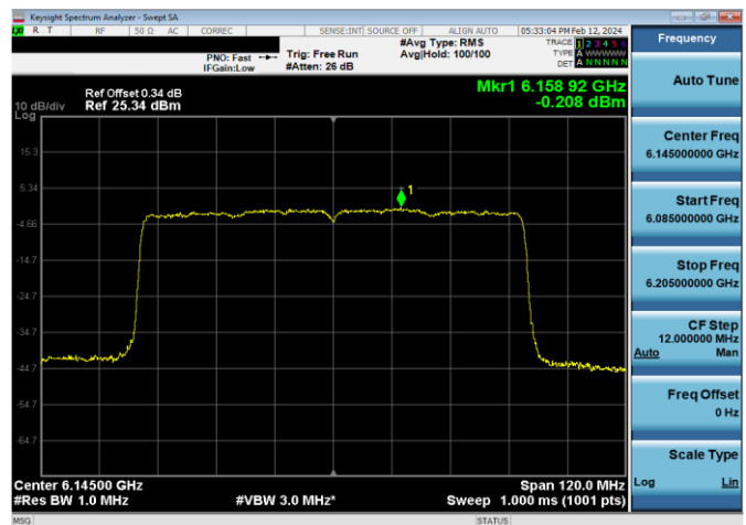
Plot 7-638. Power Spectral Density Plot SDM Diversity Antenna WF7 Standard Power (80MHz 802.11ax (UNII Band 5) – Ch. 39, MCS11)
