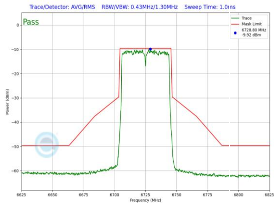
Plot 7-744. LPI In-Band Emission Plot Antenna WF5B (40MHz 802.11ax (UNII Band 7) – Ch. 155, MCS11)
