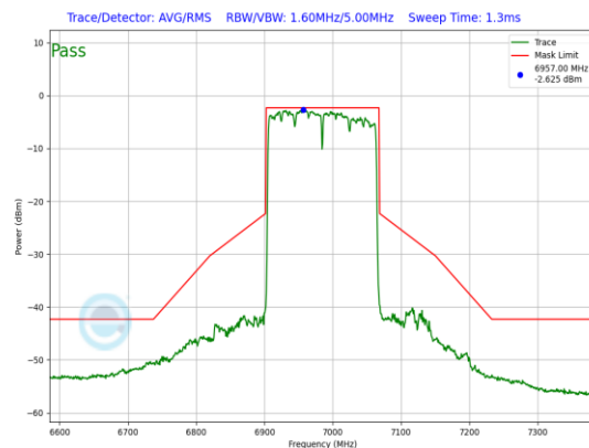
Plot 7-751. LPI In-Band Emission Plot Antenna WF5B (160MHz 802.11ax (UNII Band 8) – Ch. 207, MCS11)
