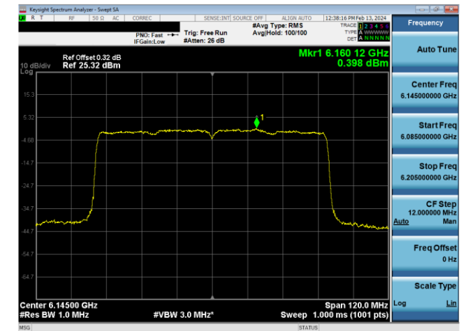
Plot 7-637. Power Spectral Density Plot SDM Diversity Antenna WF8 Standard Power (80MHz 802.11ax (UNII Band 5) – Ch. 39, MCS11)
