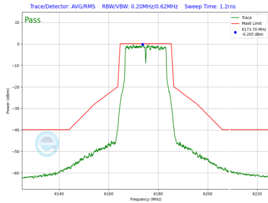
Plot 7-772. SP In-Band Emission Plot Antenna WF5B (20MHz 802.11a (UNII Band 5) – Ch. 45, 54Mbps)
