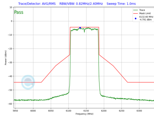
Plot 7-715. LPI In-Band Emission Plot Antenna WF5B (80MHz 802.11ax (UNII Band 5) – Ch. 39, MCS4)
