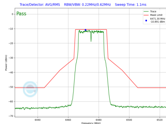
Plot 7-737. LPI In-Band Emission Plot Antenna WF5B (20MHz 802.11a (UNII Band 6) – Ch. 105, 54Mbps)
