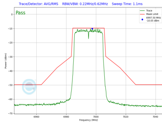
Plot 7-748. LPI In-Band Emission Plot Antenna WF5B (20MHz 802.11ax (UNII Band 8) – Ch. 209, MCS11)
