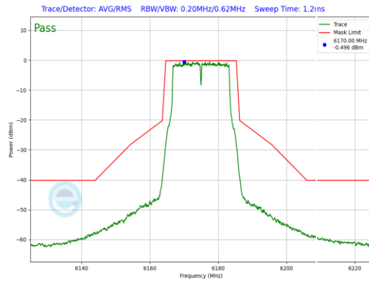
Plot 7-762. SP In-Band Emission Plot Antenna WF5B (20MHz 802.11a (UNII Band 5) – Ch. 45, 24Mbps)
