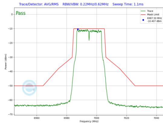
Plot 7-747. LPI In-Band Emission Plot Antenna WF5B (20MHz 802.11a (UNII Band 8) – Ch. 209, 54Mbps)
