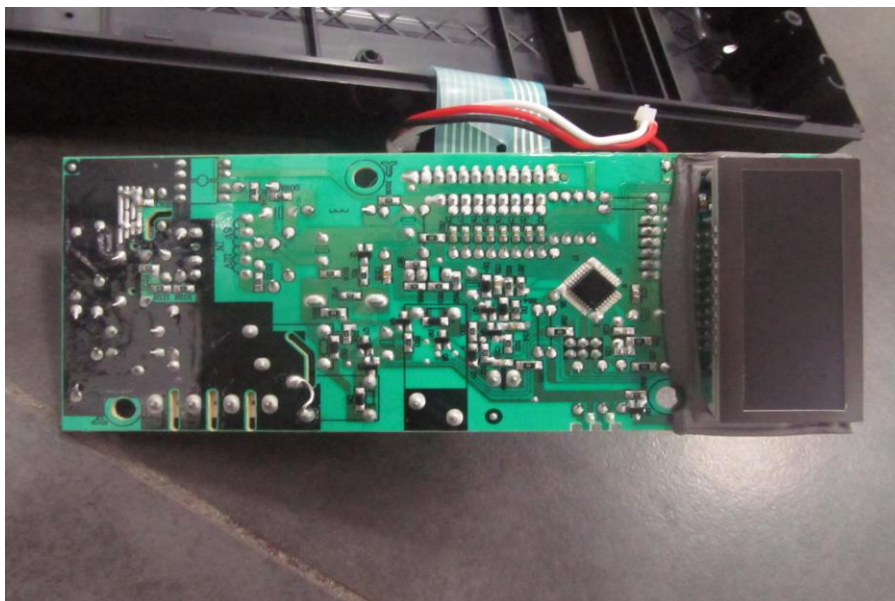
Power board - Top View
