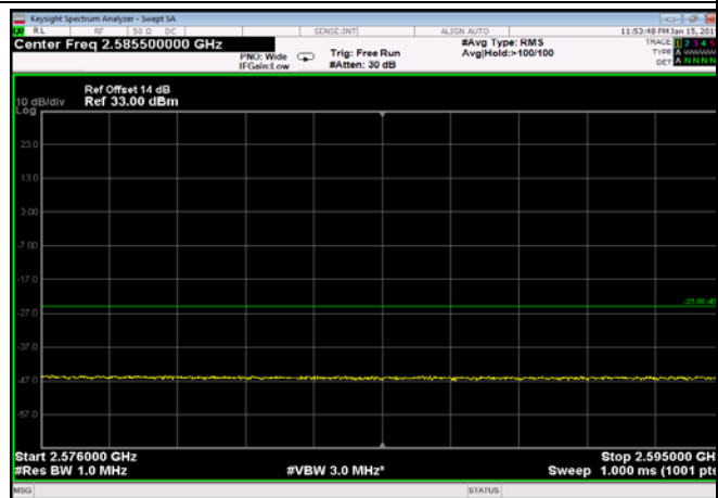
HighRange_FDD07_5MHz_2567.5_OneRB _high_Q16
