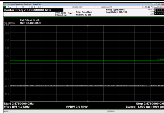
HighRange_FDD07_5MHz_2567.5_OneRB _high_QPSK
