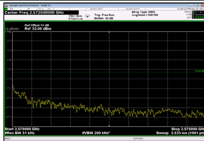
FDD07_5MHz_2567.5_Q16_OneRB_high
