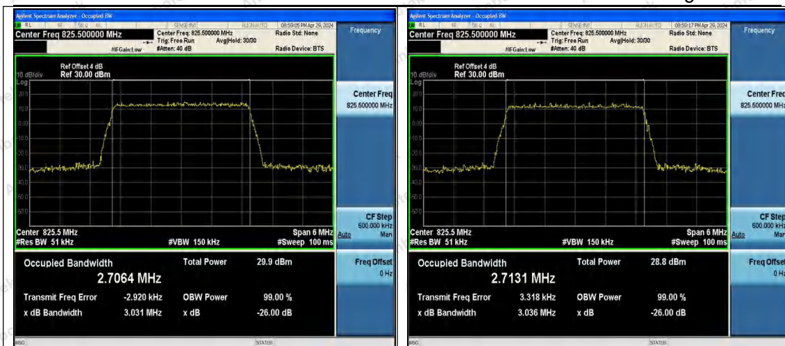
Band5-3MHz-16QAM-20415-15RB#0-PASS
