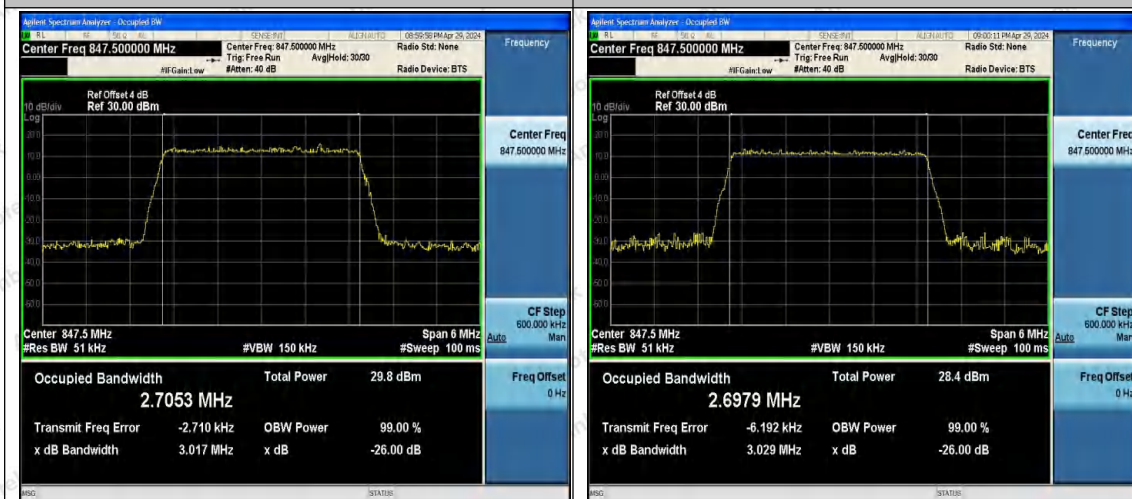
Band5-3MHz-16QAM-20635-15RB#0-PASS
