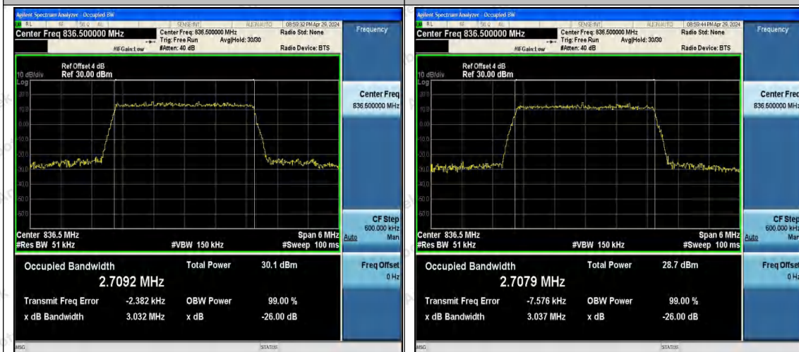
Band5-3MHz-16QAM-20525-15RB#0-PASS
