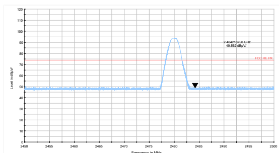
DH5-Channel 78: Peak
