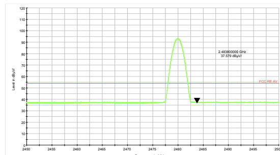
DH5-Channel 78: Average
