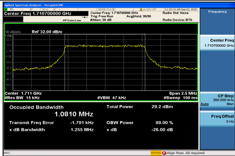
Band4-1.4MHz-QPSK-19957-6RB#0-1.0810
