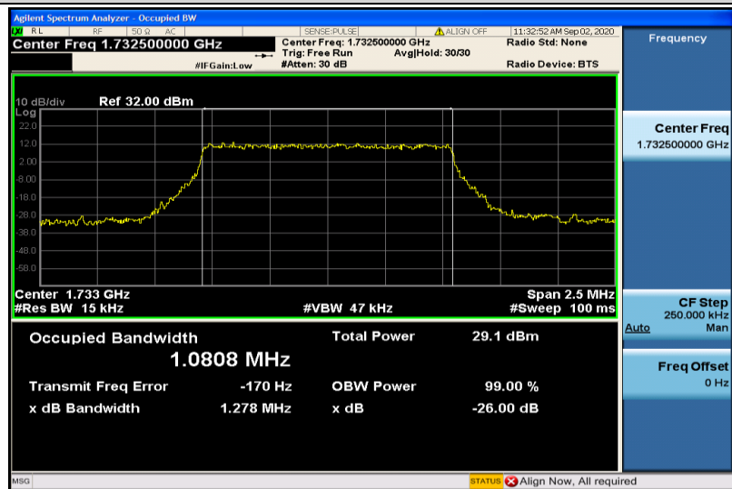
Band4-1.4MHz-QPSK-20175-6RB#0-1.0808
