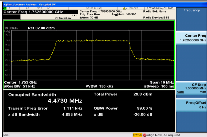
Band4-5MHz-16QAM-20375-25RB#0-4.4730
