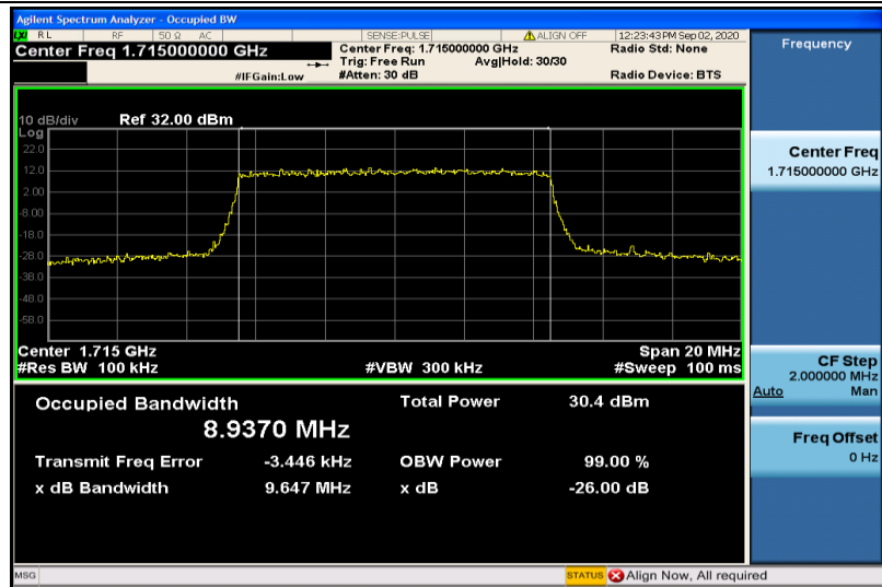
Band4-10MHz-QPSK-20000-50RB#0-8.9370
