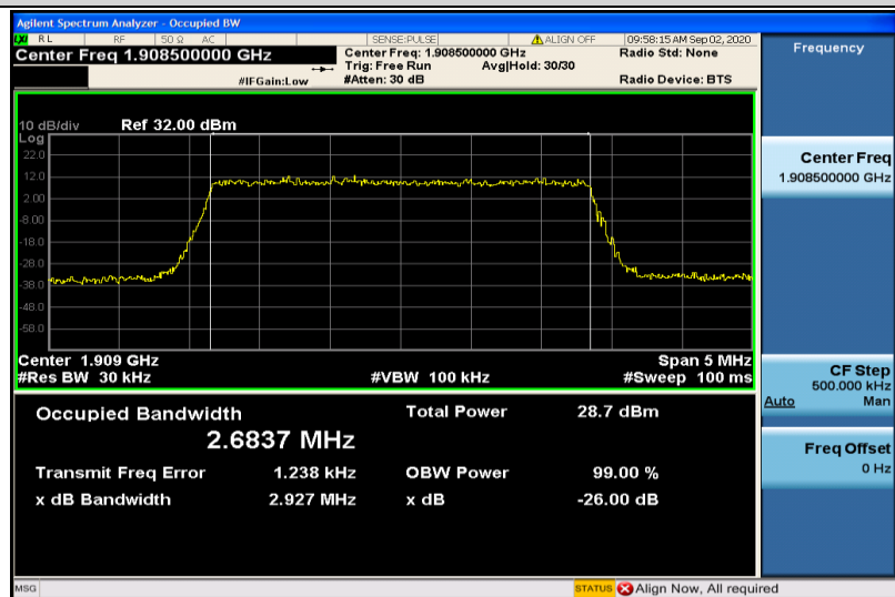
Band2-3MHz-16QAM-19185-15RB#0-2.6837
