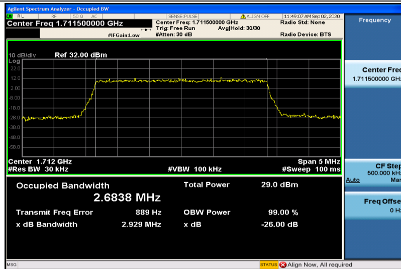
Band4-3MHz-16QAM-19965-15RB#0-2.6838
