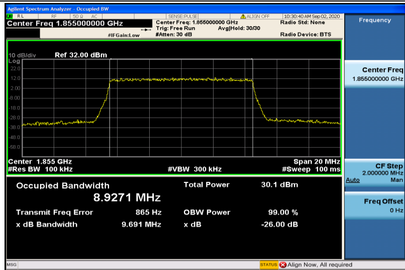
Band2-10MHz-16QAM-18650-50RB#0-8.9271
