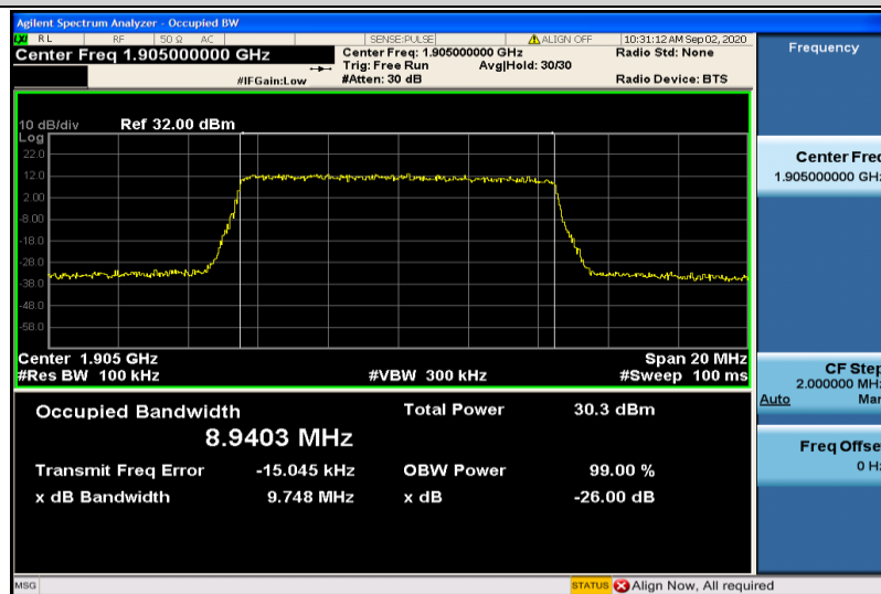
Band2-10MHz-QPSK-19150-50RB#0-8.9403
