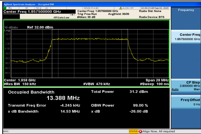
Band2-15MHz-QPSK-18675-75RB#0-13.388
