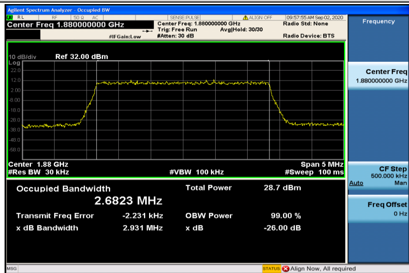
Band2-3MHz-16QAM-18900-15RB#0-2.6823
