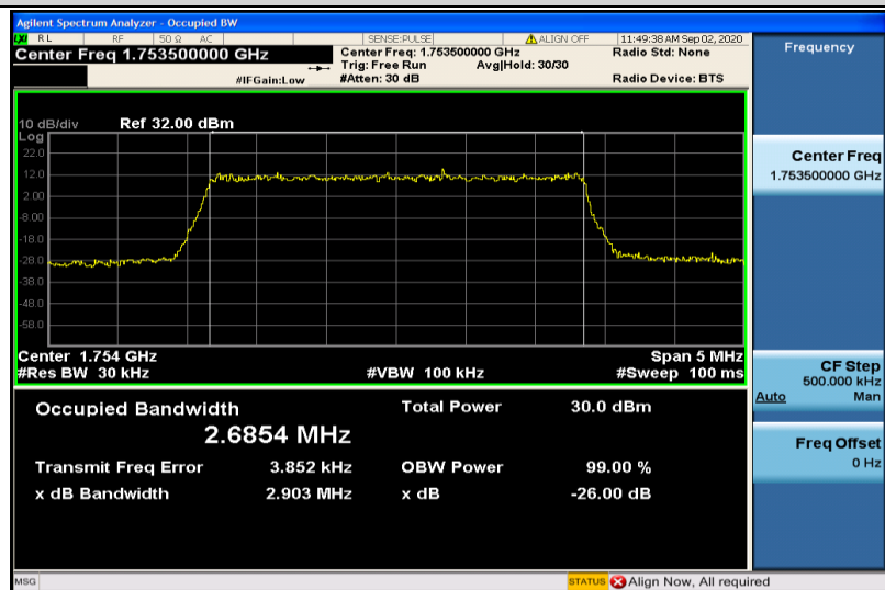
Band4-3MHz-QPSK-20385-15RB#0-2.6854
