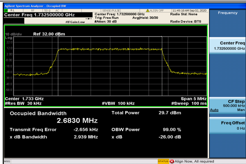
Band4-3MHz-QPSK-20175-15RB#0-2.6830
