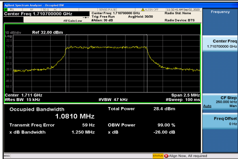
Band4-1.4MHz-16QAM-19957-6RB#0-1.0810
