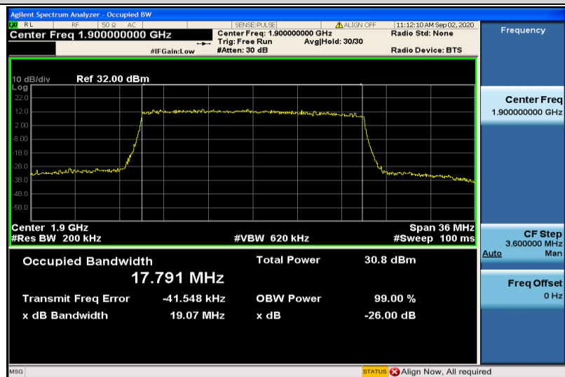
Band2-20MHz-QPSK-19100-100RB#0-17.791
