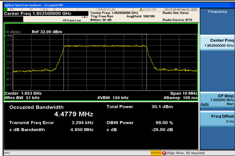
Band2-5MHz-16QAM-18625-25RB#0-4.4779
