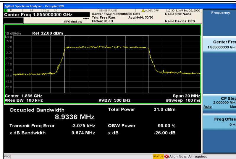
Band2-10MHz-QPSK-18650-50RB#0-8.9336
