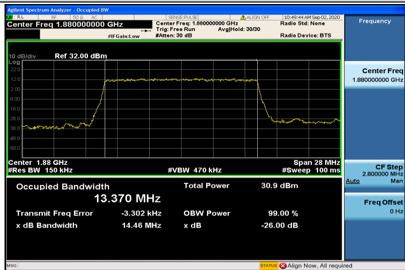
Band2-15MHz-QPSK-18900-75RB#0-13.370
