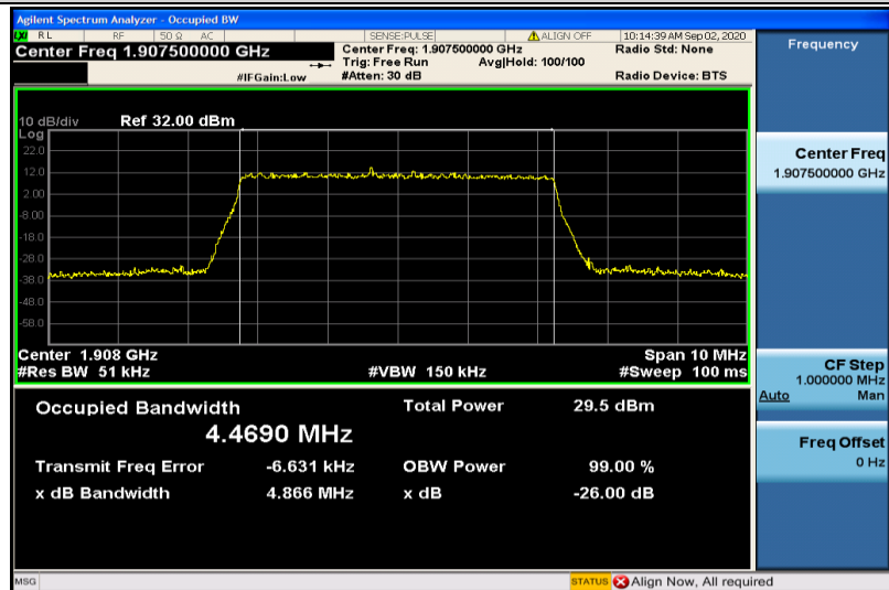
Band2-5MHz-16QAM-19175-25RB#0-4.4690
