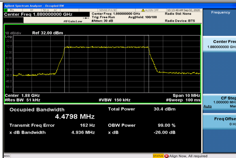
Band2-5MHz-QPSK-18900-25RB#0-4.4798
