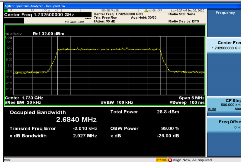
Band4-3MHz-16QAM-20175-15RB#0-2.6840
