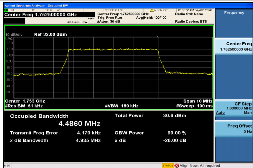
Band4-5MHz-QPSK-20375-25RB#0-4.4860
