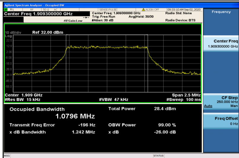
Band2-1.4MHz-16QAM-19193-6RB#0-1.0796
