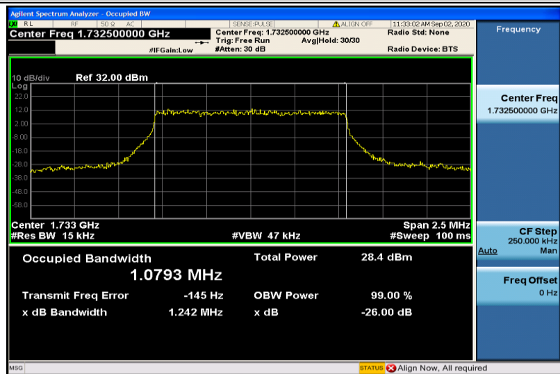
Band4-1.4MHz-16QAM-20175-6RB#0-1.0793
