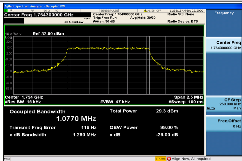
Band4-1.4MHz-QPSK-20393-6RB#0-1.0770
