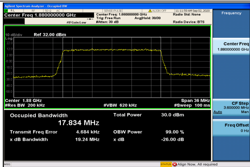
Band2-20MHz-16QAM-18900-100RB#0-17.834
