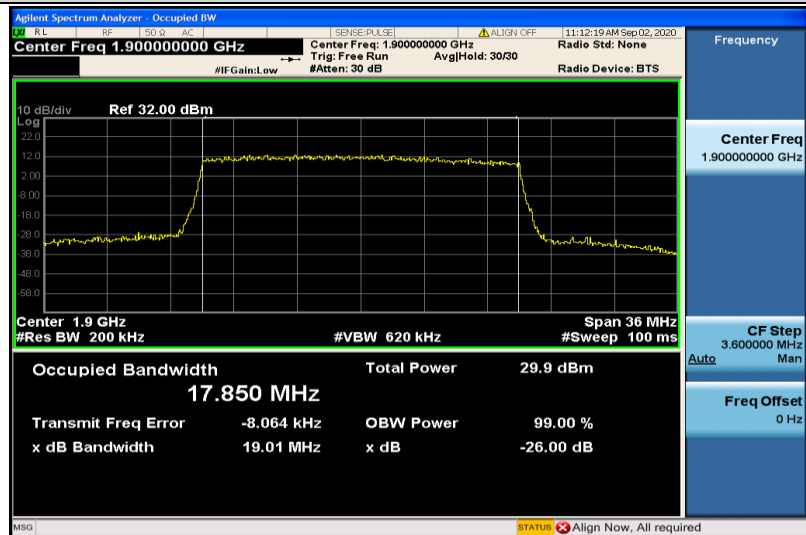
Band2-20MHz-16QAM-19100-100RB#0-17.850
