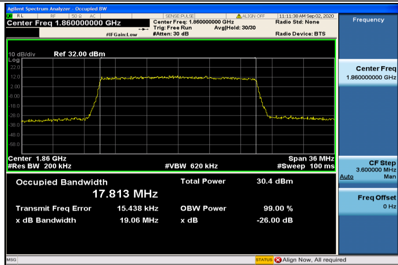
Band2-20MHz-16QAM-18700-100RB#0-17.813
