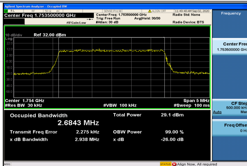
Band4-3MHz-16QAM-20385-15RB#0-2.6843
