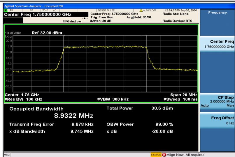
Band4-10MHz-QPSK-20350-50RB#0-8.9322
