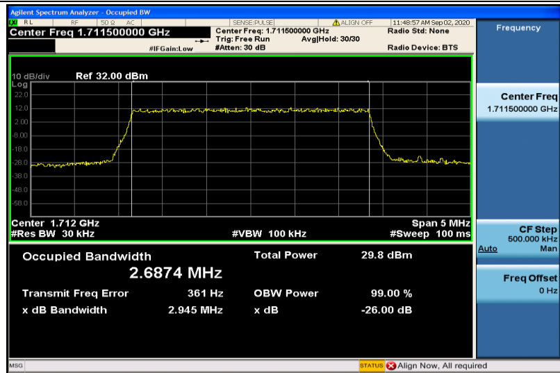
Band4-3MHz-QPSK-19965-15RB#0-2.6874
