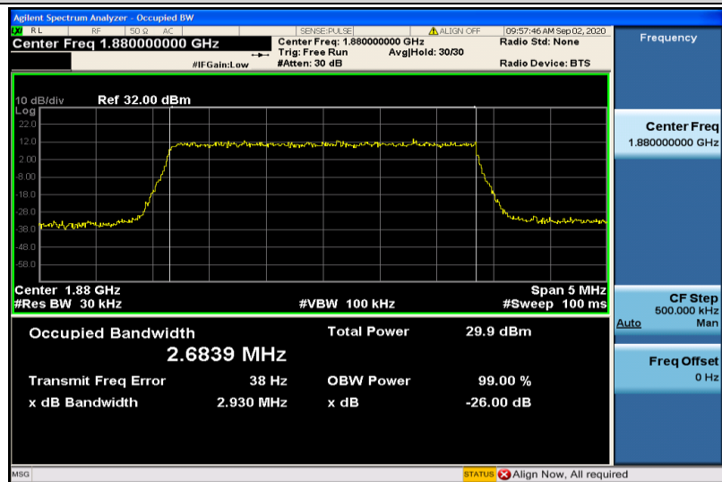
Band2-3MHz-QPSK-18900-15RB#0-2.6839
