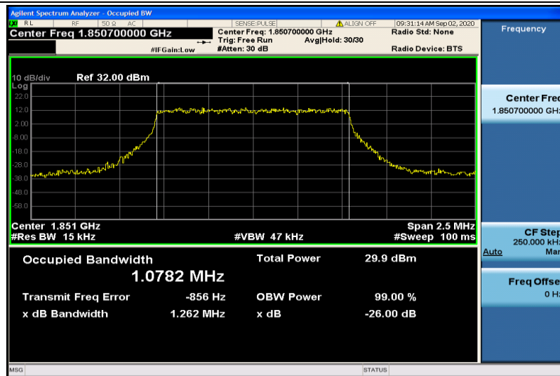
Band2-1.4MHz-QPSK-18607-6RB#0-1.0782
