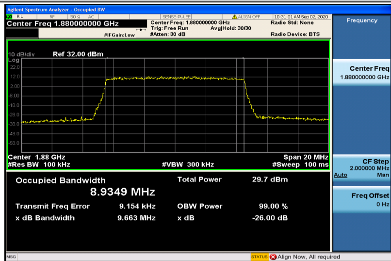
Band2-10MHz-16QAM-18900-50RB#0-8.9349
