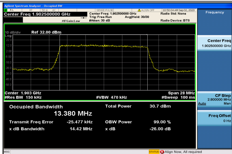
Band2-15MHz-QPSK-19125-75RB#0-13.380
