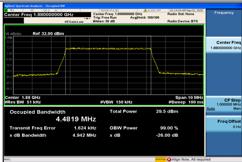
Band2-5MHz-16QAM-18900-25RB#0-4.4819
