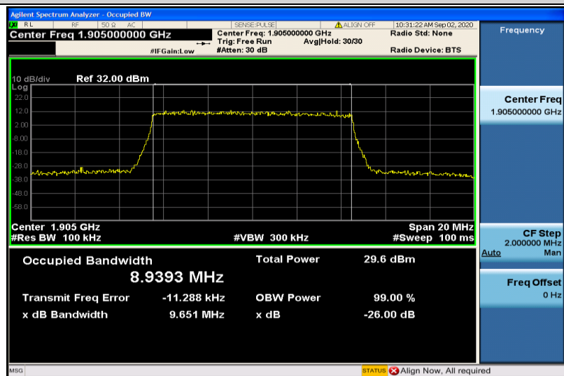
Band2-10MHz-16QAM-19150-50RB#0-8.9393
