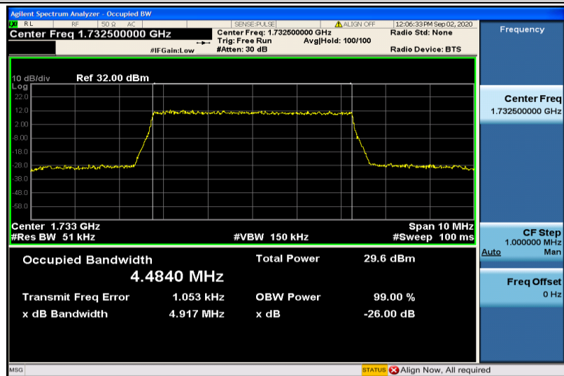
Band4-5MHz-16QAM-20175-25RB#0-4.4840
