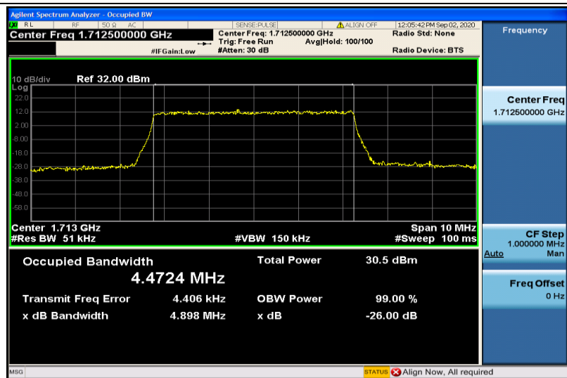
Band4-5MHz-QPSK-19975-25RB#0-4.4724
