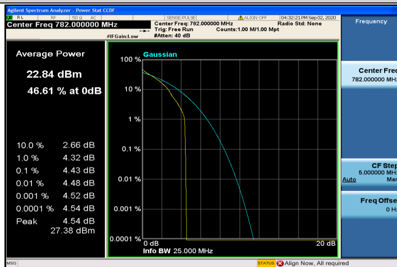
Band13-5MHz-QPSK-23230-1RB#0
