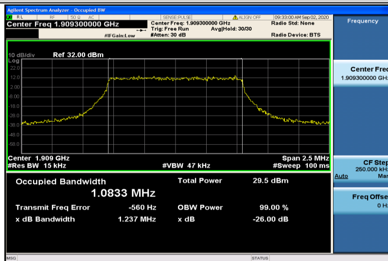
Band2-1.4MHz-QPSK-19193-6RB#0-1.0833
