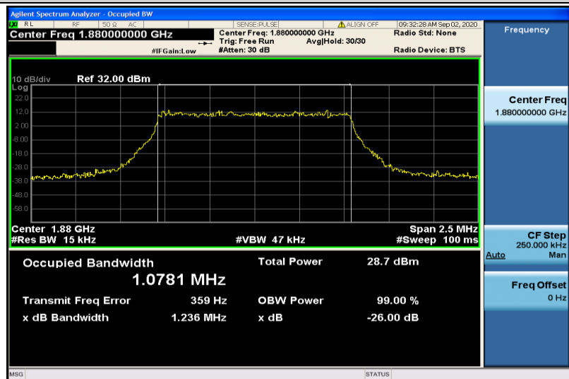
Band2-1.4MHz-16QAM-18900-6RB#0-1.0781
