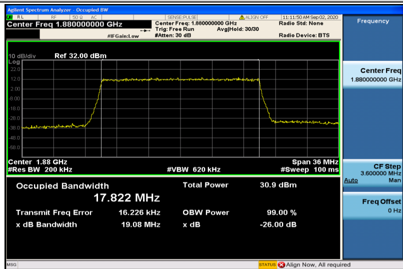
Band2-20MHz-QPSK-18900-100RB#0-17.822
