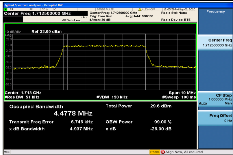
Band4-5MHz-16QAM-19975-25RB#0-4.4778
