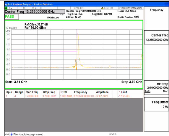
5A_n77(3700-3980MHz) 90M DFT-s-OFDM QPSK Edge_1RB_Left Low
