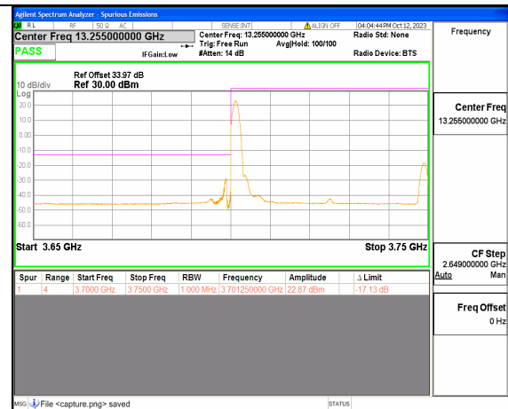
5A_n77(3700-3980MHz) 50M DFT-s-OFDM BPSK Edge_1RB_Left Low
