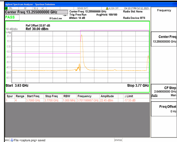
5A_n77(3700-3980MHz) 70M DFT-s-OFDM BPSK Edge_1RB_Left Low
