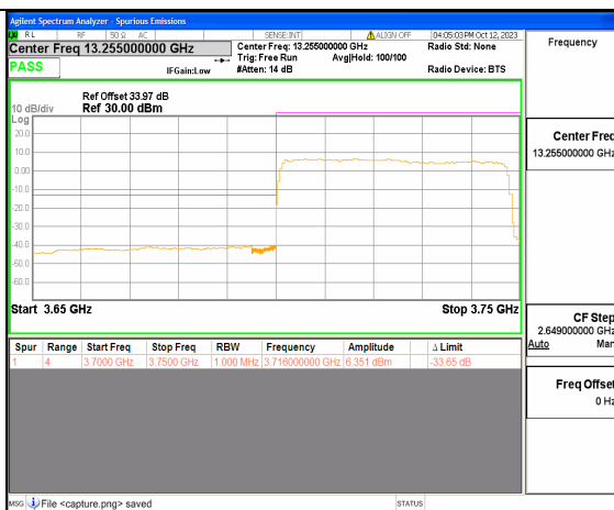
5A_n77(3700-3980MHz) 50M DFT-s-OFDM QPSK Outer_Full Low
