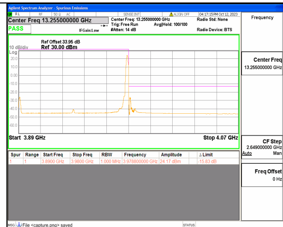
5A_n77(3700-3980MHz) 90M DFT-s-OFDM BPSK Edge_1RB_Right High
