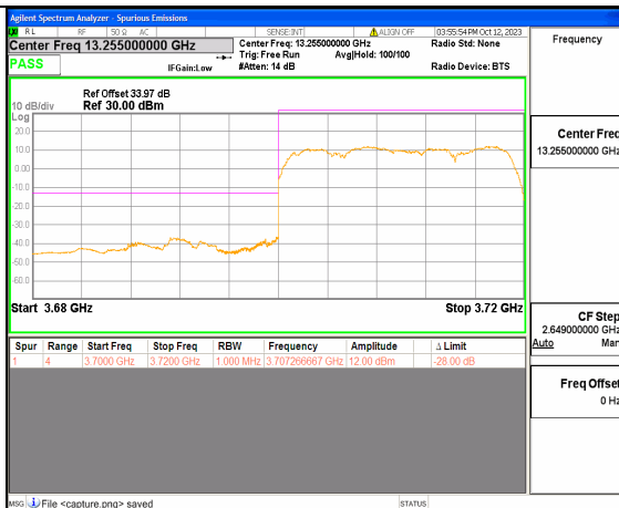
5A_n77(3700-3980MHz) 20M DFT-s-OFDM BPSK Outer_Full Low
