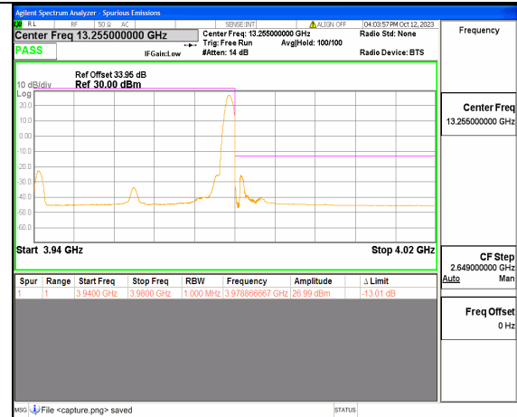
5A_n77(3700-3980MHz) 40M DFT-s-OFDM QPSK Edge_1RB_Right High
