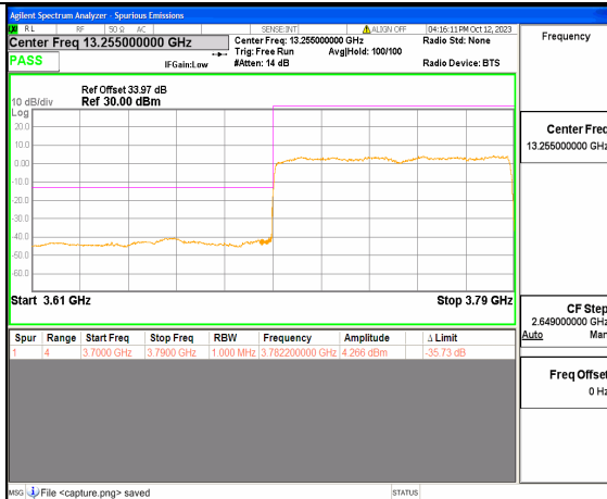
5A_n77(3700-3980MHz) 90M DFT-s-OFDM QPSK Outer_Full Low
