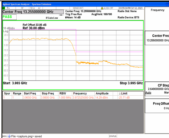
5A_n77(3700-3980MHz) 15M DFT-s-OFDM QPSK Outer_Full High
