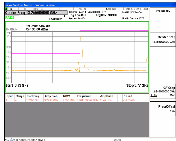
5A_n77(3700-3980MHz) 70M DFT-s-OFDM QPSK Edge_1RB_Left Low
