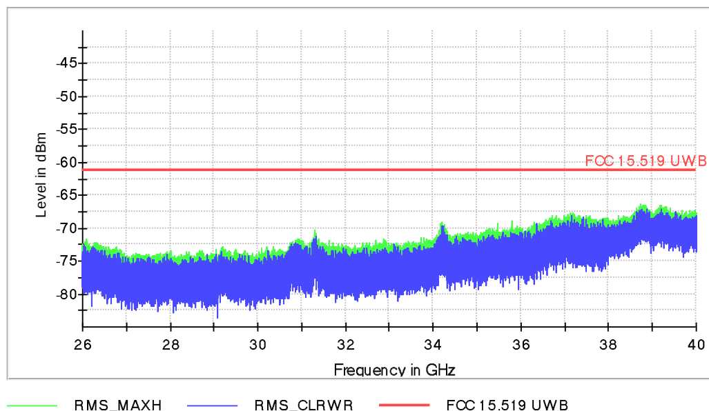
FCC 15.519_26GHz-40GHz
