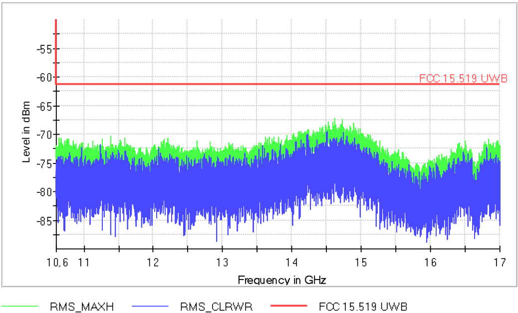
FCC 15.519_10.6-17GHz RBW 100kHz
