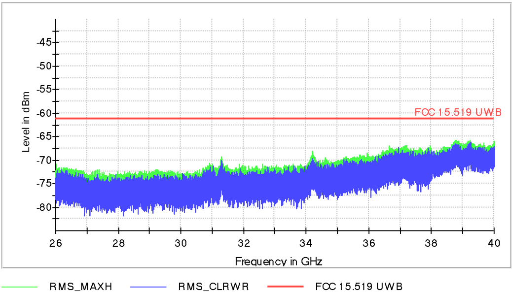
FCC 15.519_26GHz-40GHz
