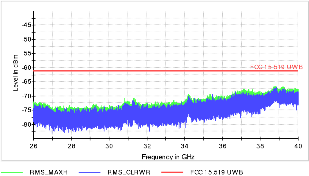
FCC 15.519_26GHz-40GHz
