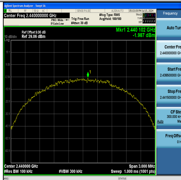
SRD-Ant1-2440-0~Reference-PASS
