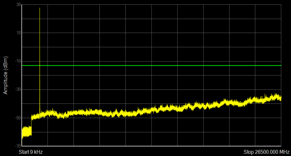
Band2 QPSK BW=5MHz Channel=18625 RB Size=1 Position=#0
