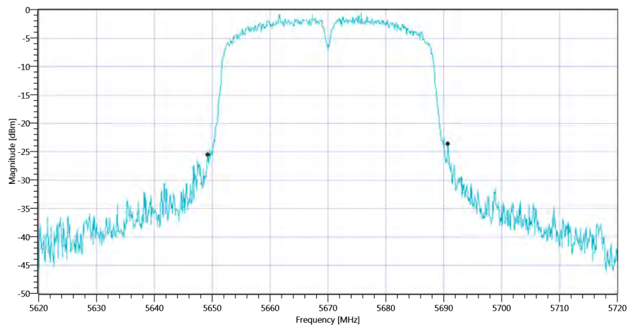
Plot_FCC Part 15.407 & ISSED Bandwidths ~ WLAN5Gx n-HT40 mode U-NII-2C 26dB_06112020_110504.png
