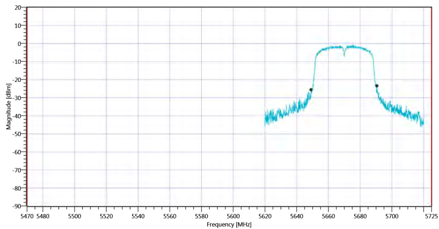
Plot_FCC Part 15.407 & ISSED Bandwidths ~ WLAN5Gx n-HT40 mode U-NII-2C_06112020_110508.png
