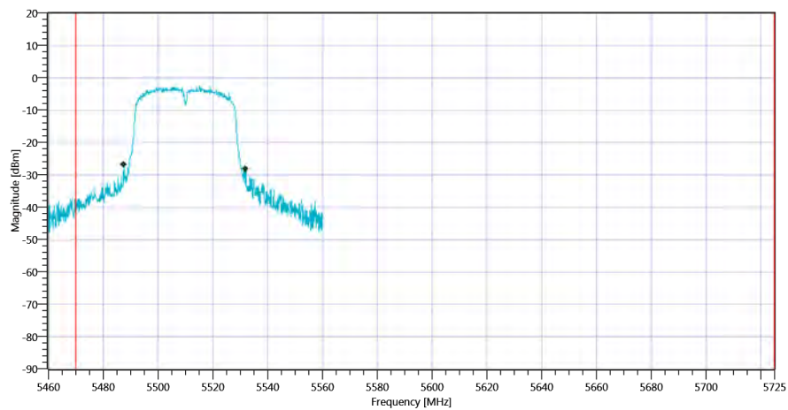
Plot_FCC Part 15.407 & ISSED Bandwidths ~ WLAN5Gx n-HT40 mode U-NII-2C_06112020_105753.png
