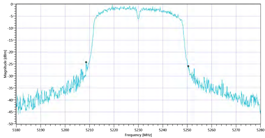
Plot_FCC Part 15.407 & ISSED Bandwidths ~ WLAN5Gx n-HT40 mode U-NII-1 26dB_06112020_104557.png
