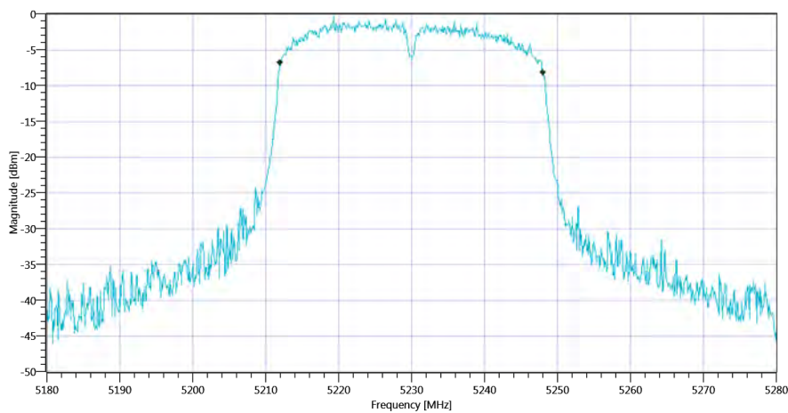
Plot_FCC Part 15.407 & ISCED Bandwidths ~ WLAN5Gx n-HT40 mode U-NII-1 99PCT_06112020_104549.png
