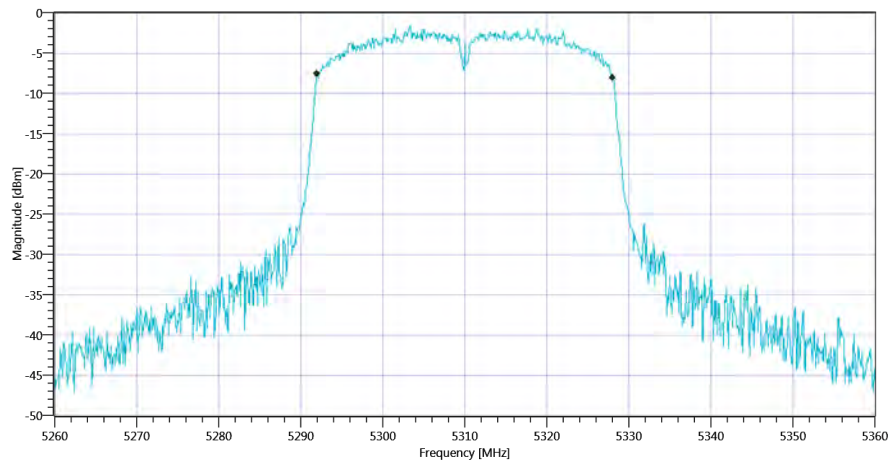
Plot_FCC Part 15.407 & ISSED Bandwidths ~ WLAN5Gx n-HT40 mode U-NII-2A 99PCT_06112020_105319.png
