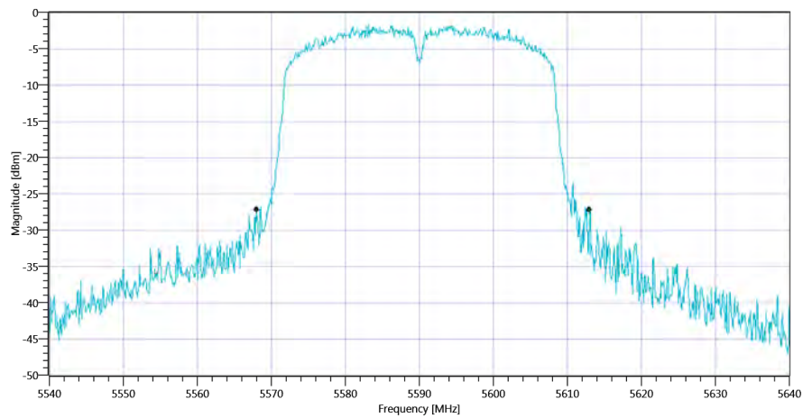
Plot_FCC Part 15.407 & ISSED Bandwidths ~ WLAN5Gx n-HT40 mode U-NII-2C 26dB_06112020_110126.png
