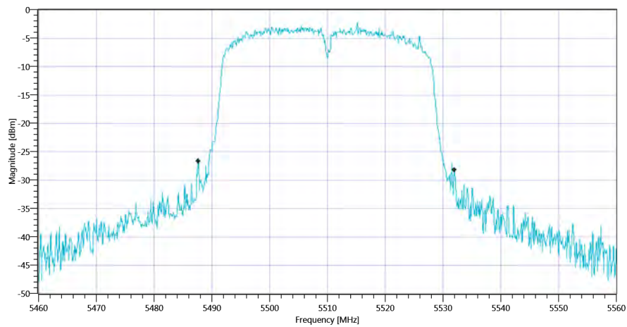
Plot_FCC Part 15.407 & ISSED Bandwidths ~ WLAN5Gx n-HT40 mode U-NII-2C 26dB_06112020_105750.png
