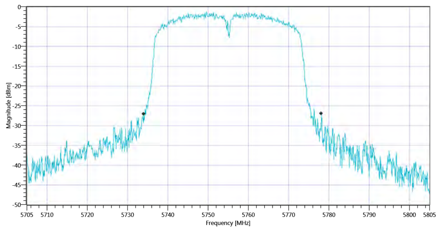
Plot_FCC Part 15.407 & ISSED Bandwidths ~ WLAN5Gx n-HT40 mode U-NII-3 26dB_06112020_110928.png
