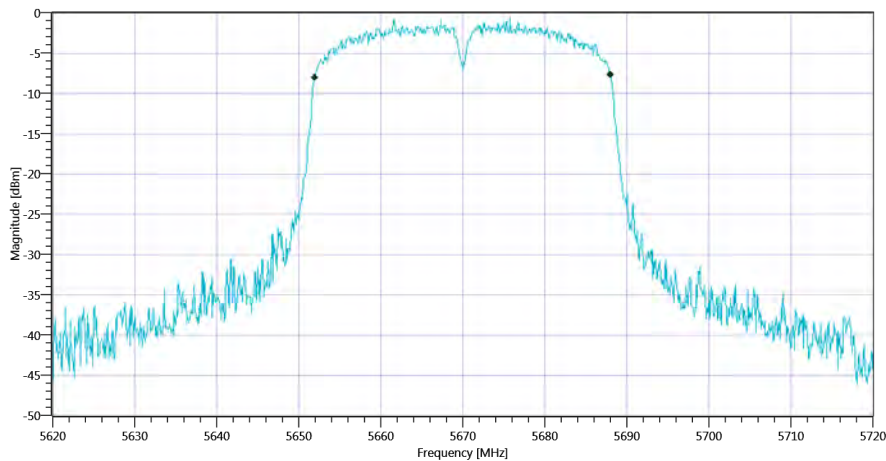
Plot_FCC Part 15.407 & ISSED Bandwidths ~ WLAN5Gx n-HT40 mode U-NII-2C 99PCT_06112020_110455.png
