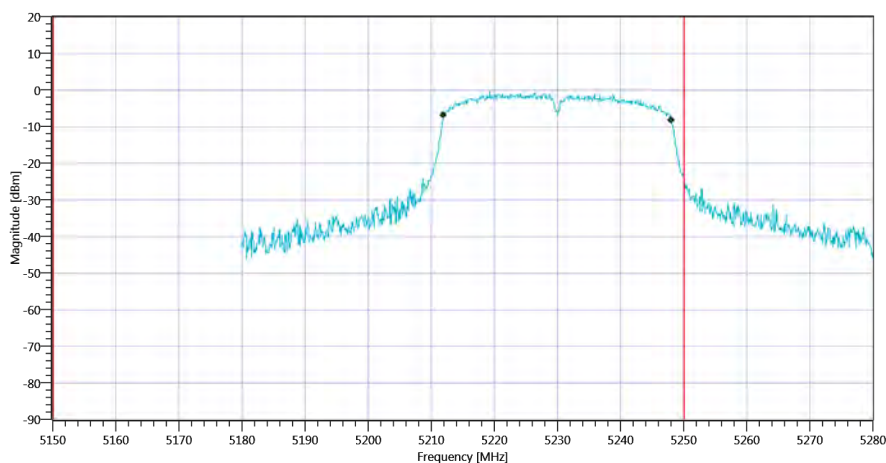
Plot_FCC Part 15.407 & ISCED Bandwidths ~ WLAN5Gx n-HT40 mode U-NII-1_06112020_104552.png
