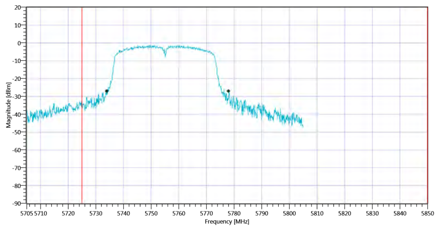
Plot_FCC Part 15.407 & ISSED Bandwidths ~ WLAN5Gx n-HT40 mode U-NII-3_06112020_110932.png
