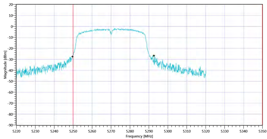
Plot_FCC Part 15.407 & ISSED Bandwidths ~ WLAN5Gx n-HT40 mode U-NII-2A_06112020_104942.png
