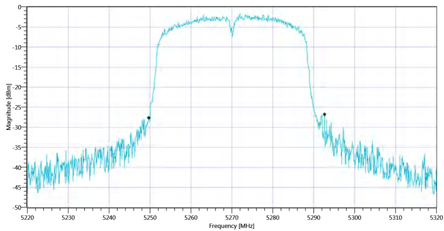
Plot_FCC Part 15.407 & ISSED Bandwidths ~ WLAN5Gx n-HT40 mode U-NII-2A 26dB_06112020_104938.png
