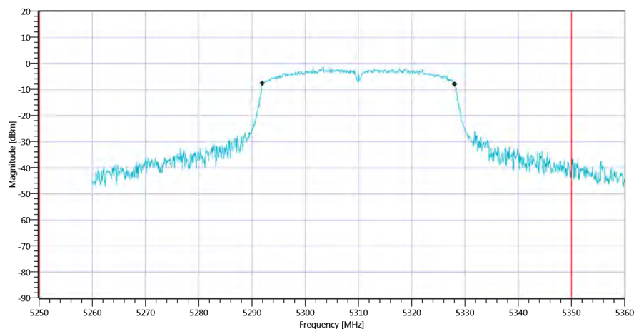
Plot_FCC Part 15.407 & ISSED Bandwidths ~ WLAN5Gx n-HT40 mode U-NII-2A_06112020_105323.png
