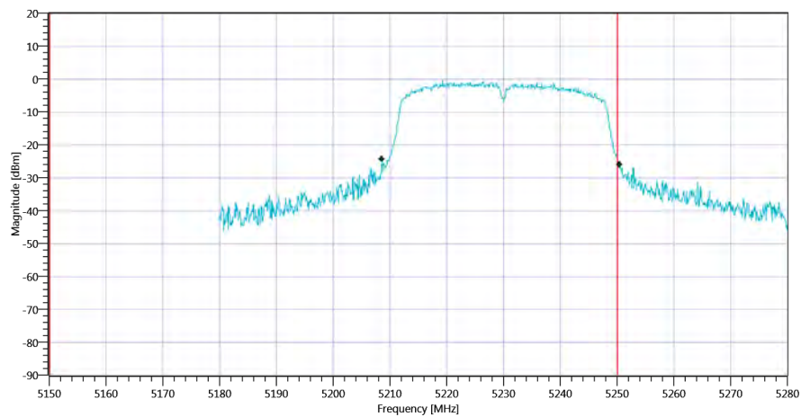
Plot_FCC Part 15.407 & ISSED Bandwidths ~ WLAN5Gx n-HT40 mode U-NII-1_06112020_104601.png
