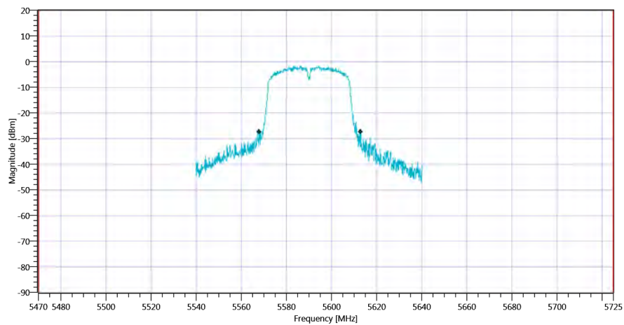
Plot_FCC Part 15.407 & ISSED Bandwidths ~ WLAN5Gx n-HT40 mode U-NII-2C_06112020_110130.png
