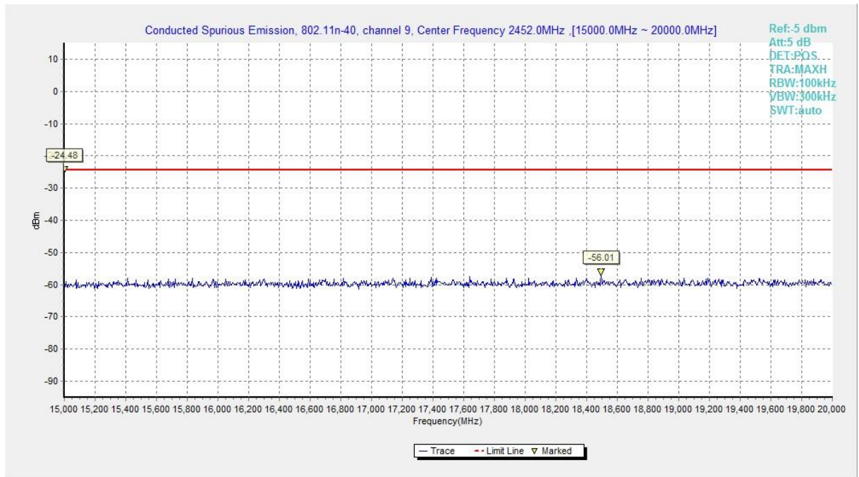
Fig.A.6.1.143 Transmitter Spurious Emission - Conducted (802.11n-HT40, Chain1, Ch9, 15 GHz-20 GHz)
