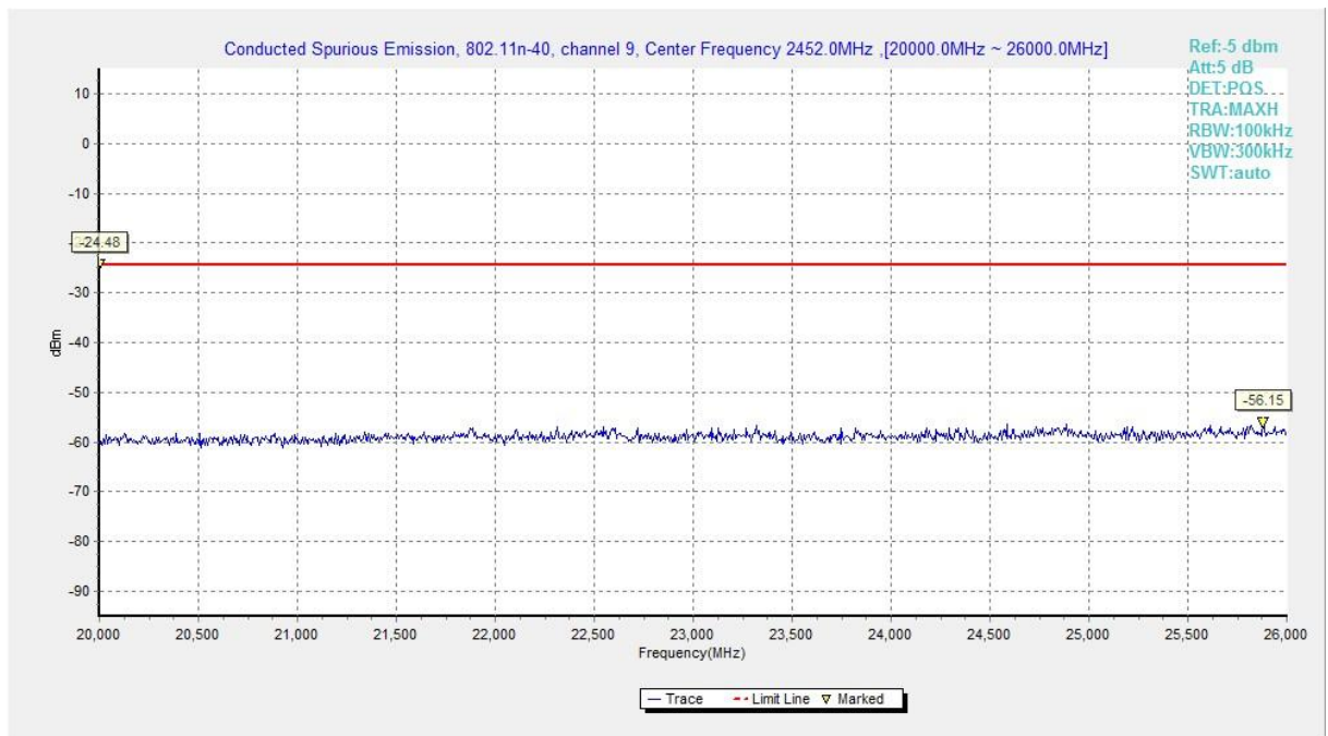
Fig.A.6.1.144 Transmitter Spurious Emission - Conducted (802.11n-HT40, Chain1, Ch9, 20 GHz-26 GHz)
