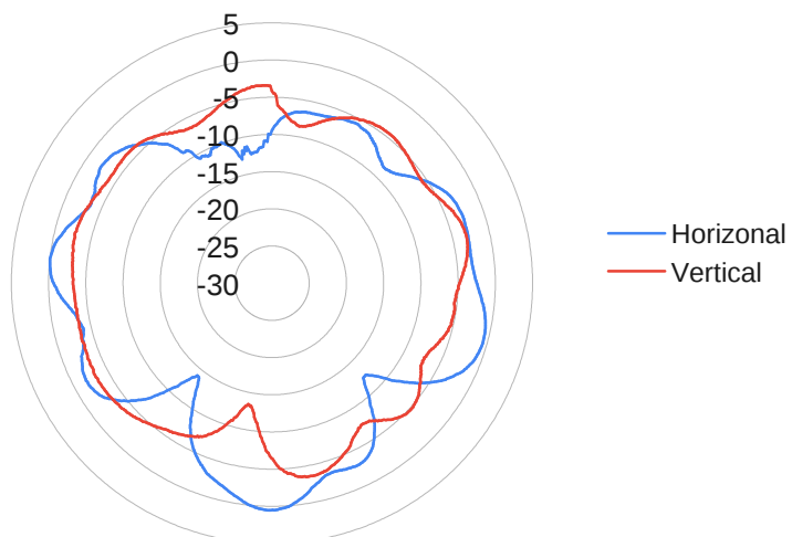
Antenna gain
