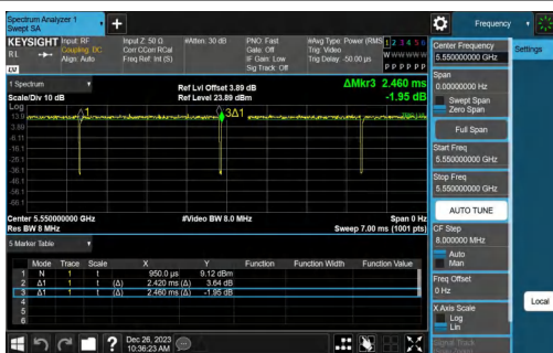
NTNV-11N40SISO-Ant0-5670
