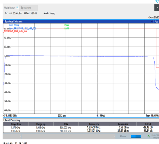
1-N25--15-40-H-6-CP-QPSK-Outer_Full-216@0-Ant1-seegraph-PASS-see graph
