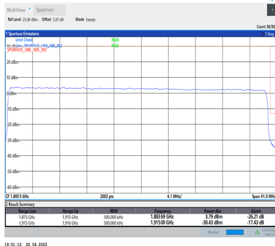
1-N25--15-40-H-3-DFT-PI2BPSK-Outer_Full-216@0-Ant1-seegraph-PASS-see graph
