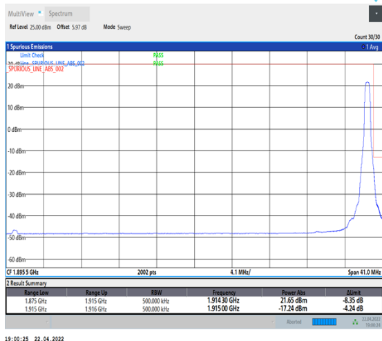
1-N25--15-40-H-2-DFT-PI2BPSK-Edge_1RB_Right-1@215-Ant1-seegraph-PASS-see graph
