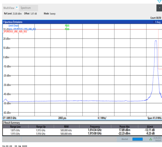
1-N25--15-40-H-5-CP-QPSK-Edge_1RB_Right-1@215-Ant1-seegraph-PASS-see graph
