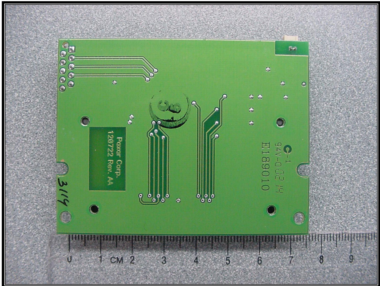
PHOTOGRAPH 22: PCMCIA PCB BACK
