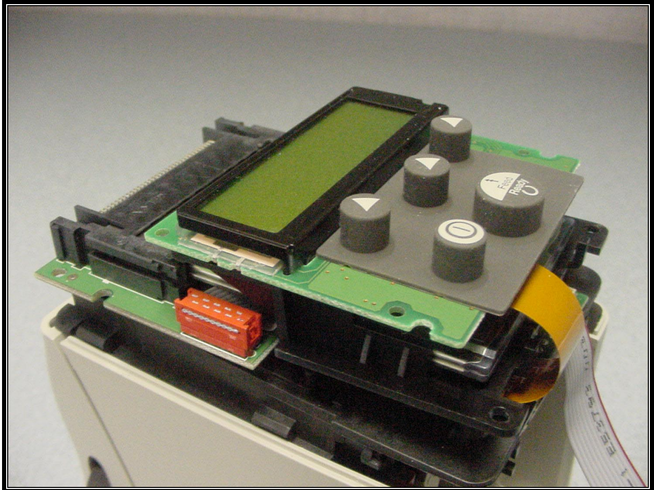
PHOTOGRAPH 18: EUT WITH TOP COVER REMOVED
