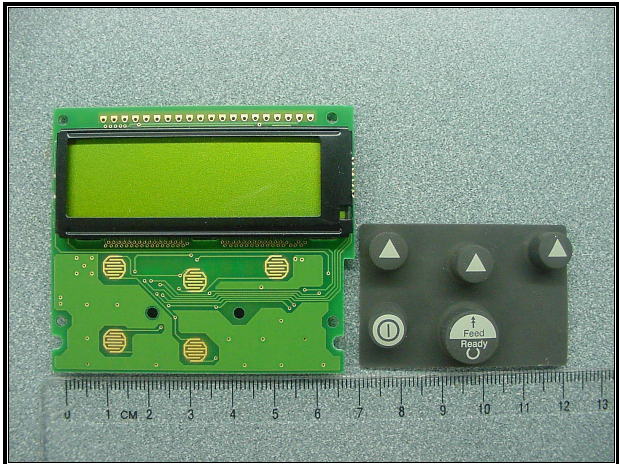
PHOTOGRAPH 19: FRONT OF LCD PCB WITH TOP OF KEYPAD
