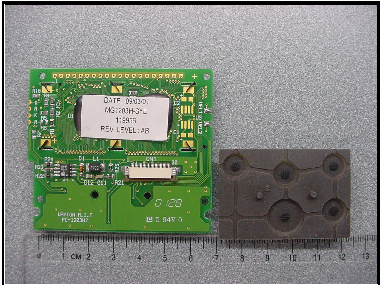
PHOTOGRAPH 20: BACK OF LCD PCB WITH BACK OF KEYPAD
