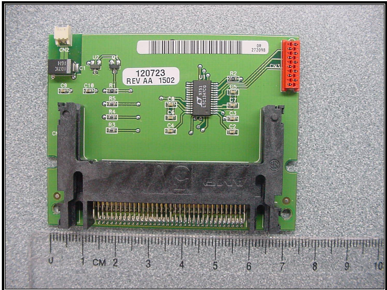
PHOTOGRAPH 21: PCMCIA PCB FRONT
