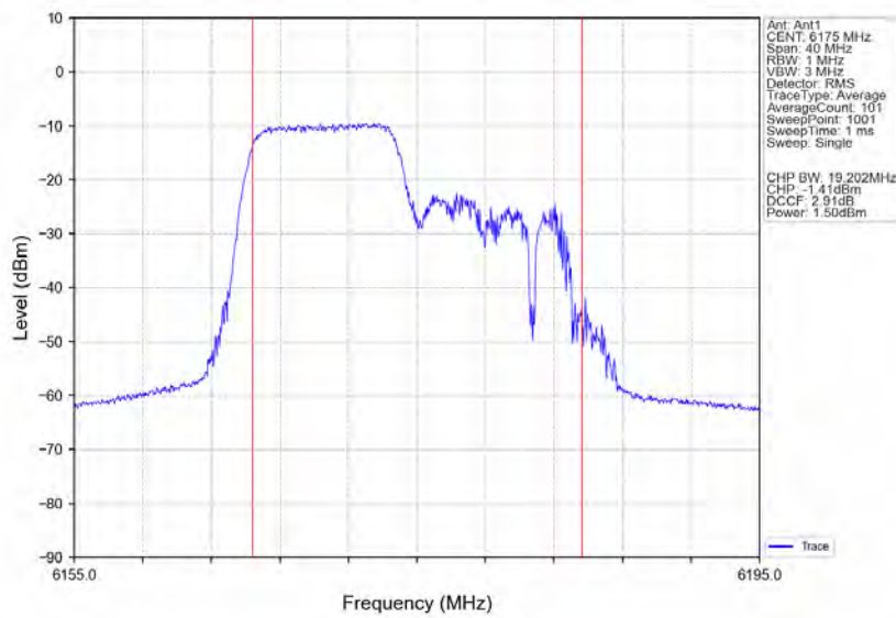
802.11ax(HE20)_MCH_6175MHz_RU106_Right_Ant1_NTNV
