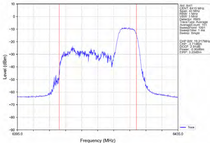
802.11ax(HE20) HCH_6415MHz_RU52_Right_Ant1_NTNV
