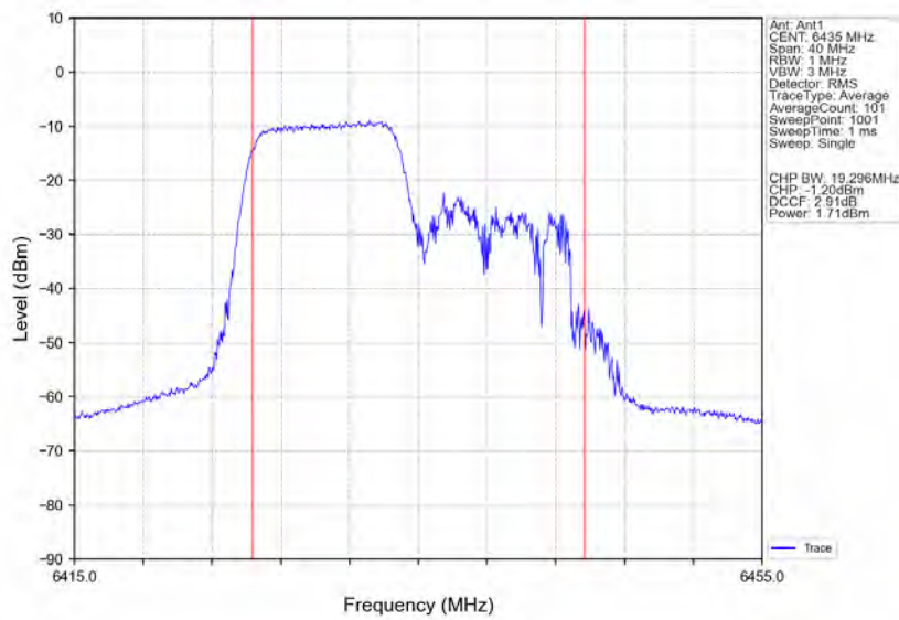
802.11ax(HE20)_LCH_6435MHz_RU106_Right_Ant1_NTNV
