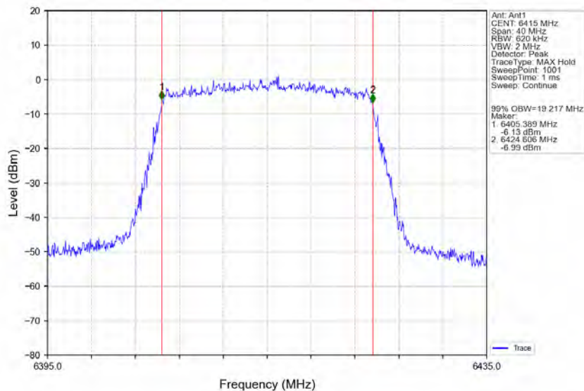
802.11ax(HE20)_HCH_6415MHz_RU242_Ant1_NTNV
