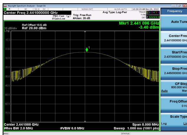
Output Power: GFSK,2441MHz,DH5
