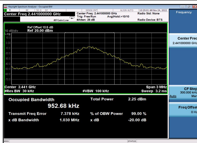
20dB Bandwidth: GFSK,2441MHz,DH5
