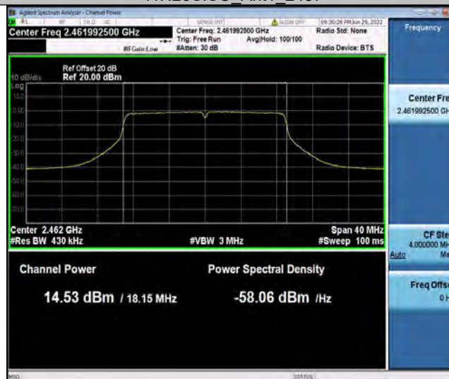
11N20SISO Ant1 2462
