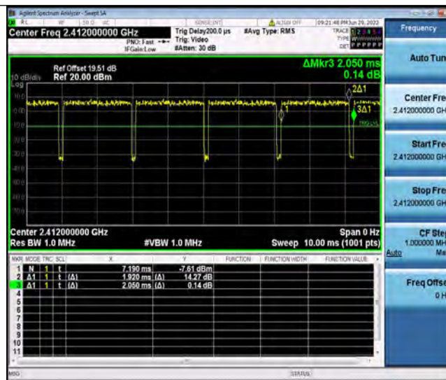
11N20SISO Ant1 2412
