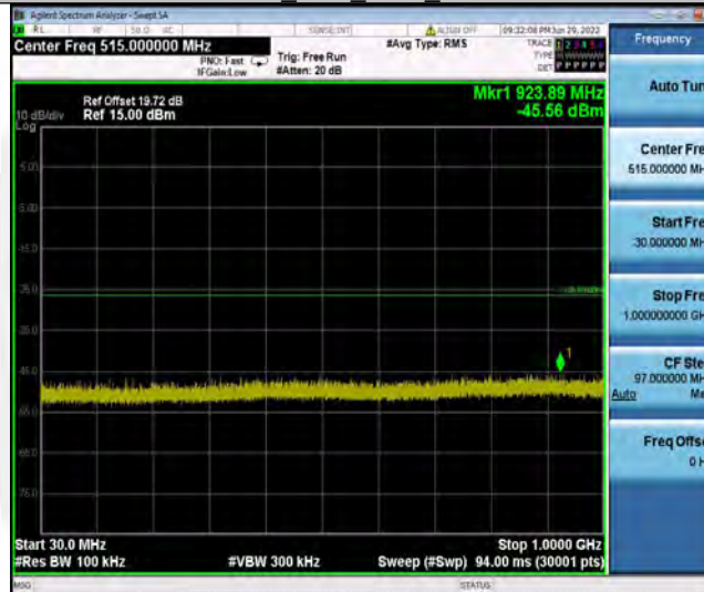
11N20SISO_Ant1_2462_30~1000
