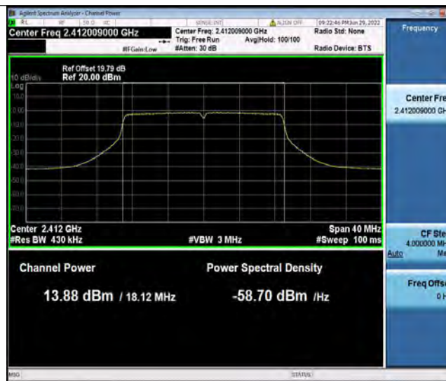
11N20SISO Ant1 2412
